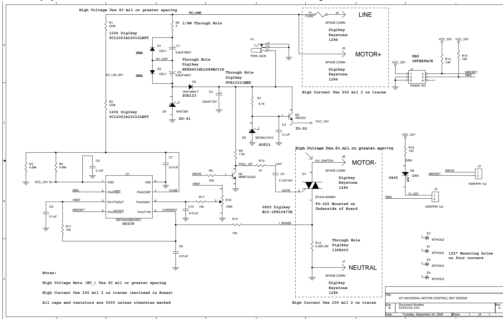
Figure 5. Z8 Encore! XP Universal Motor Control Reference Design
