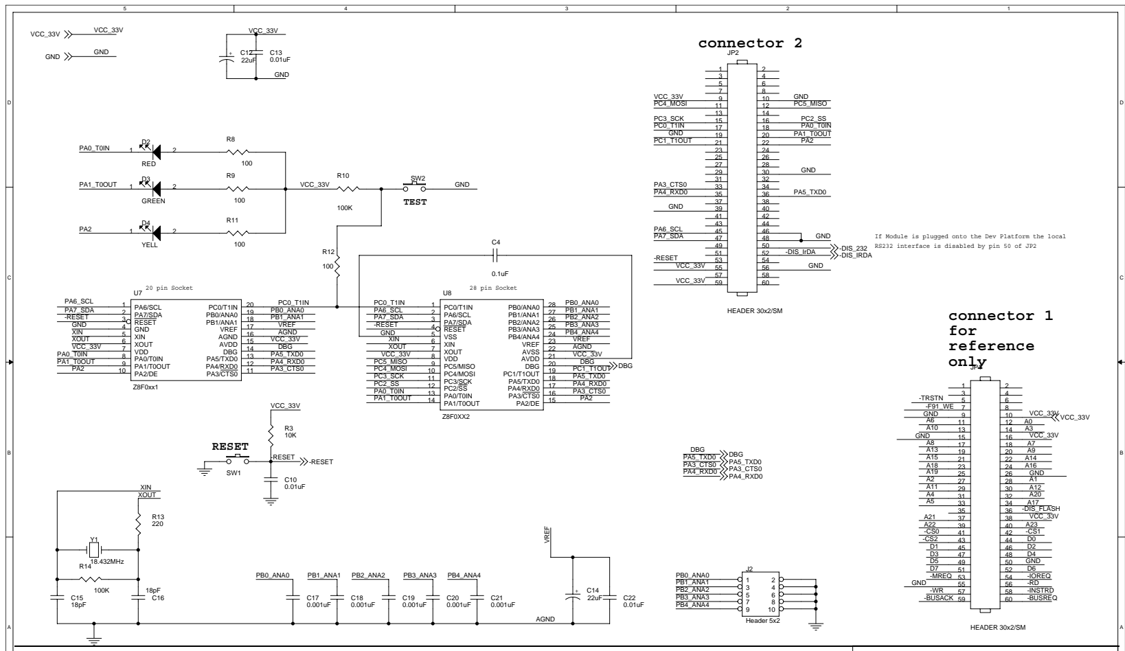
Figure 3 and Figure 4 displays the schematics for Z8 Encore! XP® F0822 Series Evaluation Board.
