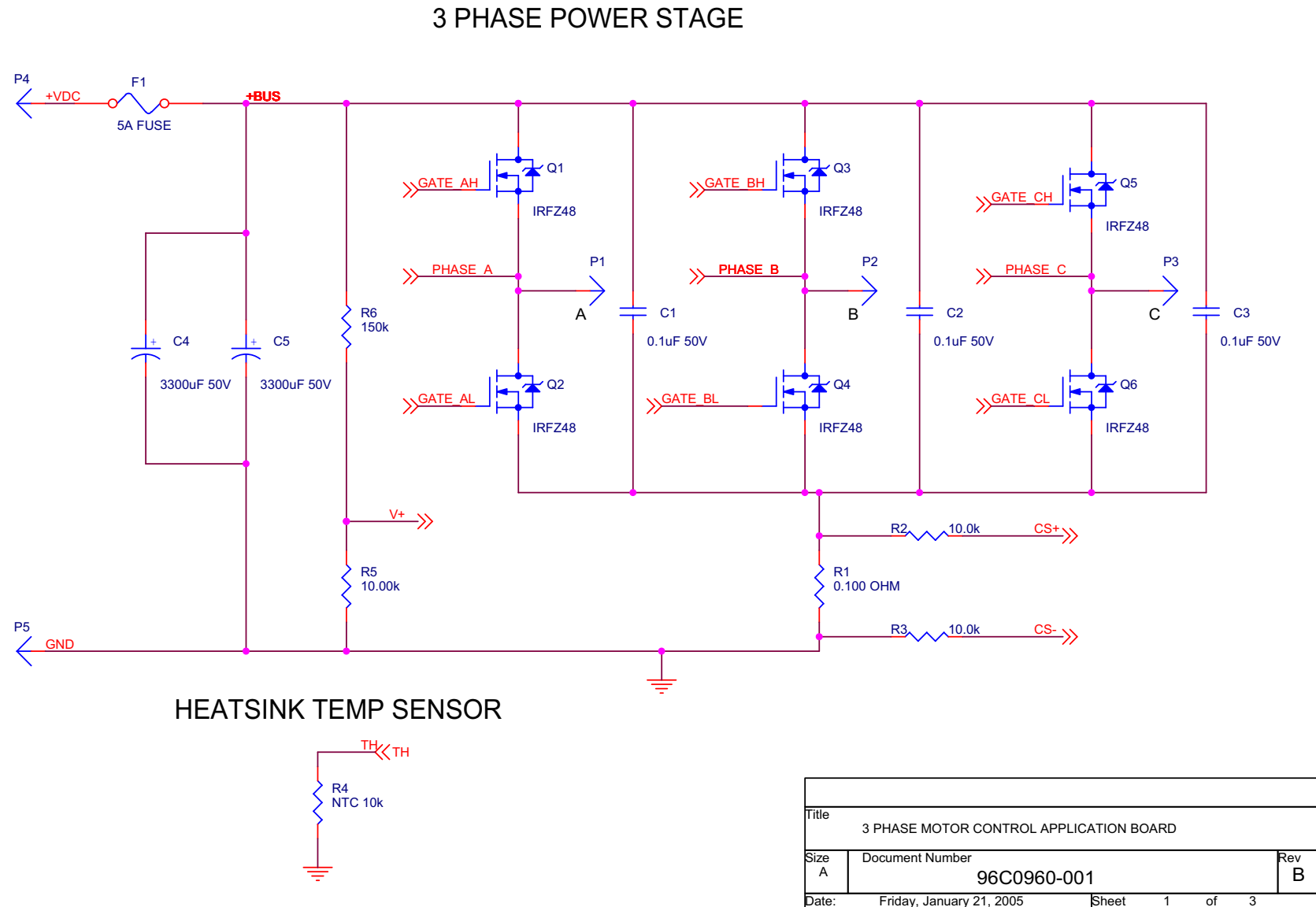
Figure 7. 3-Phase Motor Control Application Board Schematic, #1 of 3
