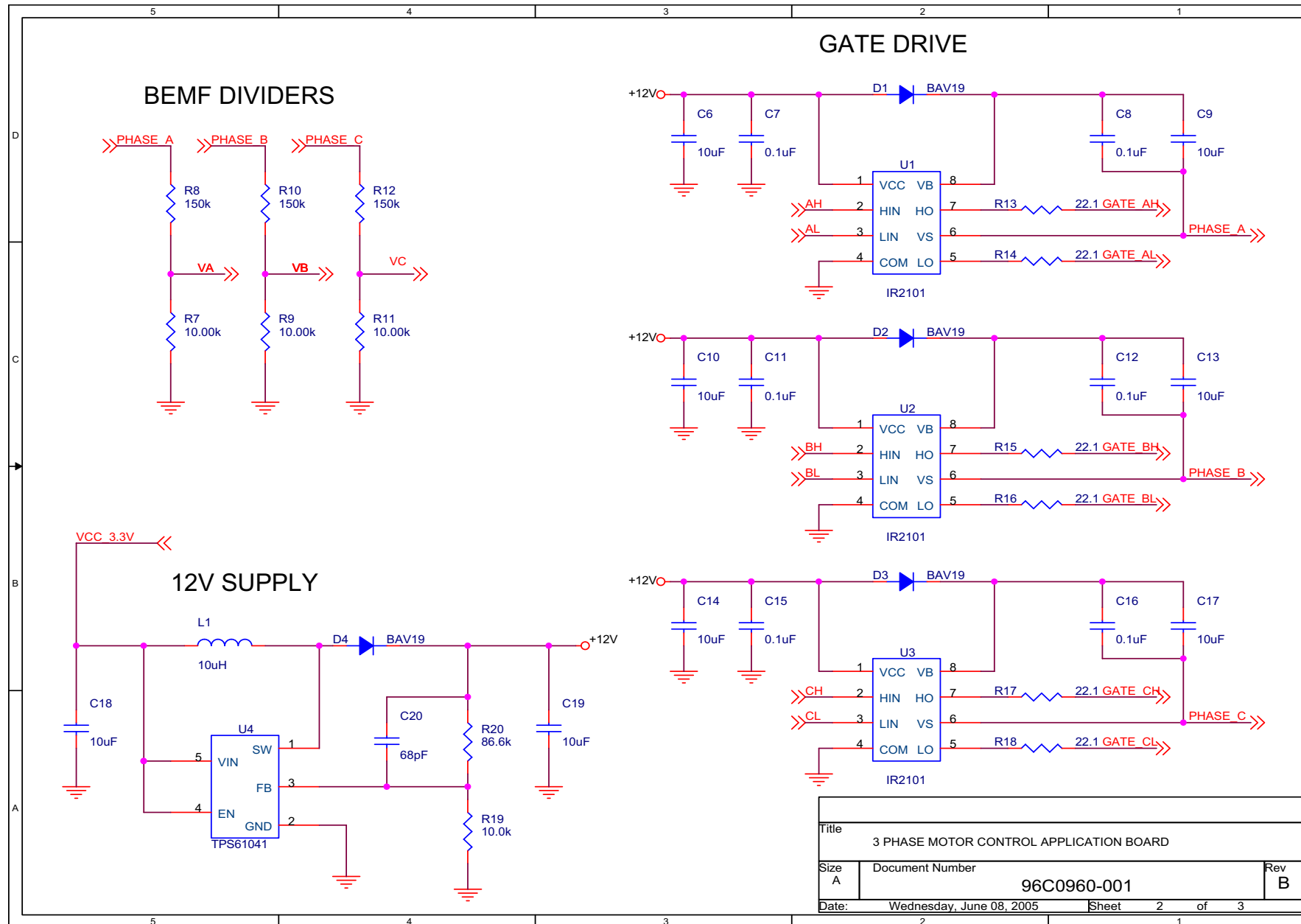
Figure 8. 3-Phase Motor Control Application Board Schematic, #2 of 3
