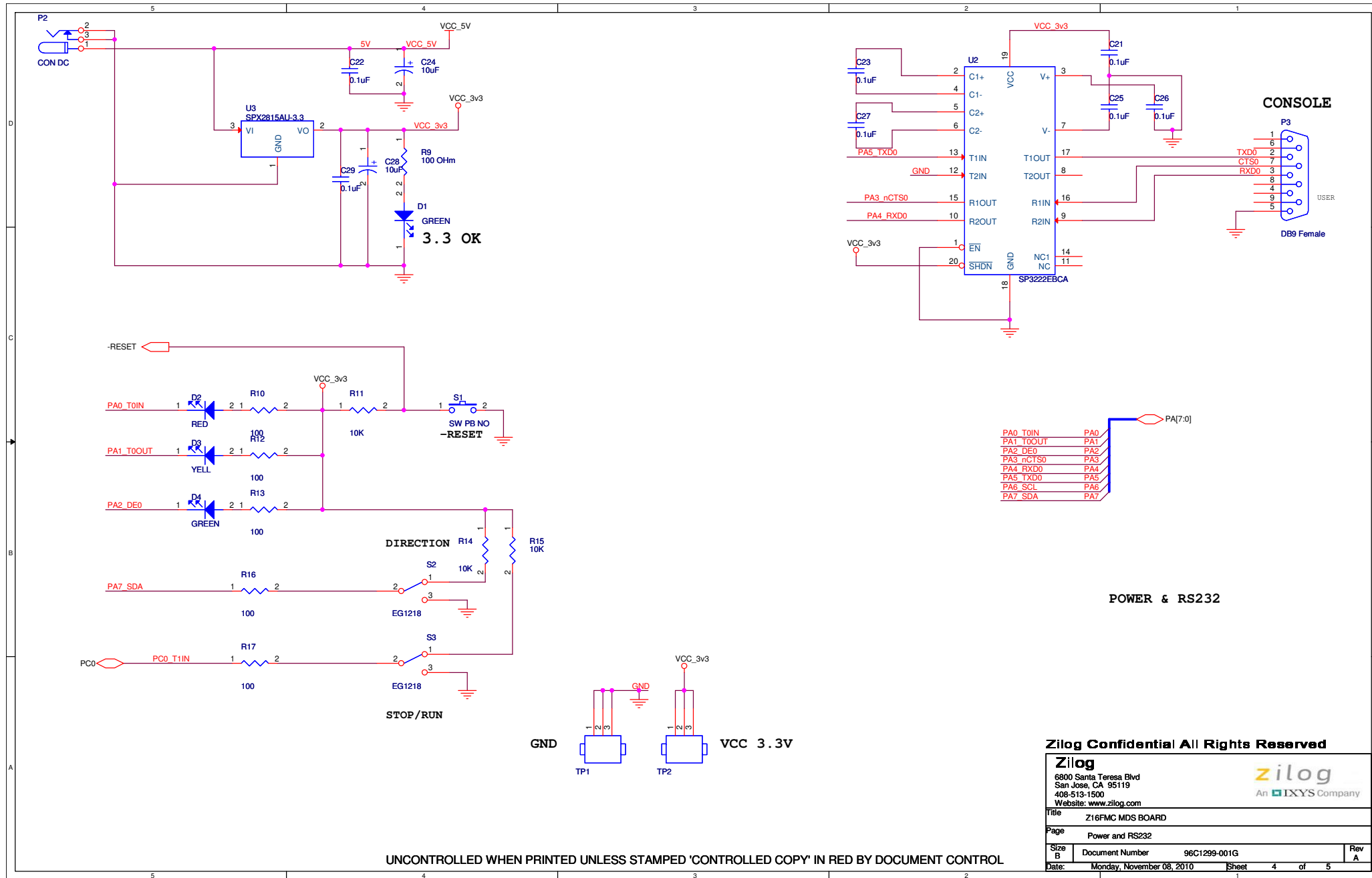
Figure 9. Z16FMC MDS Board Schematic, #2 of 3
