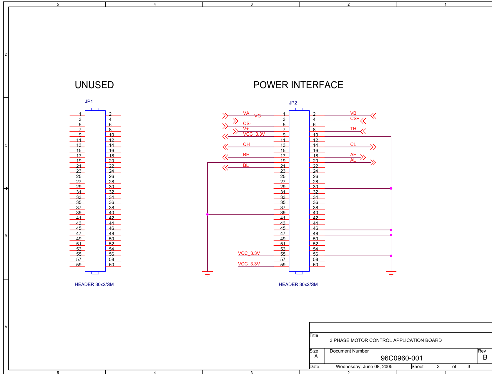
Figure 9. 3-Phase Motor Control Application Board Schematic, #3 of 3
