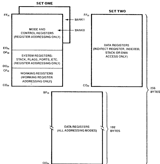
Figure 6. Super8 Registers
