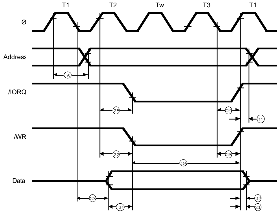
Z180 I/O Write Cycle Timing
