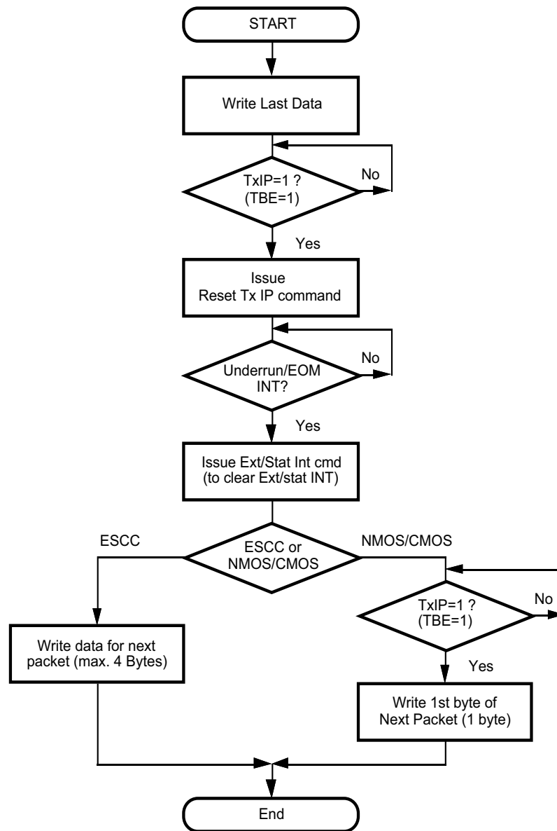
Flowchart example of processing an end of packet
