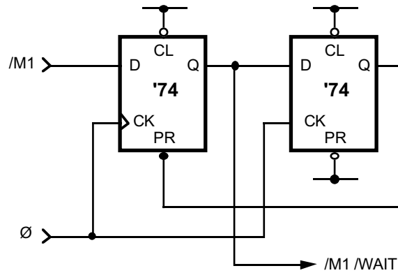
Wait State Generator Logic
