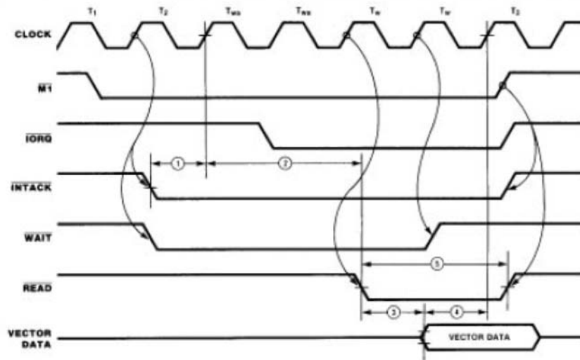
Figure 10. Z80A/Z80B CPU to Z8500/Z8500A Peripheral Interrupt Acknowledge Interface Timing
