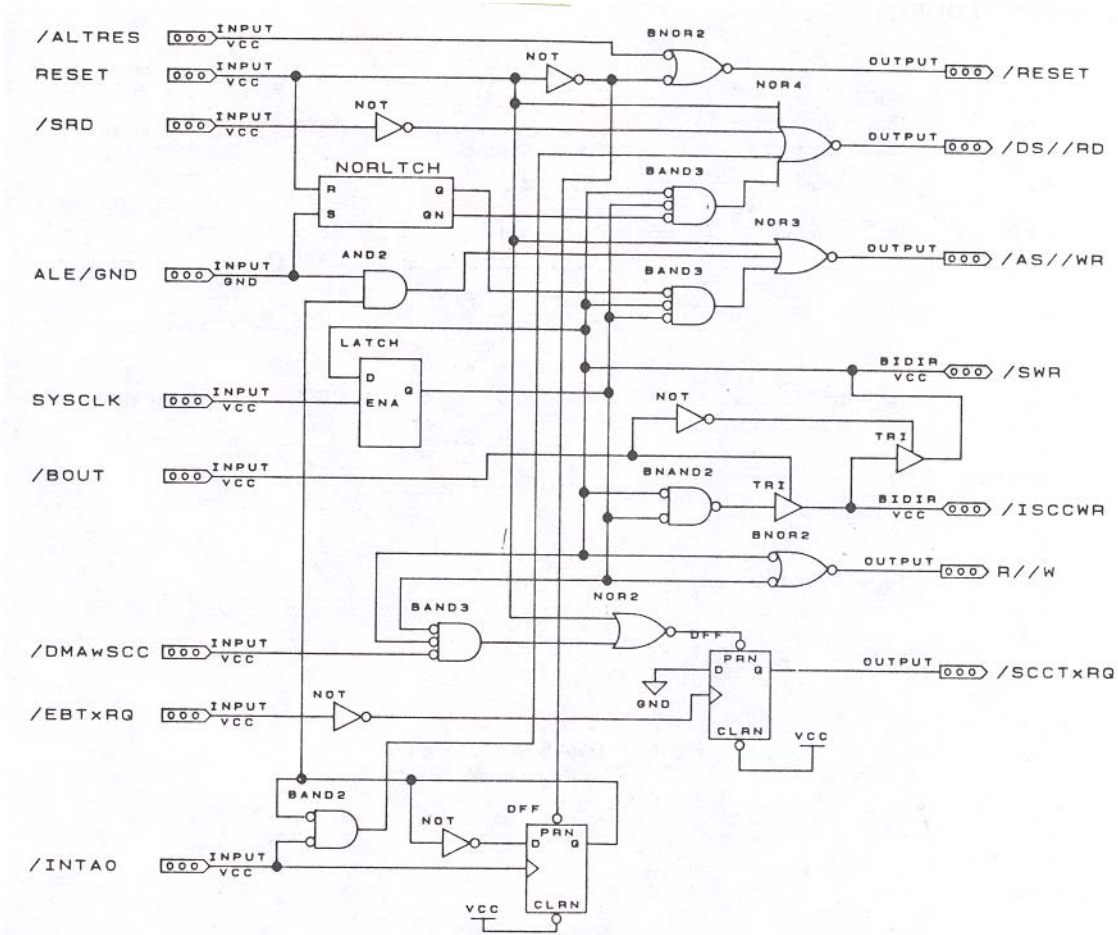
SCC EPLD for 186 Board
