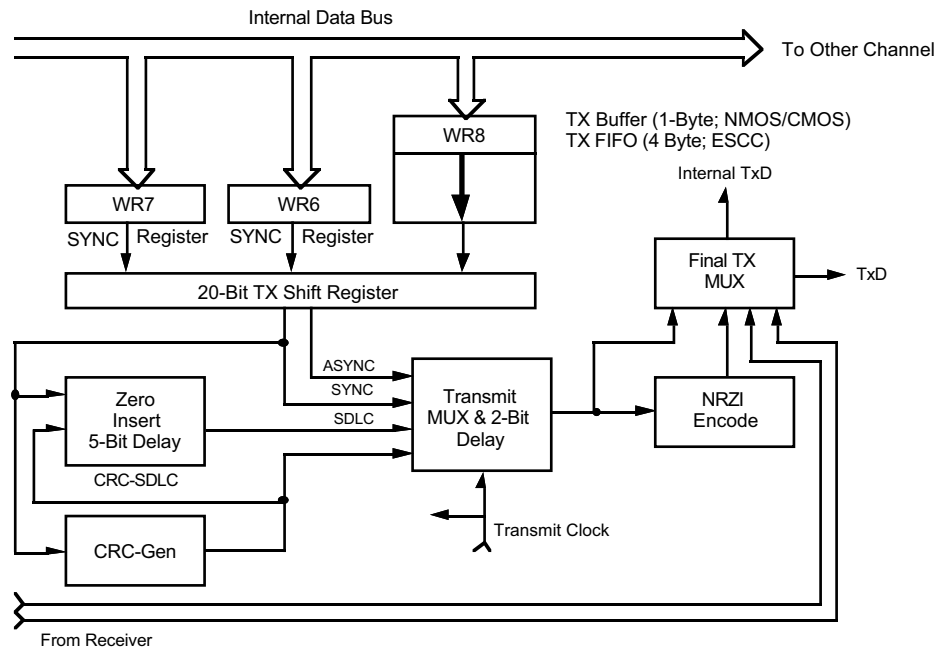
Transmit Data Path
