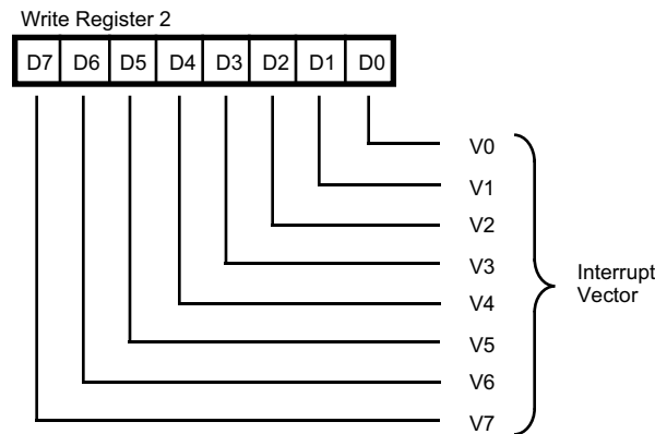
Write Register 2
