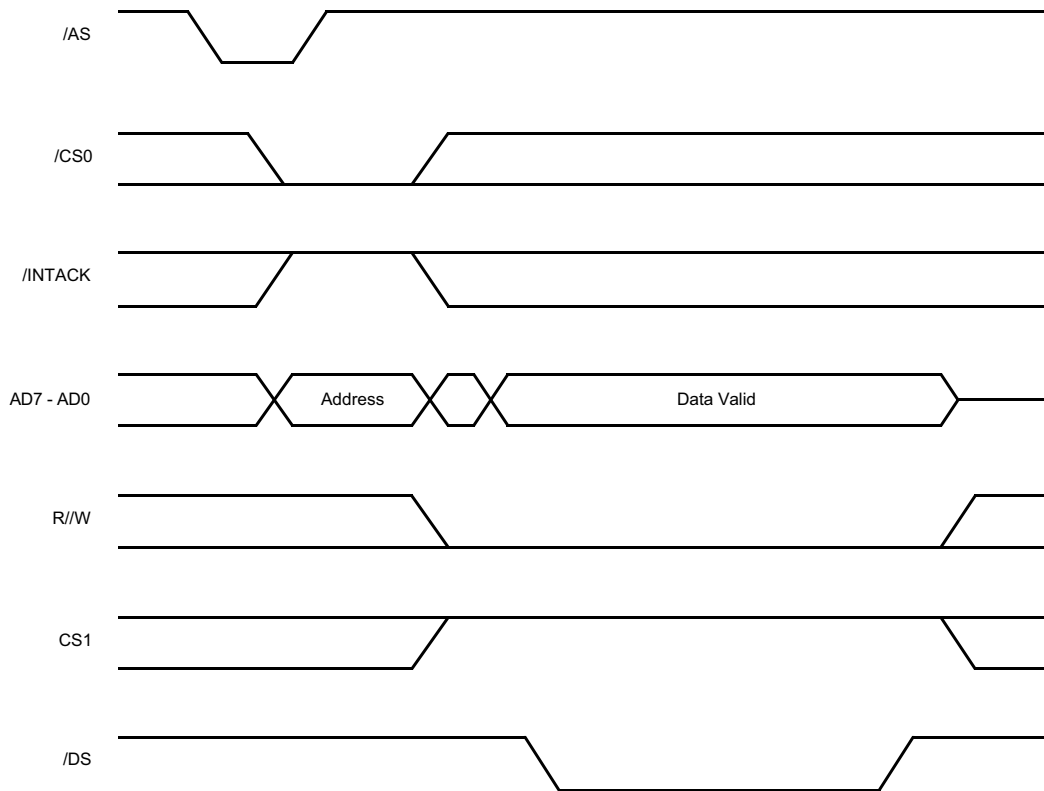
Z80X30 Write Cycle
