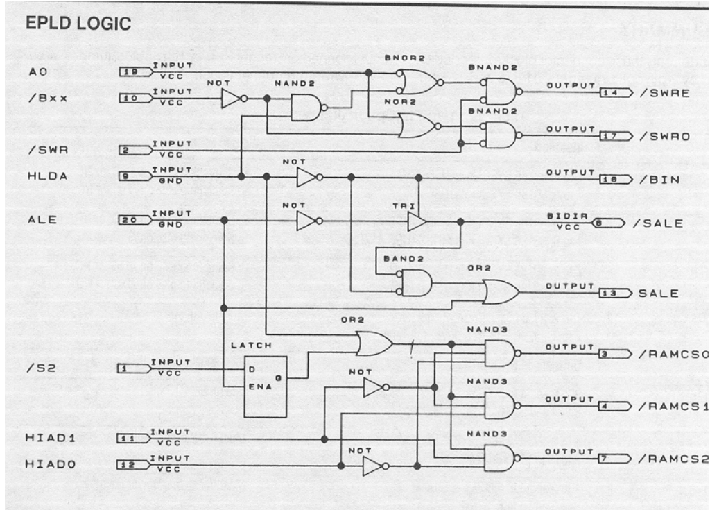
Control EPLD for 186 Board
