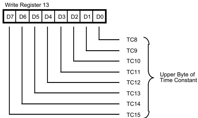
Write Register 13
