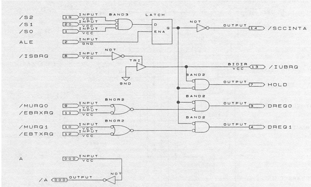
DMA EPLD for 186 Board
