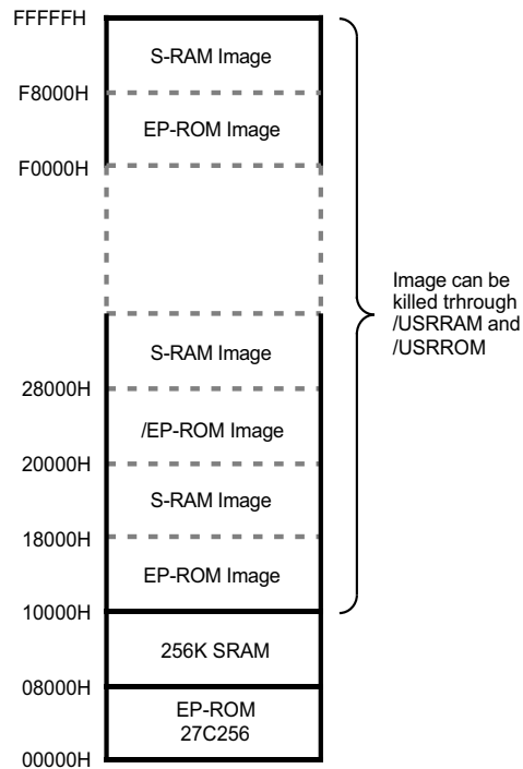
Physical Memory Address Map
