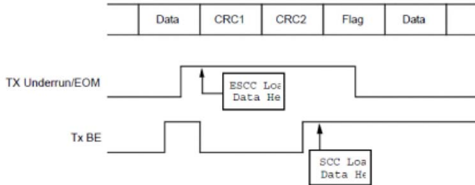
Figure 14. Operation of Shared Flag Transmission
