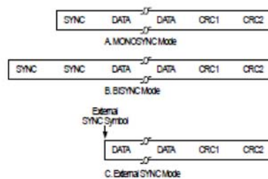
Figure 1. Synchronous Modes of Communication
