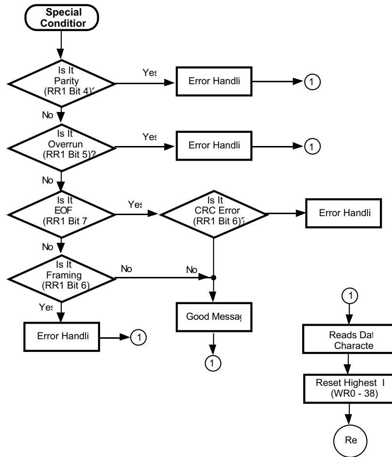
Special Conditions Interrupt Service Flow
