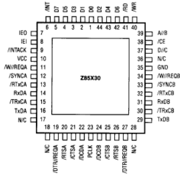
Z85X30 PLCC Pin Assignments
