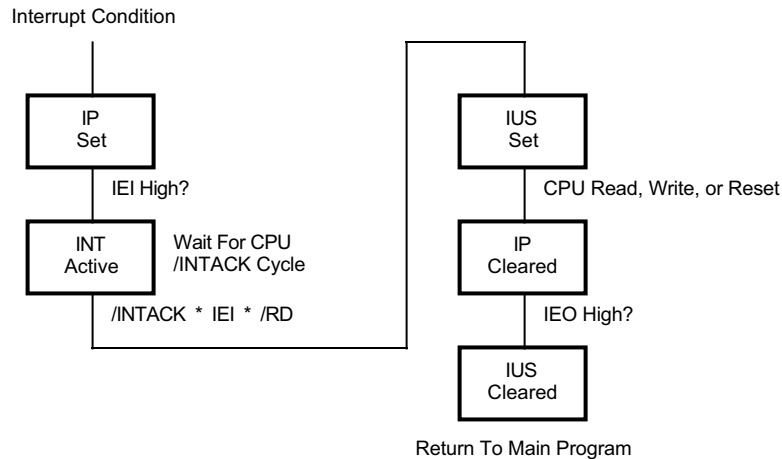
SCC Interrupt Status Diagram
