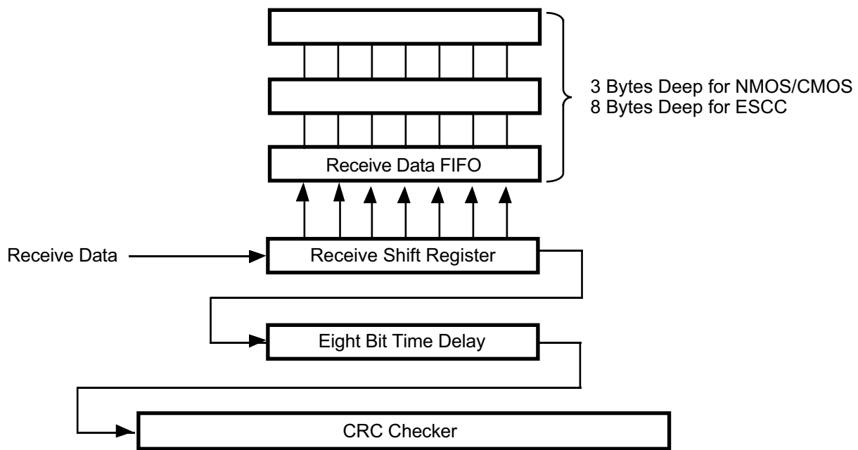
Receive CRC Data Path
