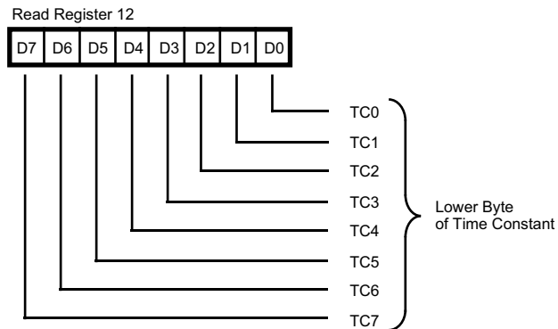
Read Register 12
