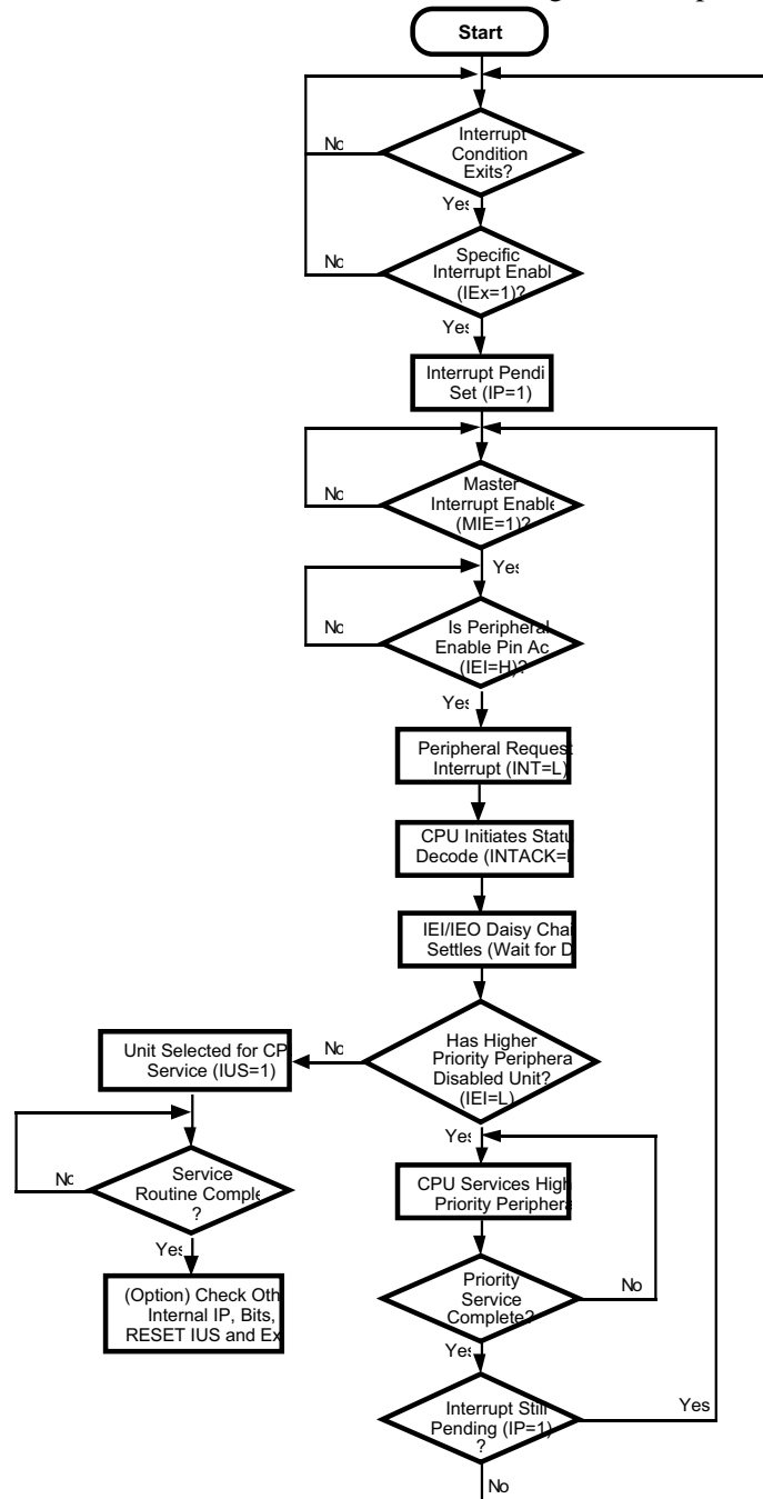
Interrupt Flow Chart (for each interrupt source)
