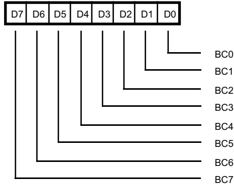
Read Register 6 *
