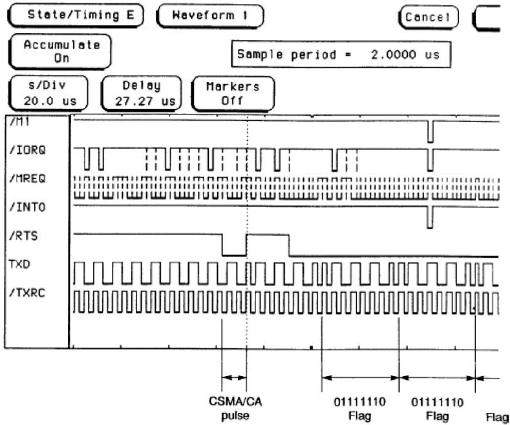
CSMA/CA before an LLAP frame
