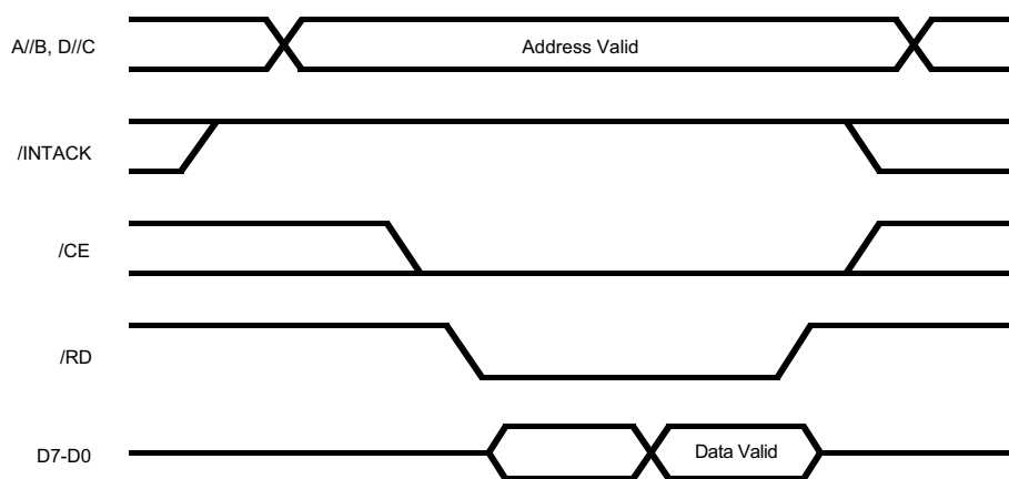
Z85X30 Read Cycle Timing
