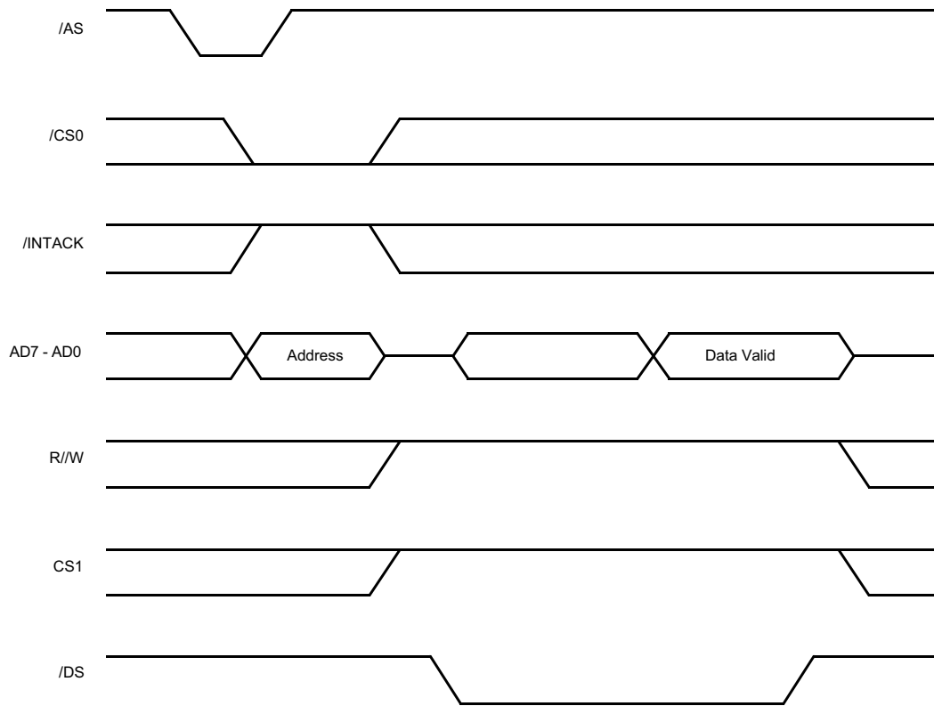
Z80X30 Read Cycle
