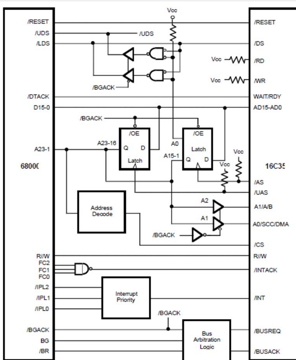
Figure 3. ISCC Interface to a 68000 Microprocessor
