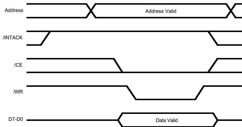
SCC Write Cycle Timing
