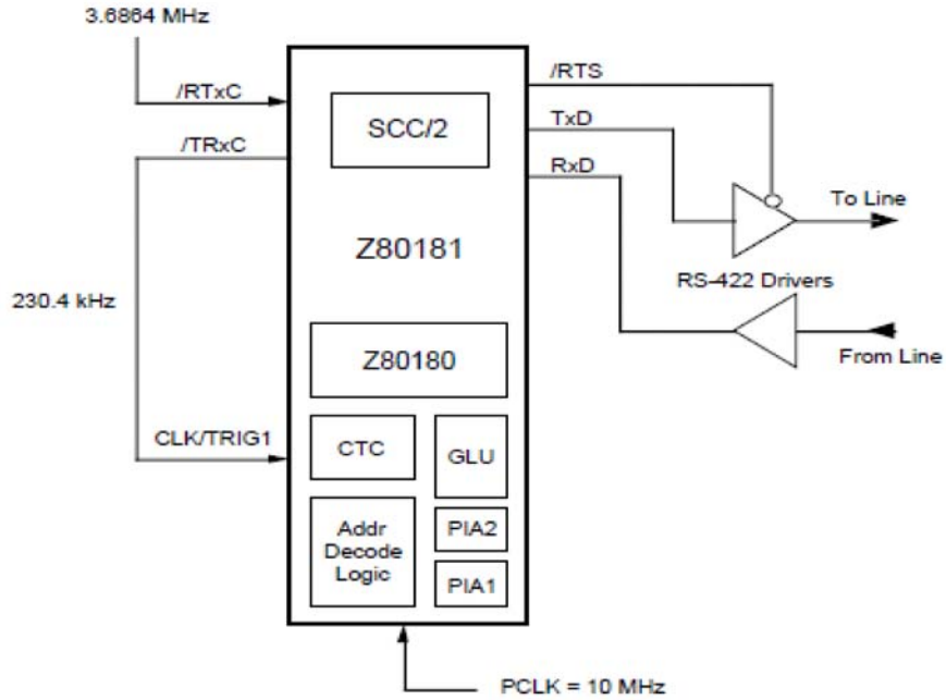
Figure 2. Driver Hardware Configuration
