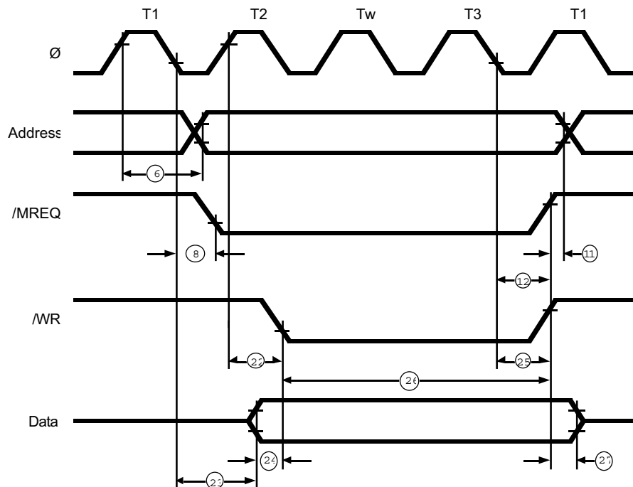
Z180 Memory Write Cycle Timing (One Wait State)
