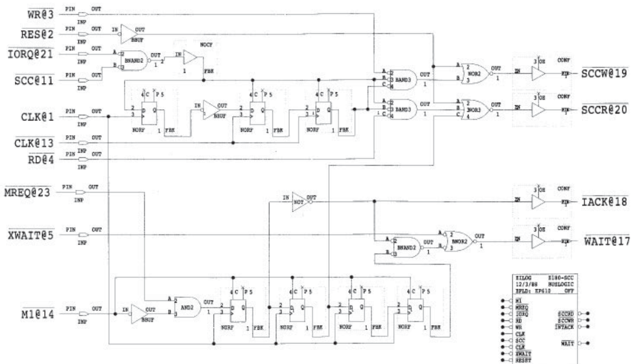
ELPD Circuit Implementation
