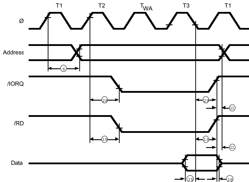
Z180 I/O Read Cycle Timing (/IOC = 0)
