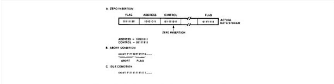
Figure 2. Bit Patterns for Various Line Conditions
