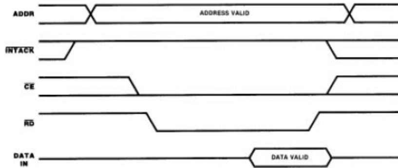
Figure 1. Z8500 Peripheral I/O Read Cycle Timing
