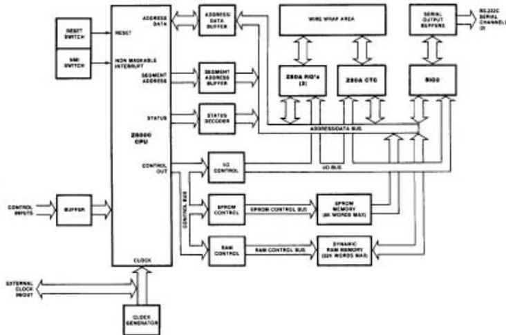
Figure 3. Block Diagram of Z8000 DM
