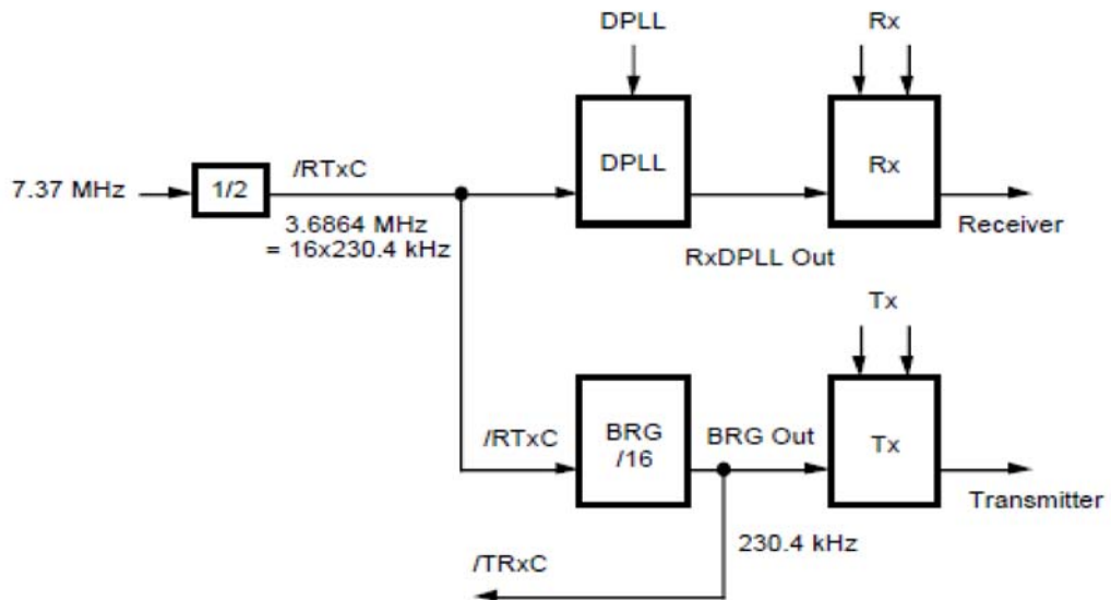
Figure 3. SCC Clocking Scheme
