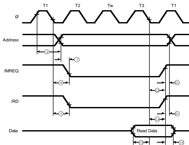
Z180 Memory Read Cycle Timing (One Wait State)
