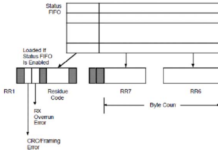
Figure 8. Status FIFO
