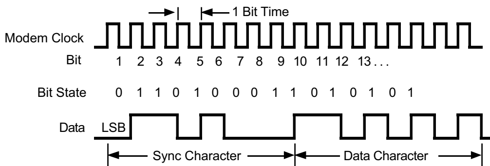
Monosync Data Character Format
