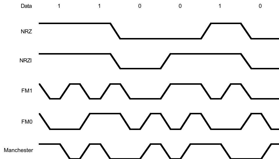
NRZ (NRZI), FM1 (FM0) Timing
