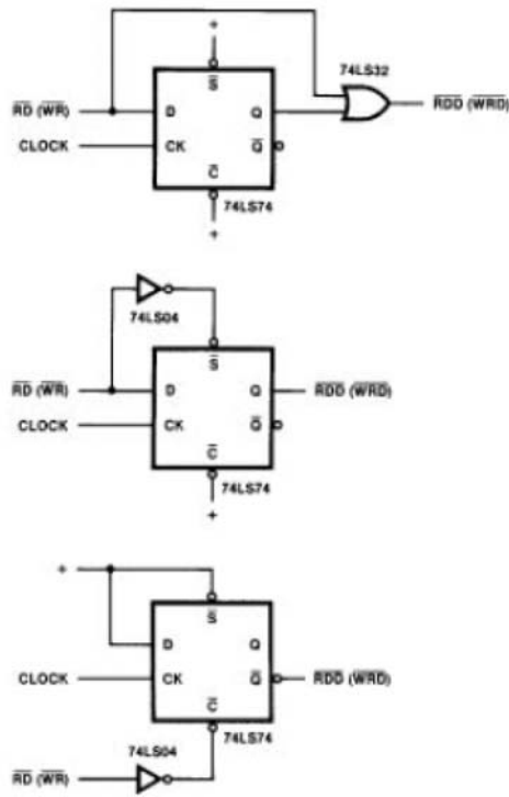
Figure 8. Delaying \overline{RD} or \overline{WR}
