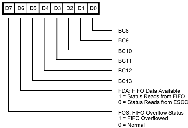
Read Register 7 *
