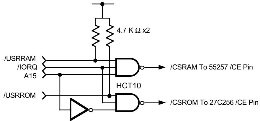
Memory Interface Logic
