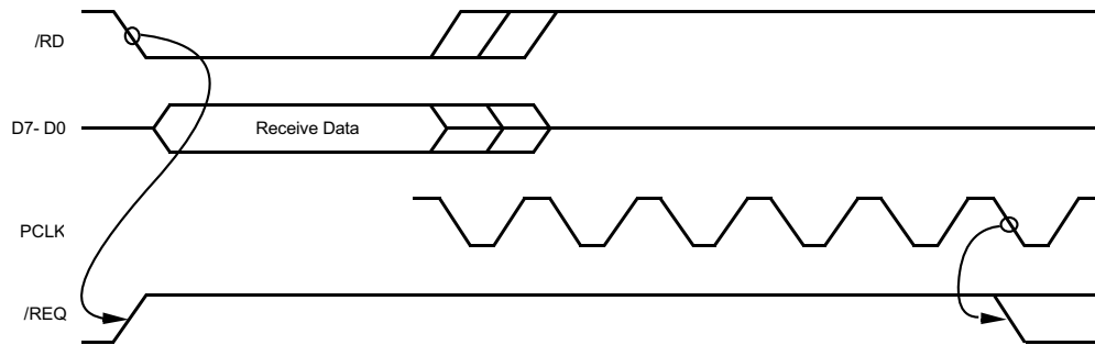
Z85X30 Receive Request Release
