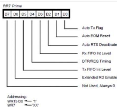
Figure 1. WR7' Definition
