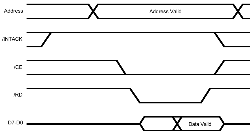
SCC Read Cycle Timing
