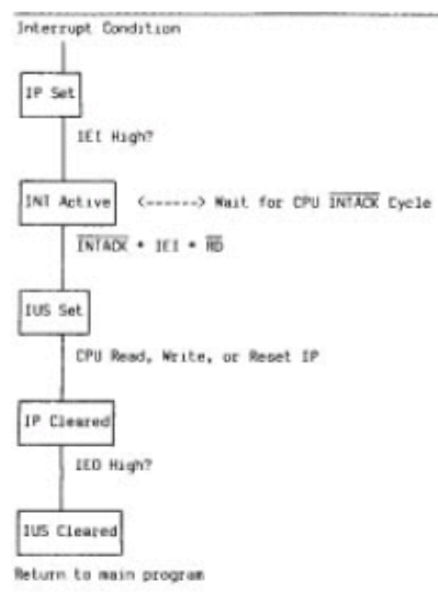
Figure 3. Z8500 Interrupt State Diagram
