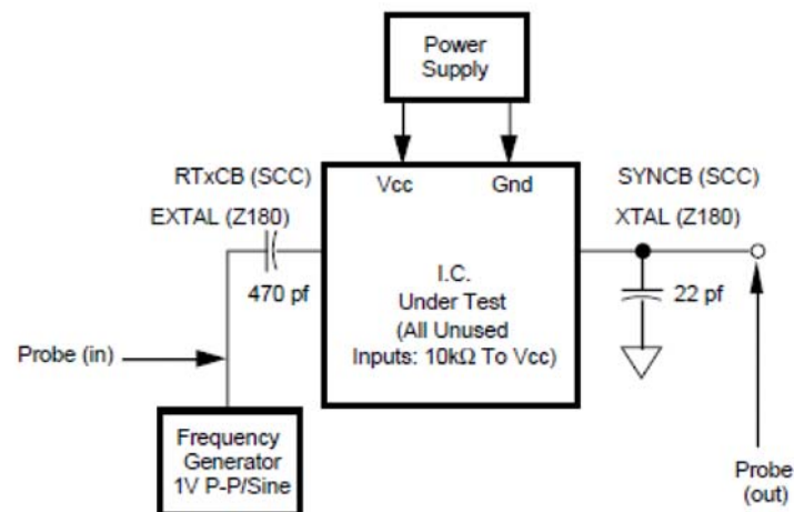
Figure 6. Gain Measurement
