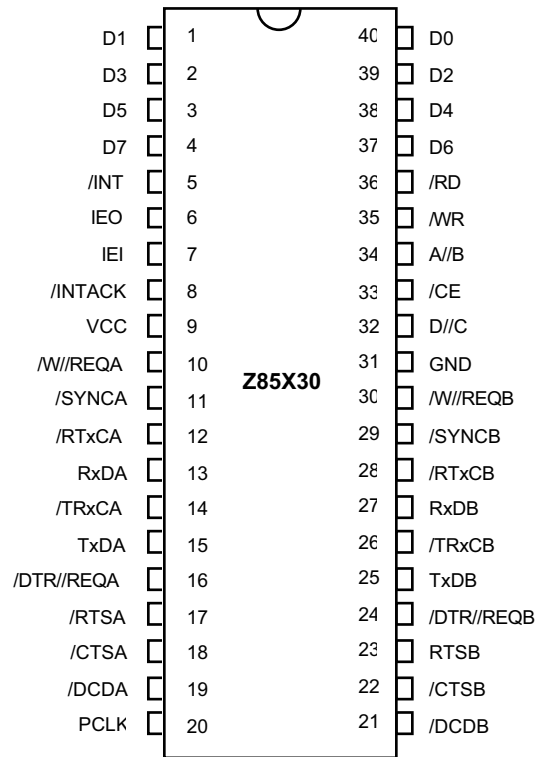
Z85X30 DIP Pin Assignments
