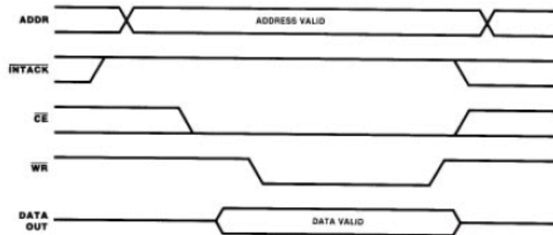
Figure 2. Z8500 Peripheral I/O Write Cycle Timing
