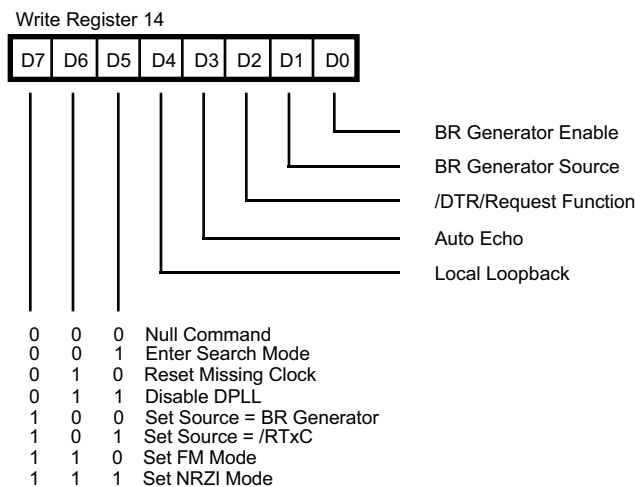
Write Register 14
