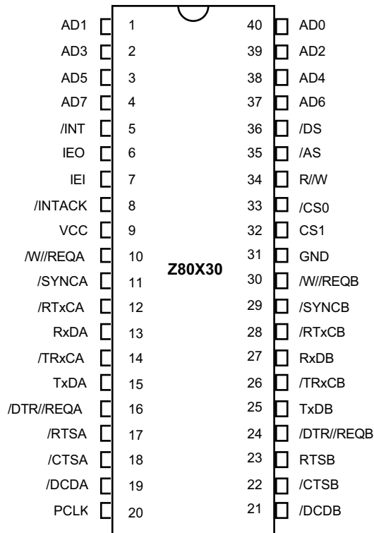
Z80X30 DIP Pin Assignments
