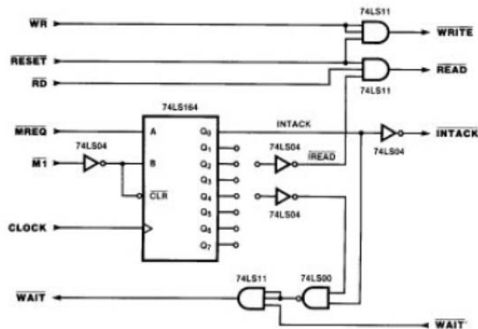
Figure 9. Z80A/Z80B CPU to Z8500/Z8500A Peripheral Interrupt Acknowledge Interface Logic
