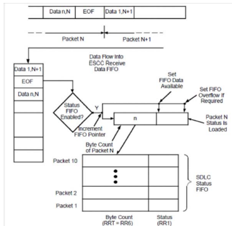
Figure 9. Status FIFO Operation at End Of Frame
