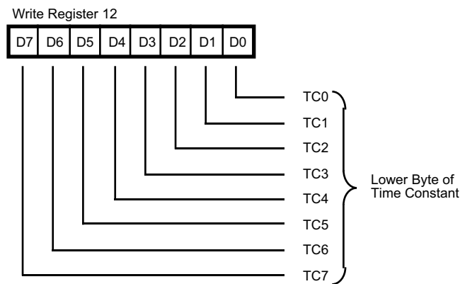
Write Register 12
