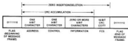
Figure 1. Fields of the SDLC Transmission Frame
