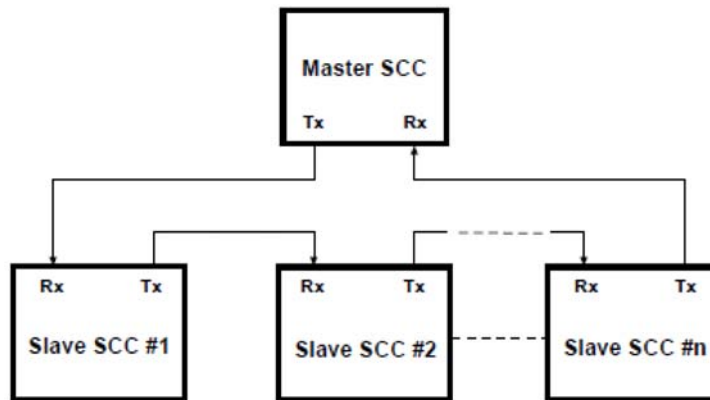
Figure 5. SDLC Loop Mode Configuration
