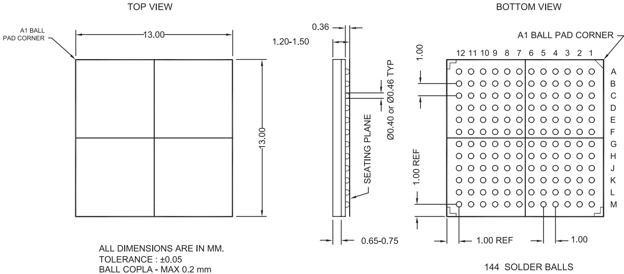
Figure 45. 144-Lead Chip Array Ball Grid Array
