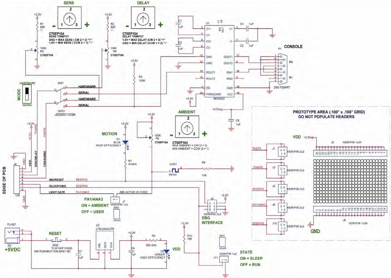
Figure & Schematic Diagram of the ZDMII Evaluation Board
