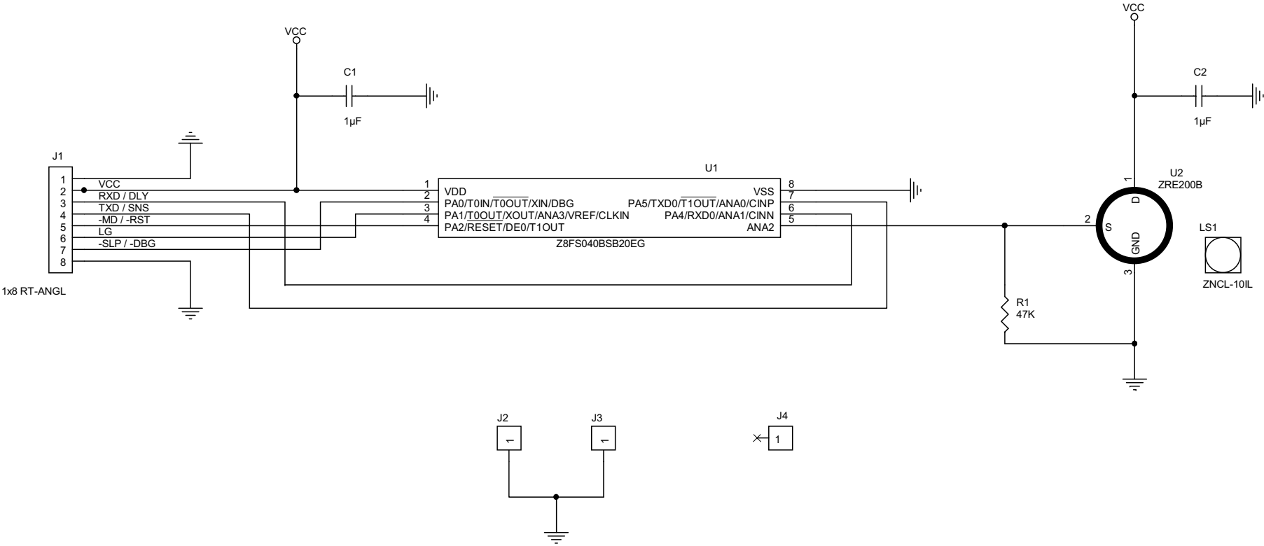
Figure % Schematic Diagram of the ZMOTION Detection Module II
