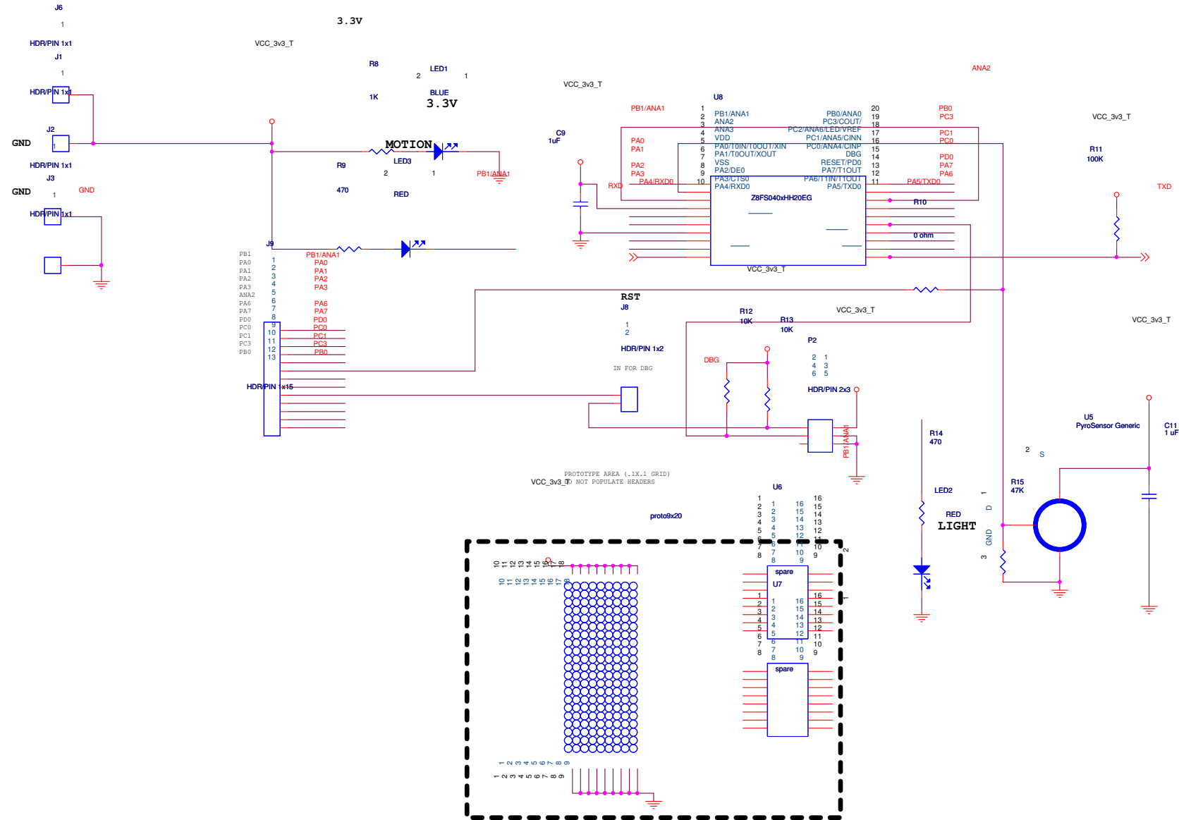
Figure 17 displays the schematics for the ZMOTION 20-Pin Development Board.
