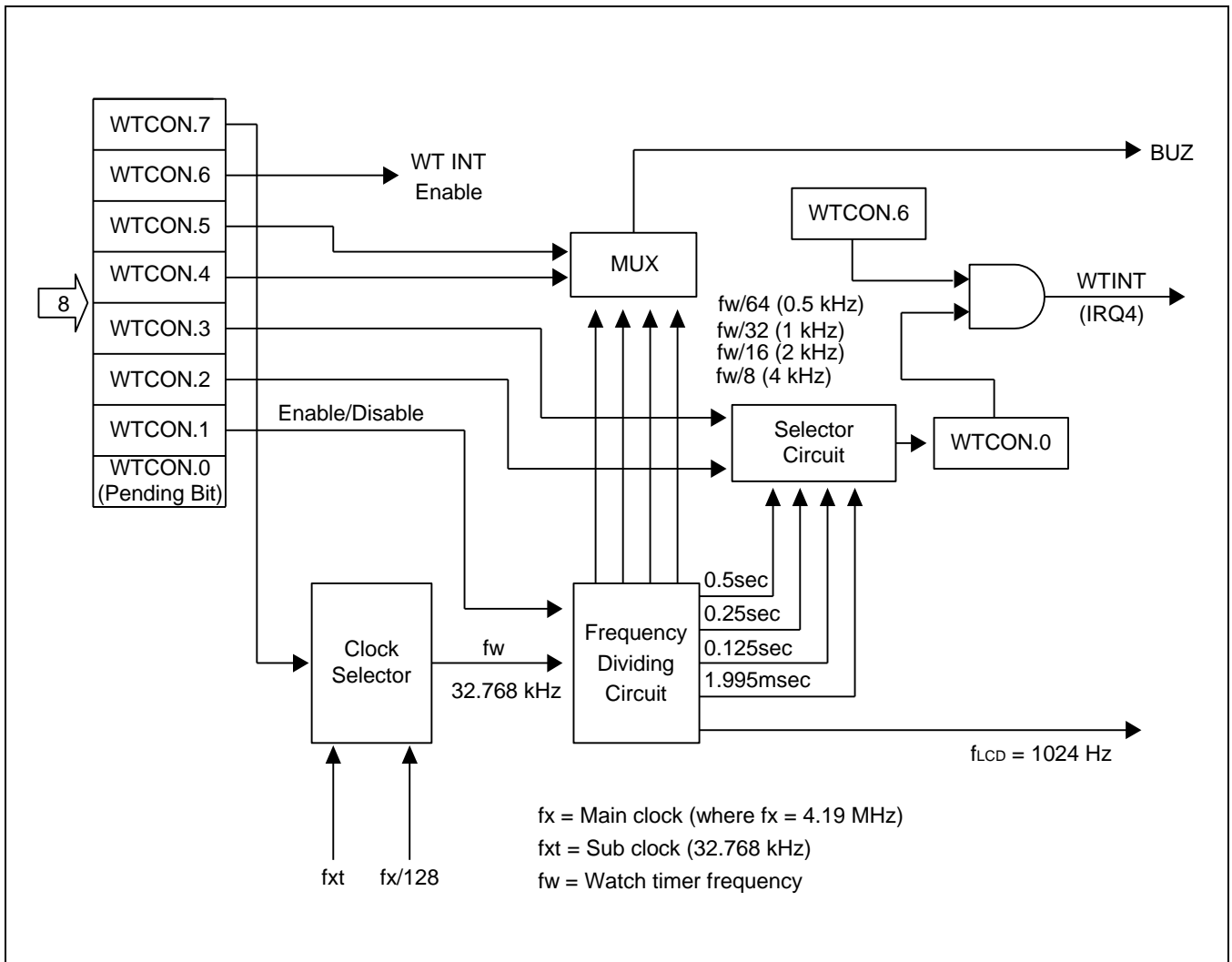
Figure 14-2 Watch Timer Circuit Diagram
