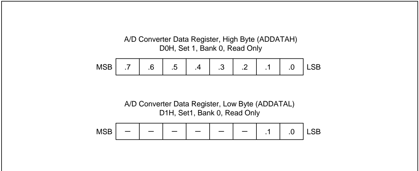
Figure 17-2 A/D Converter Data Register (ADDATAH/L)
