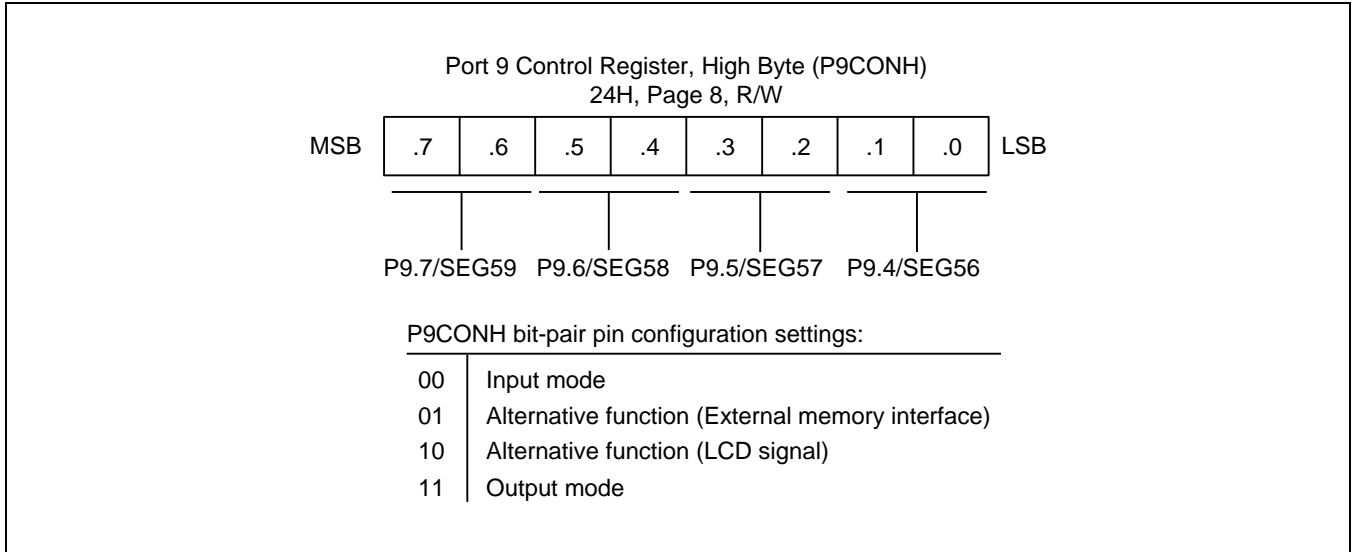
Figure 9-37 Port 9 High-byte Control Register (P9CONH)
