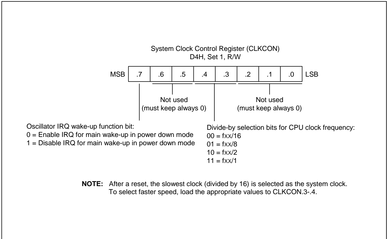
Figure 7-7 System Clock Control Register (CLKCON)
