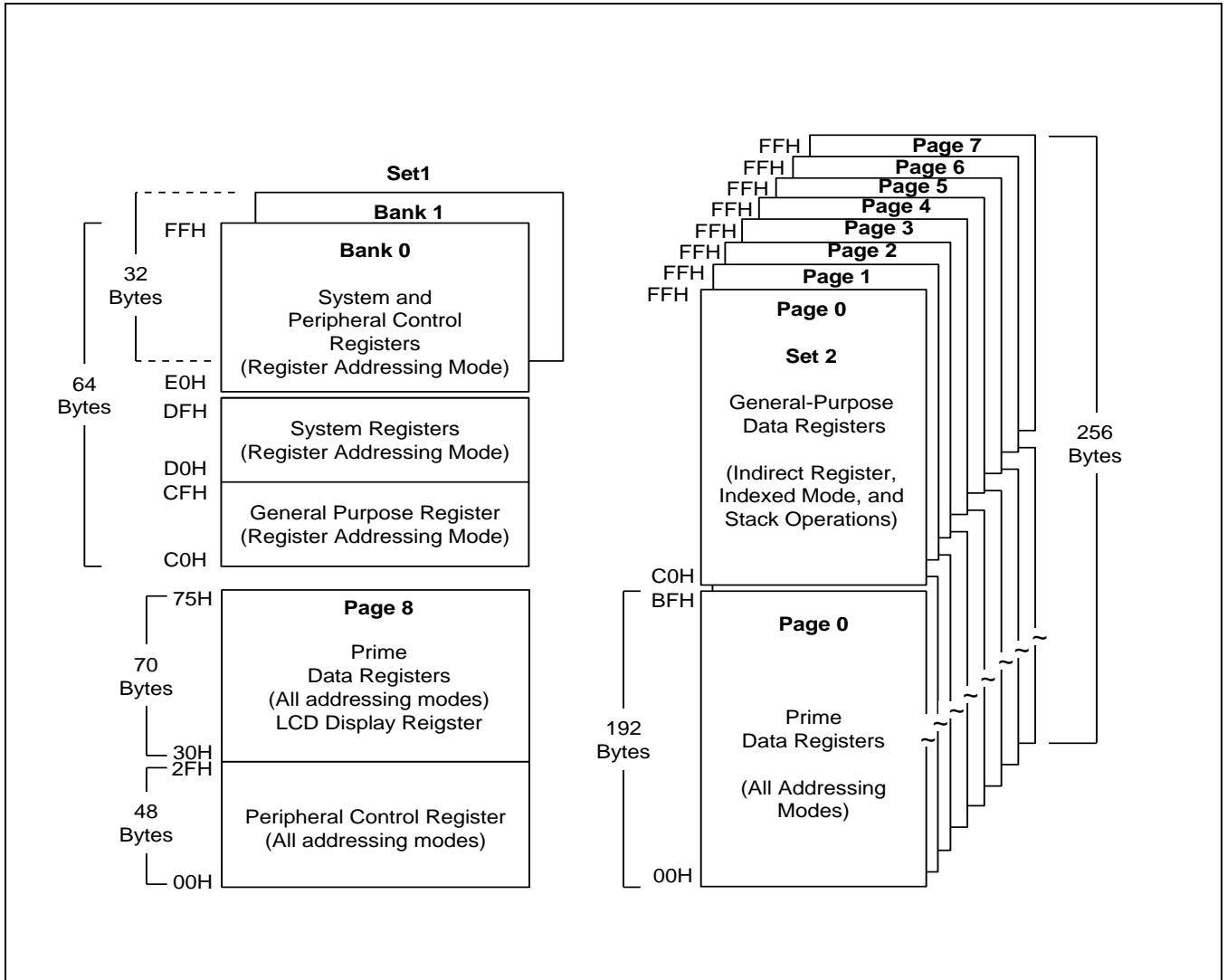
Figure 2-3 Internal Register File Organization (S3F8S8B)
