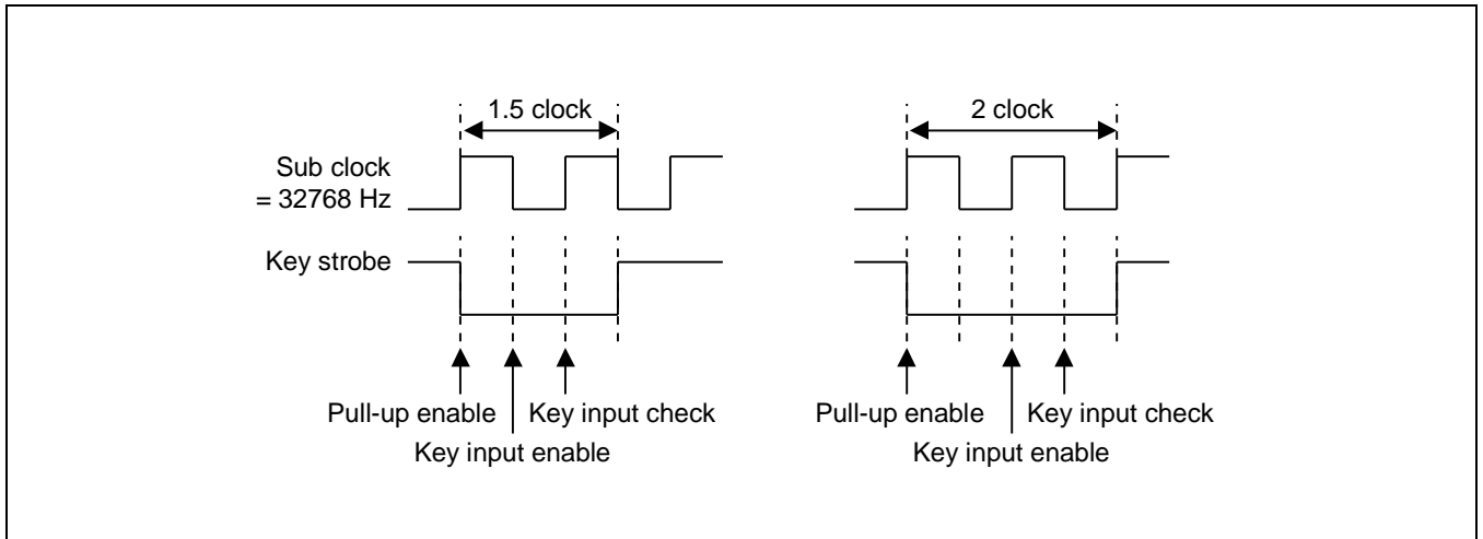
Figure 16-3 Key Input Check Sequence during Key Strobe out Duration
