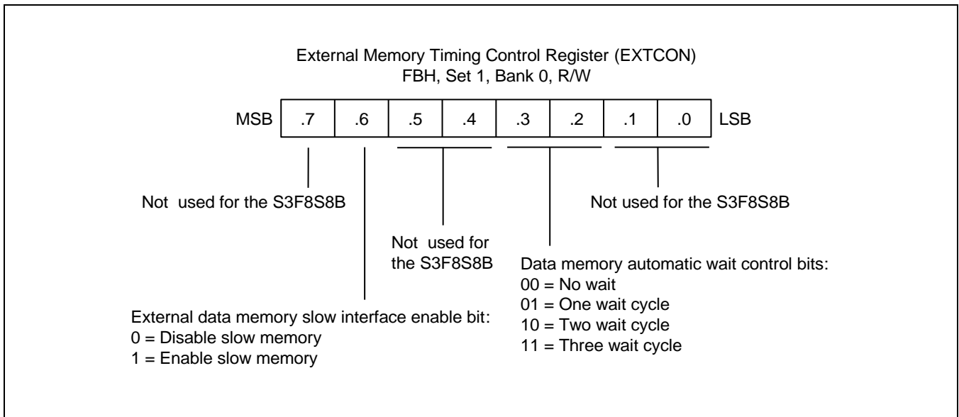
Figure 24-5 External Memory Timing Control Register (EXTCON)
