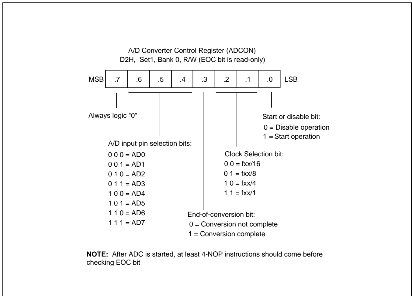
Figure 17-1 A/D Converter Control Register (ADCON)
