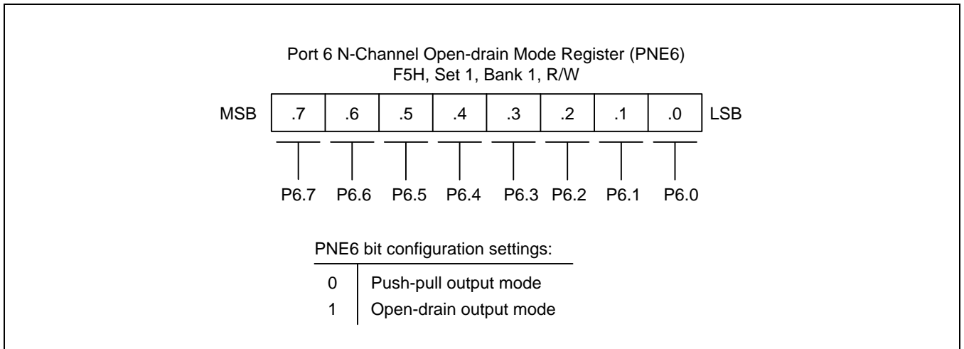
Figure 9-28 Port 6 N-Channel Open-drain Mode Register (PNE6)
