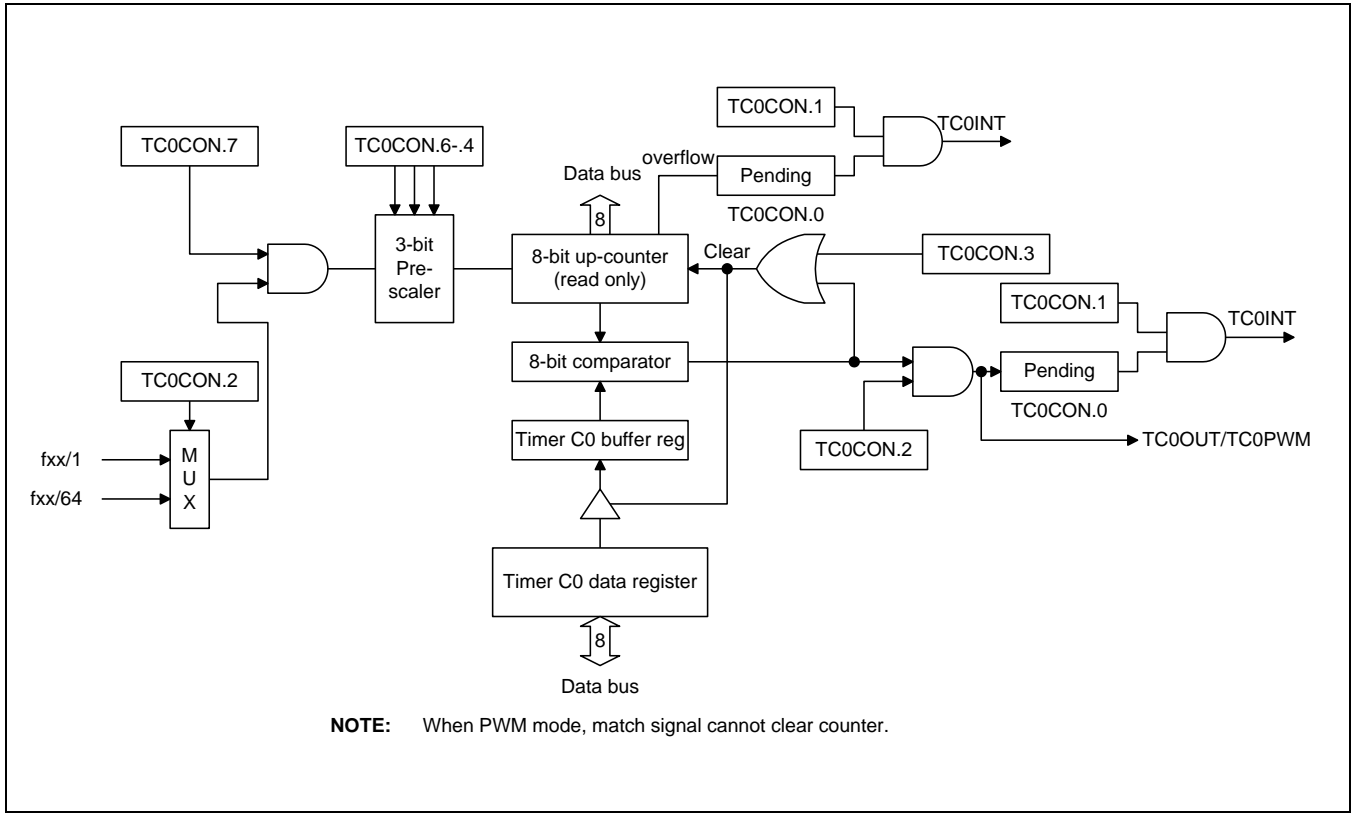
Figure 12-2 Timer C0 Functional Block Diagram
