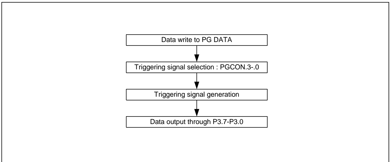
Figure 23-1 Pattern Generation Flow
