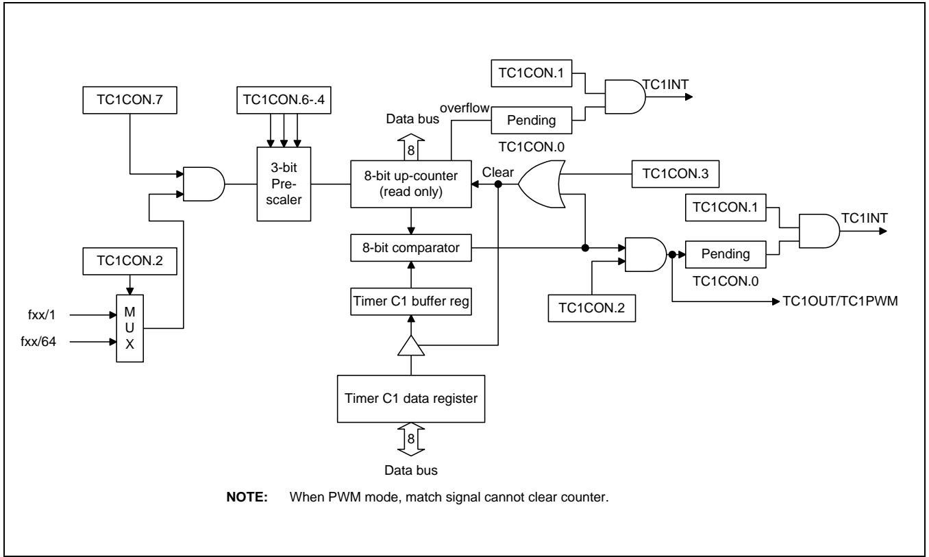
Figure 12-4 Timer C1 Functional Block Diagram
