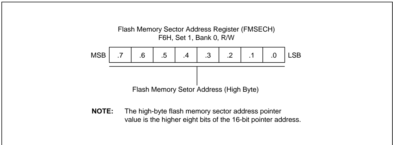
Figure 25-3 Flash Memory Sector Address Register High Byte (FMSECH)
