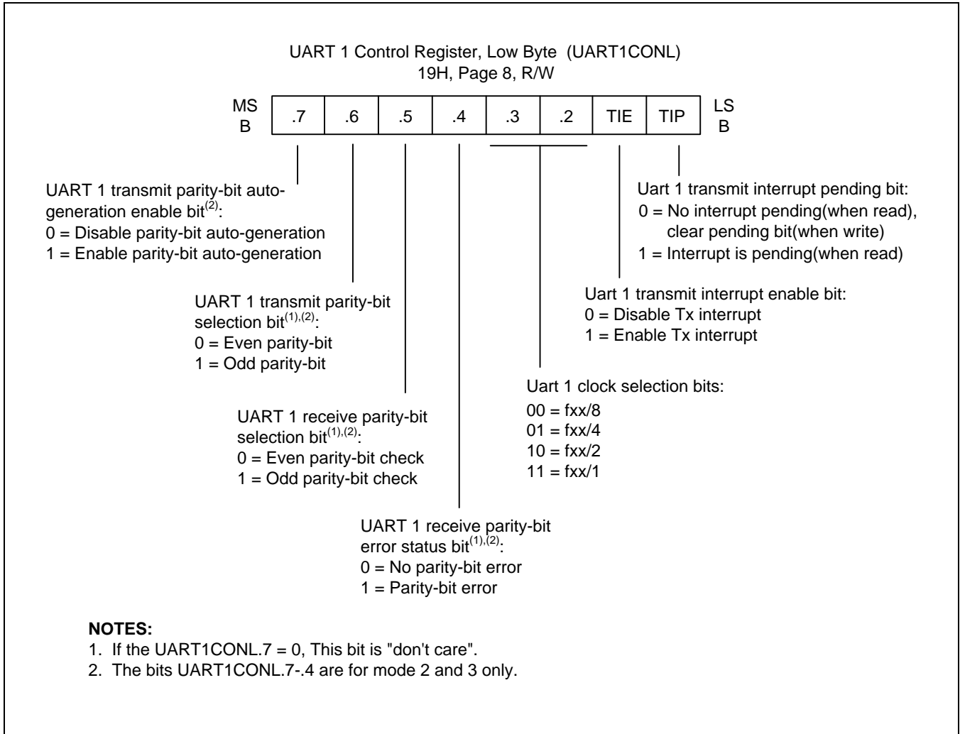
Figure 21-2 UART 1 Low Byte Control Register (UART1CONL)
