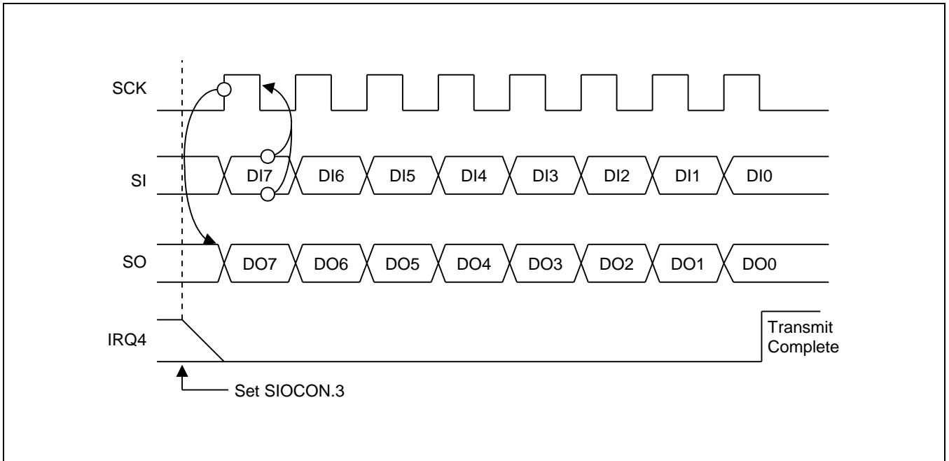
Figure 19-5 Serial I/O Timing in Transmit/Receive Mode (Tx at rising, SIOCON.4 = 1)
