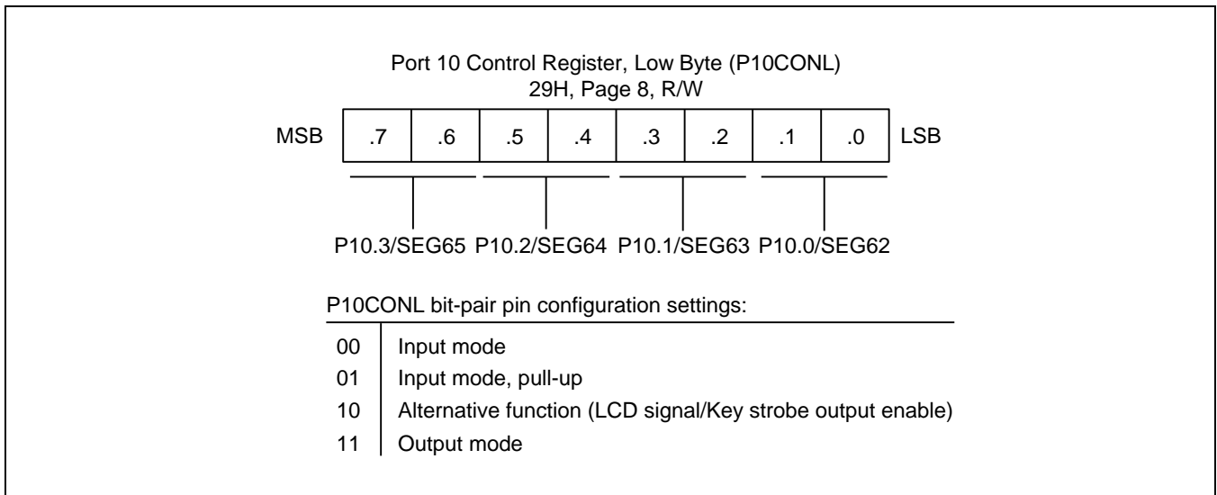
Figure 9-42 Port 10 Low-byte Control Register (P10CONL)
