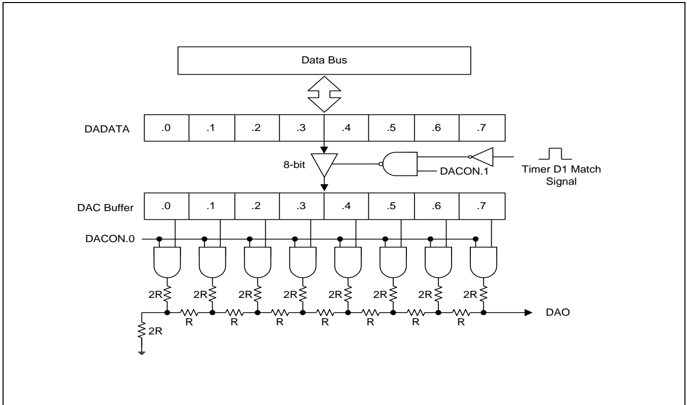
Figure 18-1 DAC Circuit Diagram
