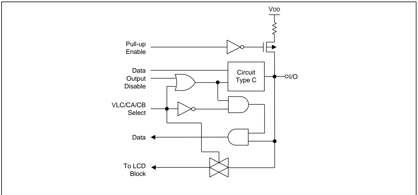
Figure 1-8 Pin Circuit Type F-17 (P5.0 - P5.5)
