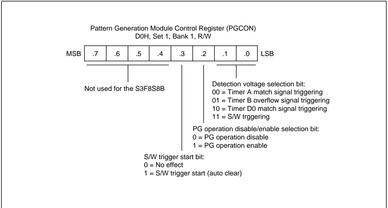
Figure 23-2 Pattern Generation Control Register (PGCON)
