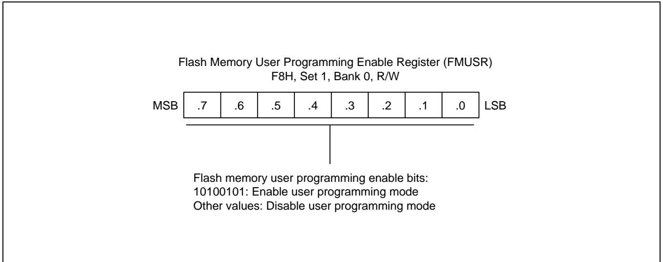
Figure 25-2 Flash Memory User Programming Enable Register (FMUSR)
