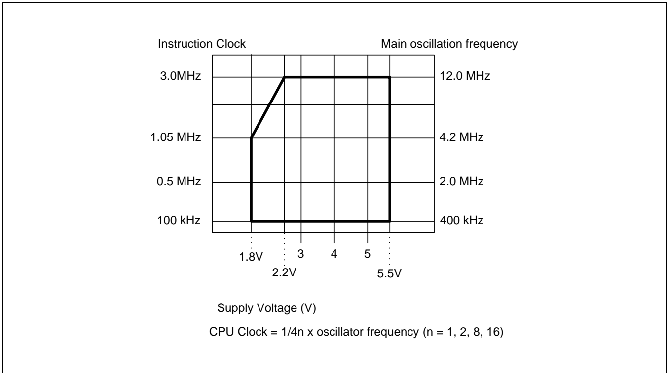
Figure 26-11 Operating Voltage Range
