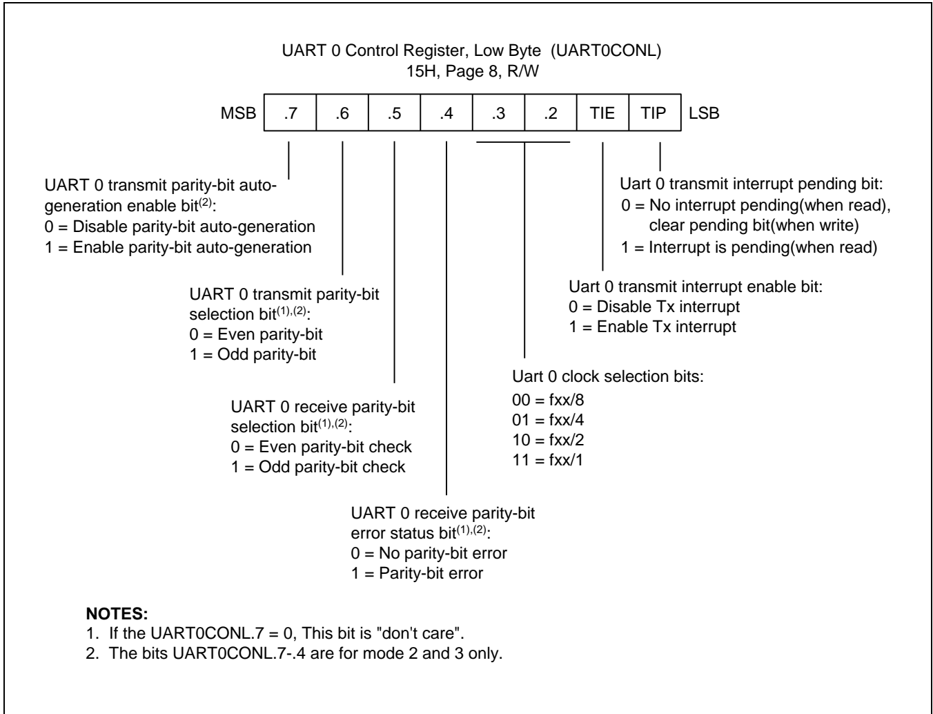
Figure 20-2 UART 0 Low Byte Control Register (UART0CONL)
