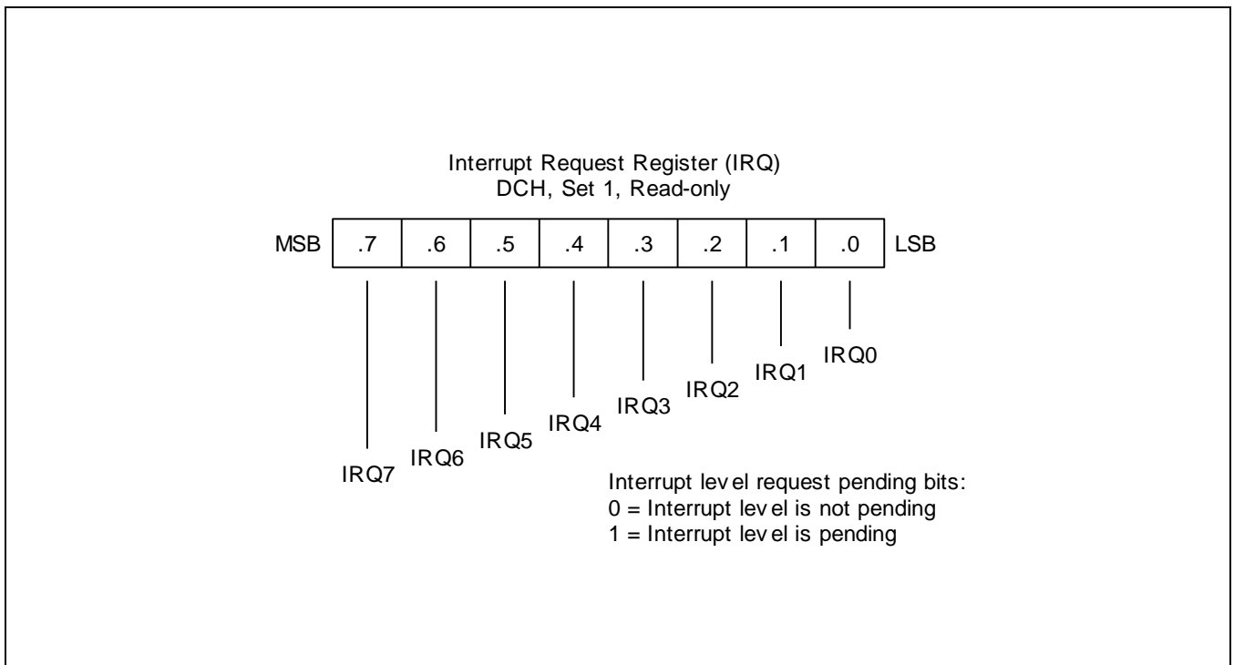
Figure 5-9 Interrupt Request Register (IRQ)
