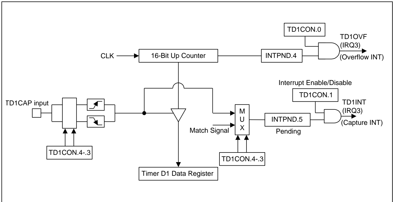
Figure 13-9 Simplified Timer D1 Function Diagram: Capture Mode
