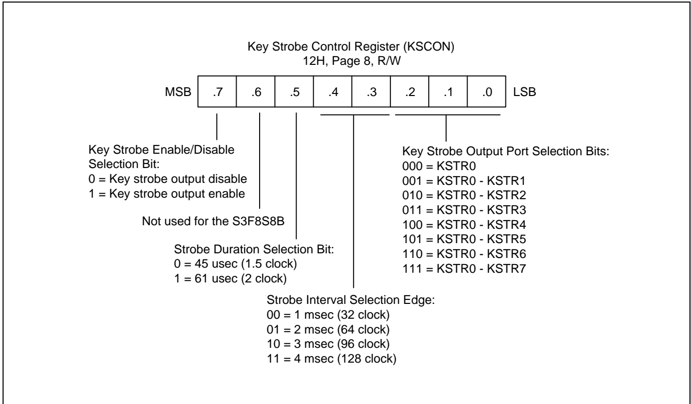
Figure 16-1 Key Strobe Control Register (KSCON)
