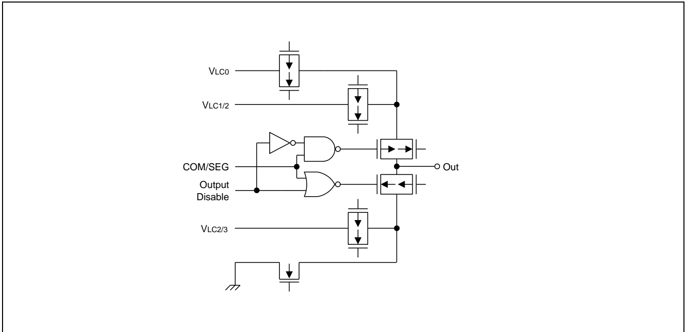
Figure 1-9 Pin Circuit Type H-39
