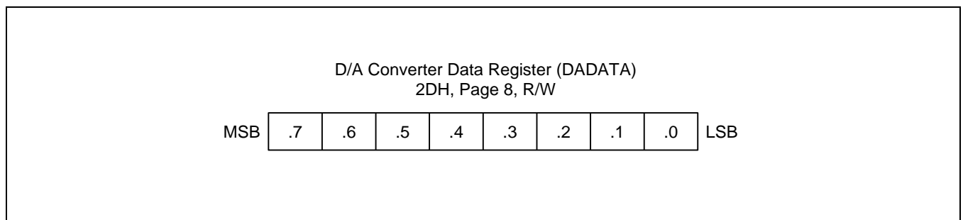
Figure 18-3 D/A Converter Data Register (DADATA)
