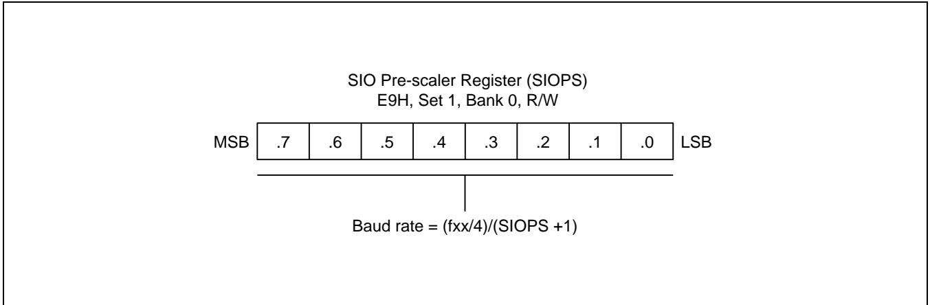
Figure 19-2 SIO Pre-scaler Register (SIOPS)
