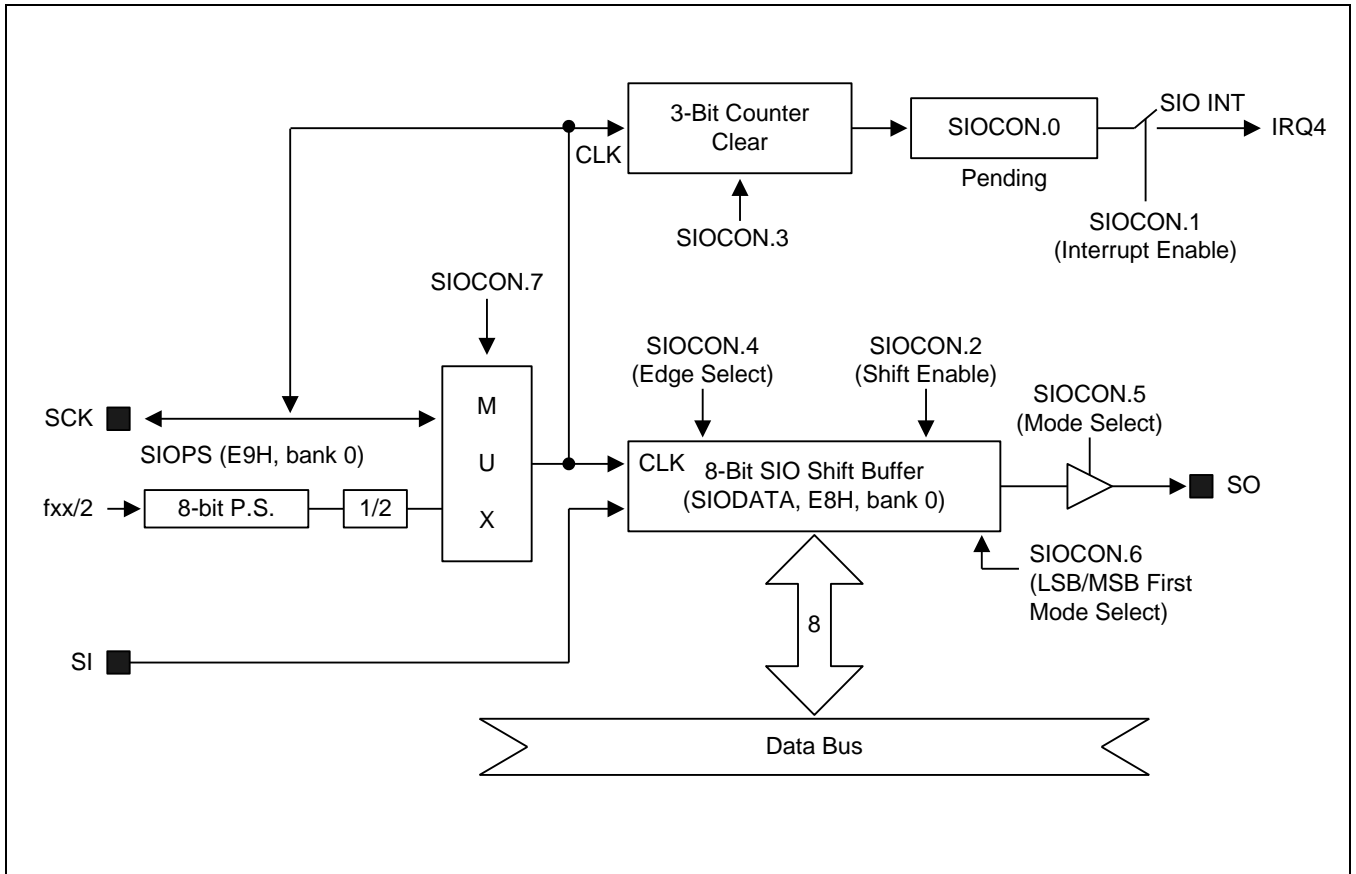
Figure 19-3 SIO Functional Block Diagram
