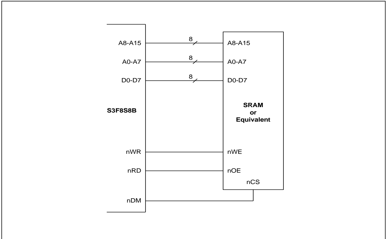
Figure 24-8 External Data Memory Interface Function Diagram (with SRAM)
