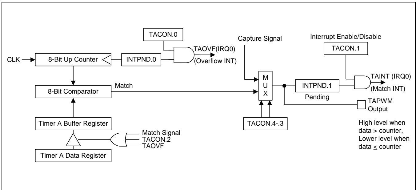
Figure 11-3 Simplified Timer A Function Diagram: PWM Mode
