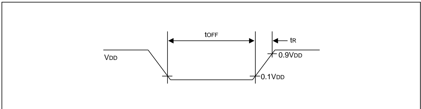
Figure 26-5 LVR (Low Voltage Reset) Timing
