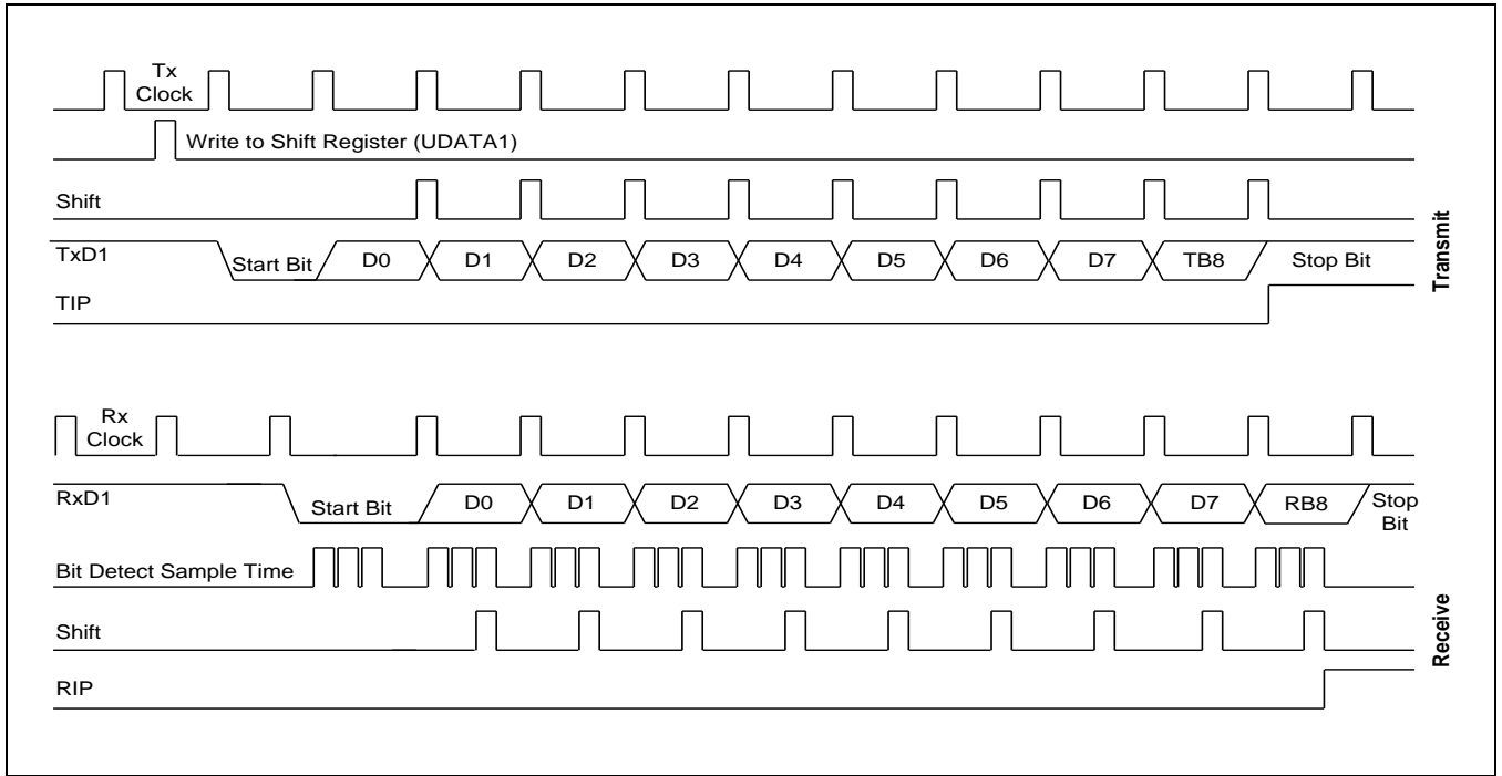
Figure 21-8 Timing Diagram for Serial Port Mode 2 Operation
