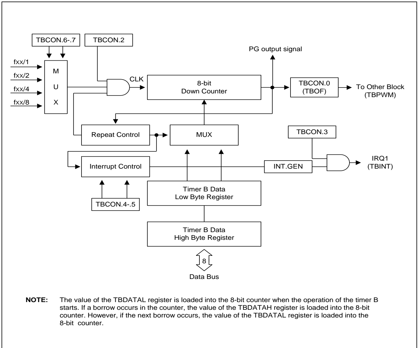
Figure 11-7 Timer B Functional Block Diagram
