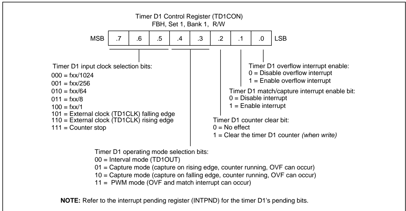
Figure 13-6 Timer D1 Control Register (TD1CON)
