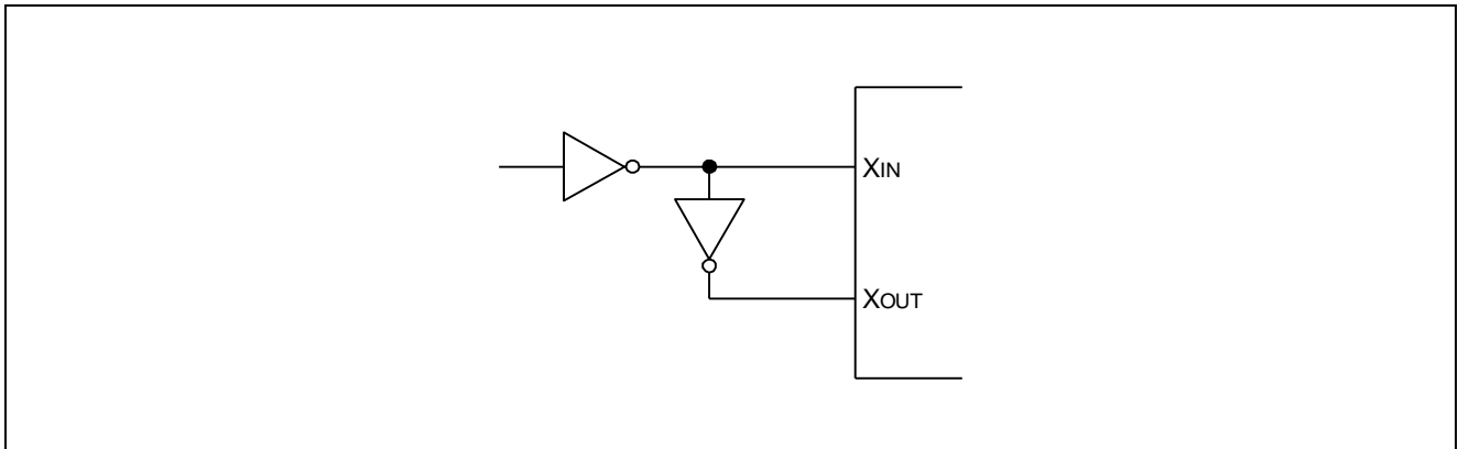
Figure 7-2 External Oscillator (fX)
