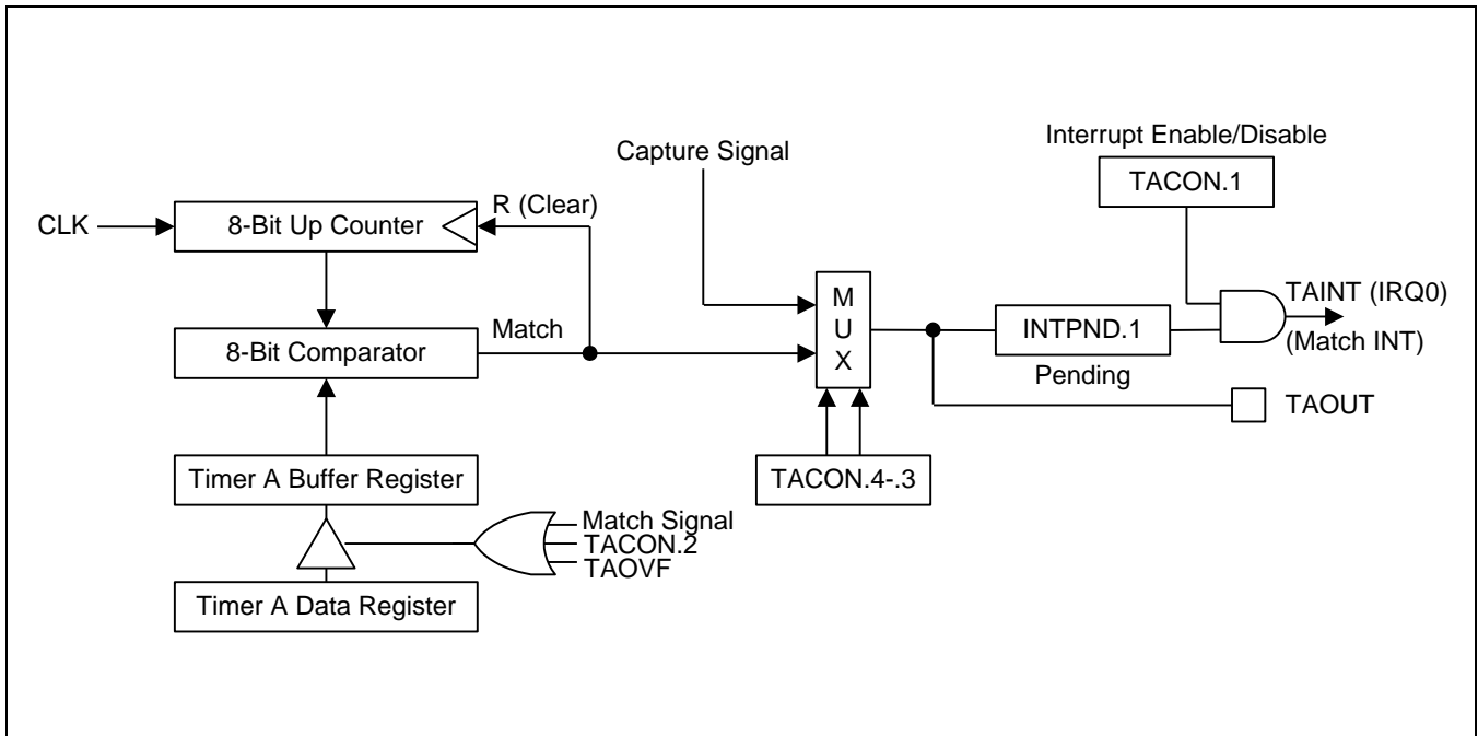
Figure 11-2 Simplified Timer A Function Diagram: Interval Timer Mode
