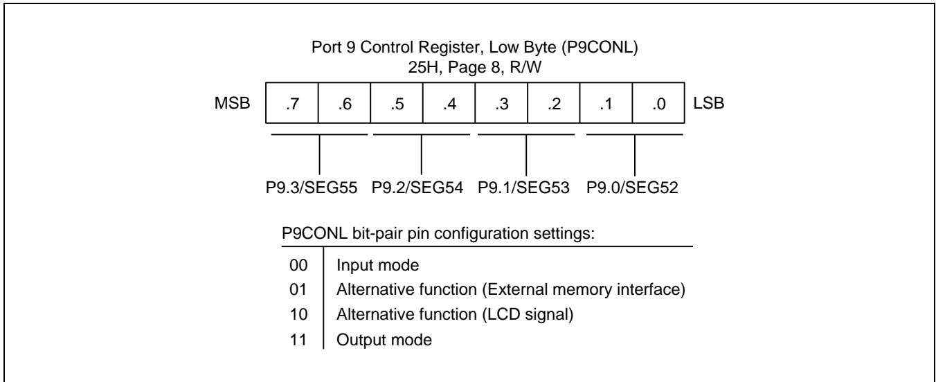
Figure 9-38 Port 9 Low-byte Control Register (P9CONL)
