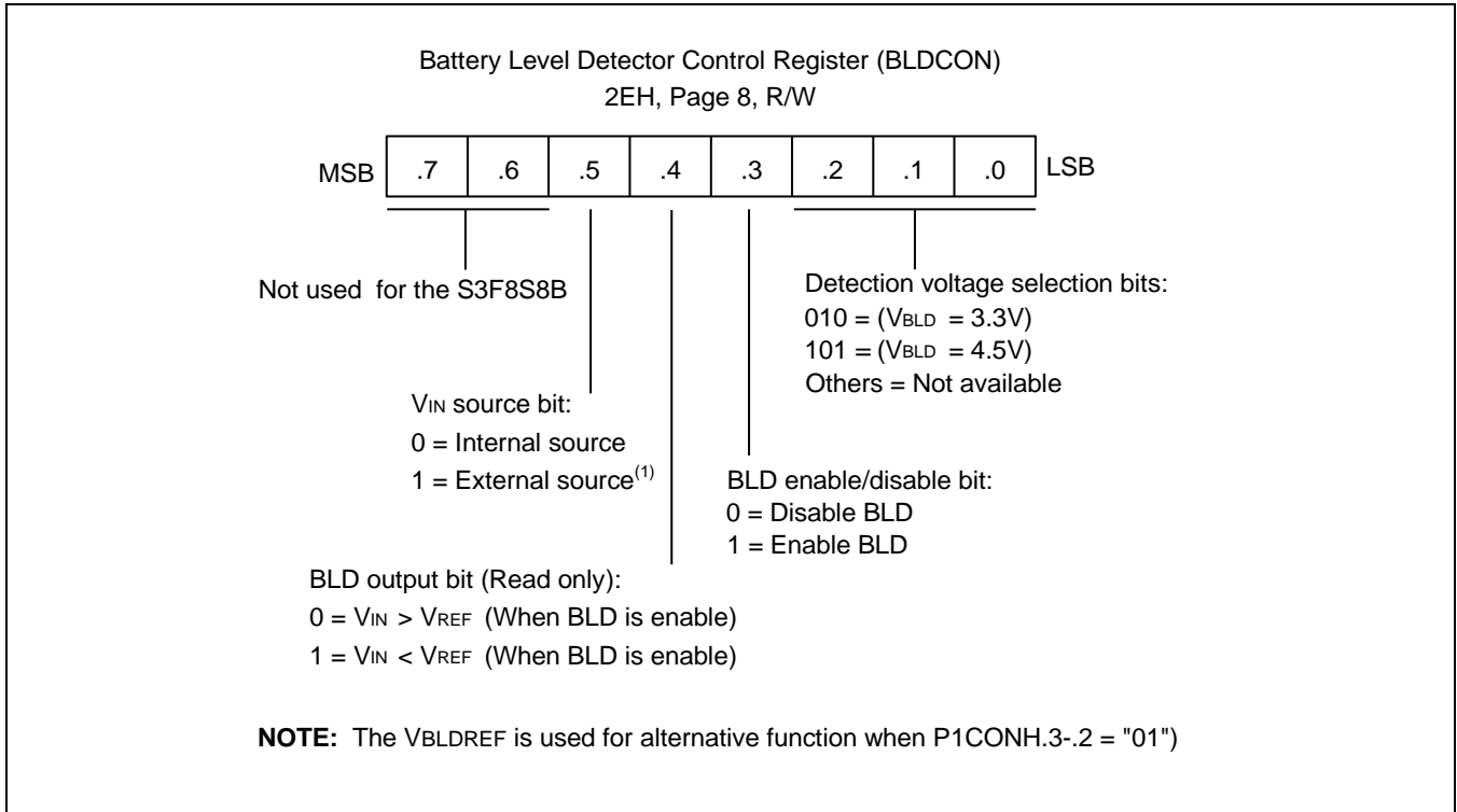
Figure 22-2 Battery Level Detector Control Register (BLDCON)
