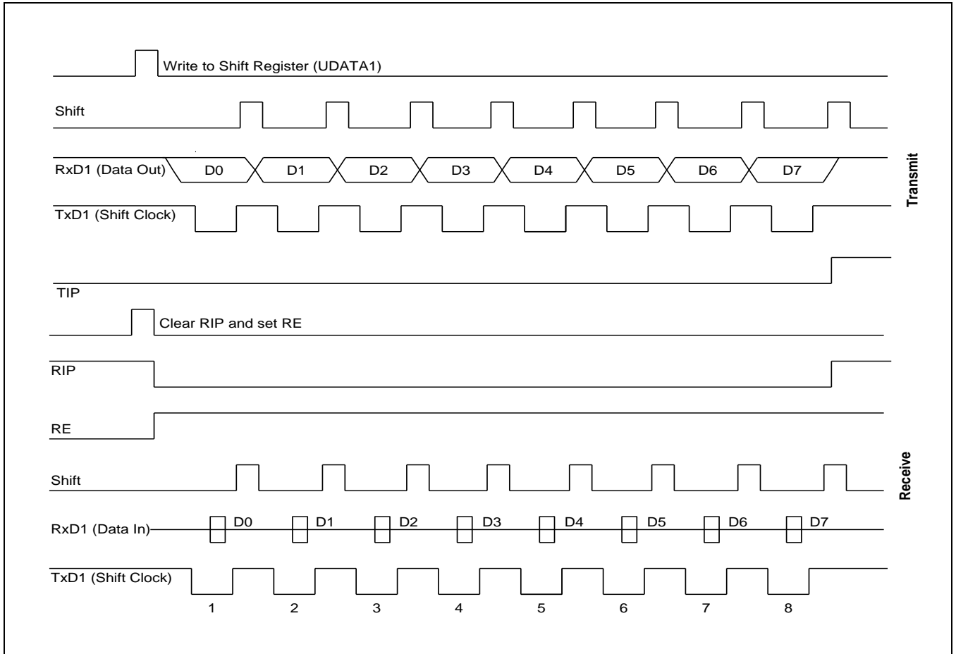
Figure 21-6 Timing Diagram for Serial Port Mode 0 Operation
