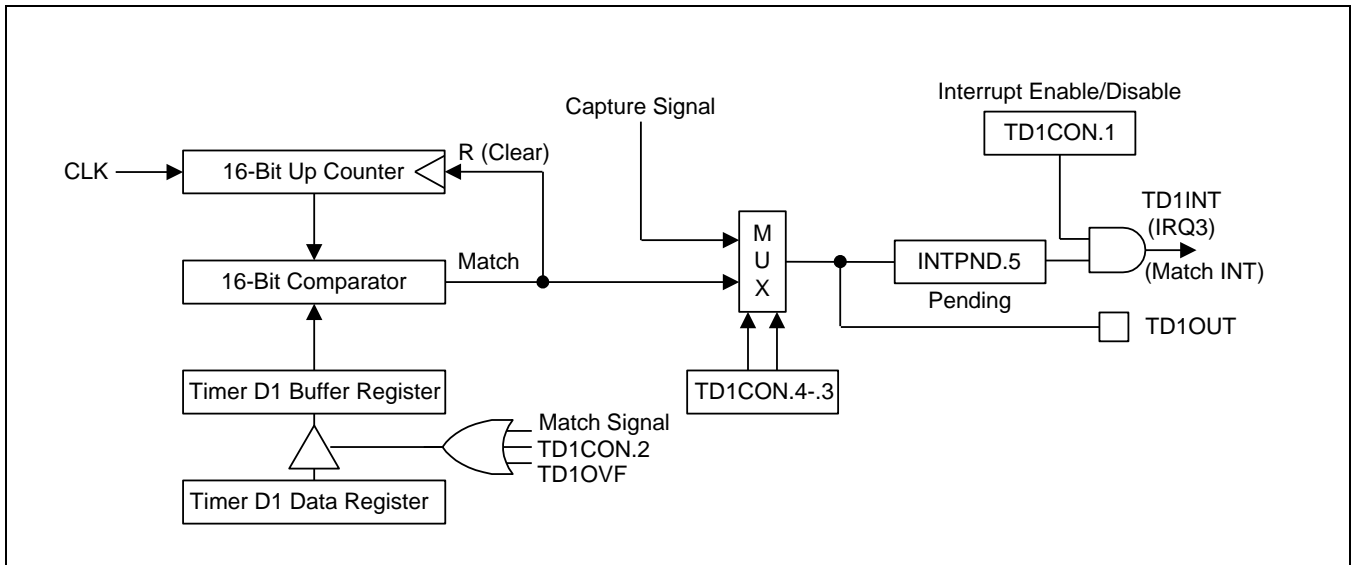
Figure 13-7 Simplified Timer D1 Function Diagram: Interval Timer Mode
