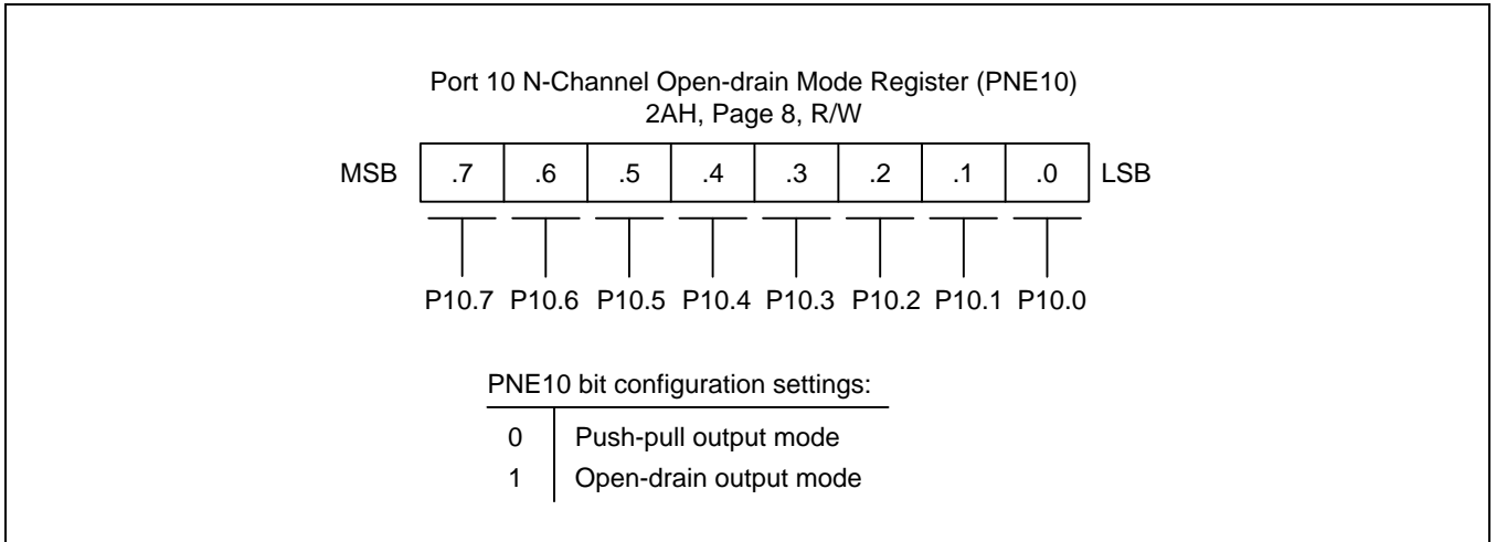
Figure 9-43 Port 10 N-Channel Open-drain Mode Register (PNE10)
