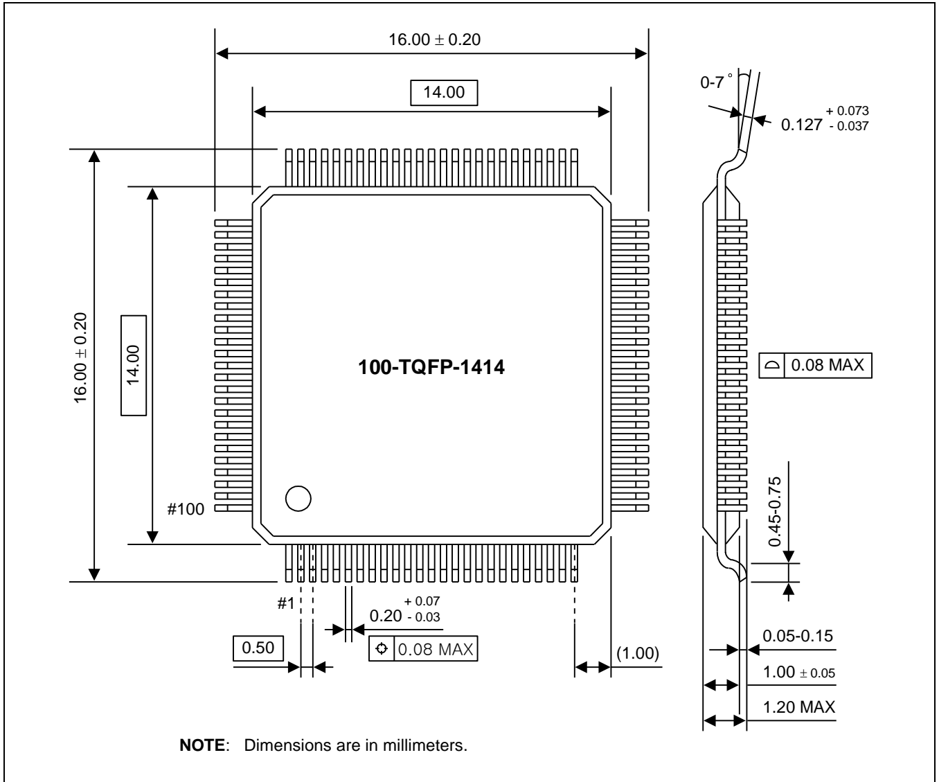
Figure 27-2 Package Dimensions (100-TQFP-1414)
