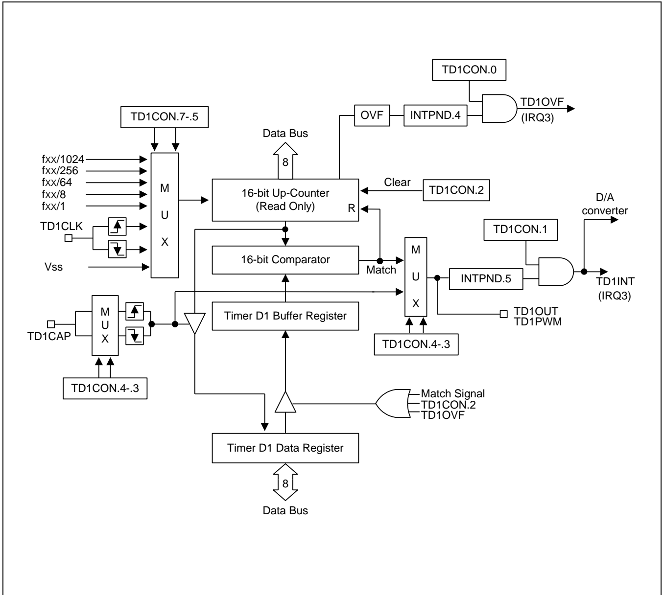
Figure 13-10 Timer D1 Functional Block Diagram
