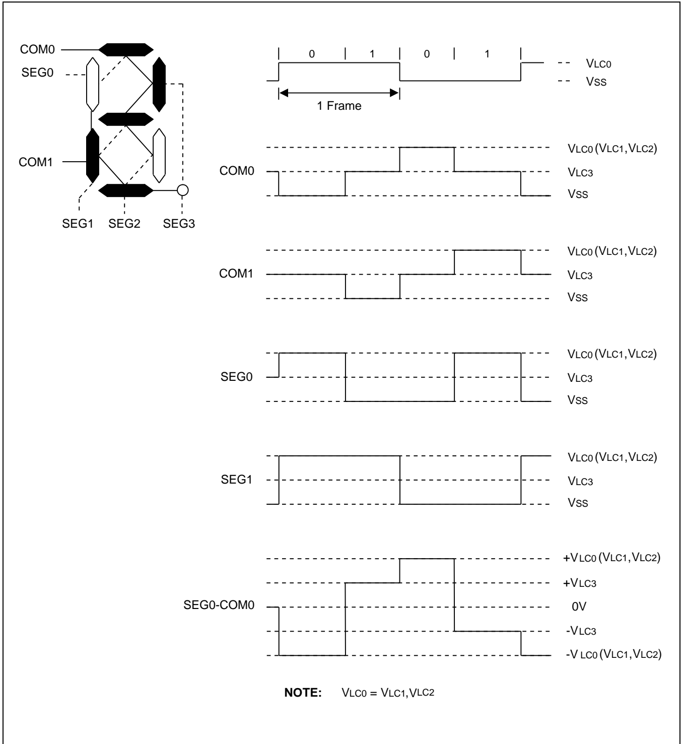
Figure 15-11 LCD Signal Waveforms (1/2 Duty, 1/2 Bias)
