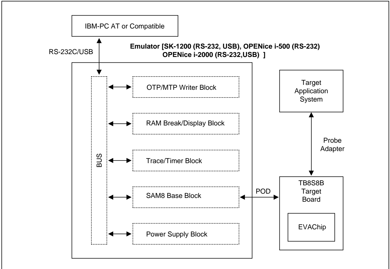
Figure 29-1 Emulator Product Configuration
