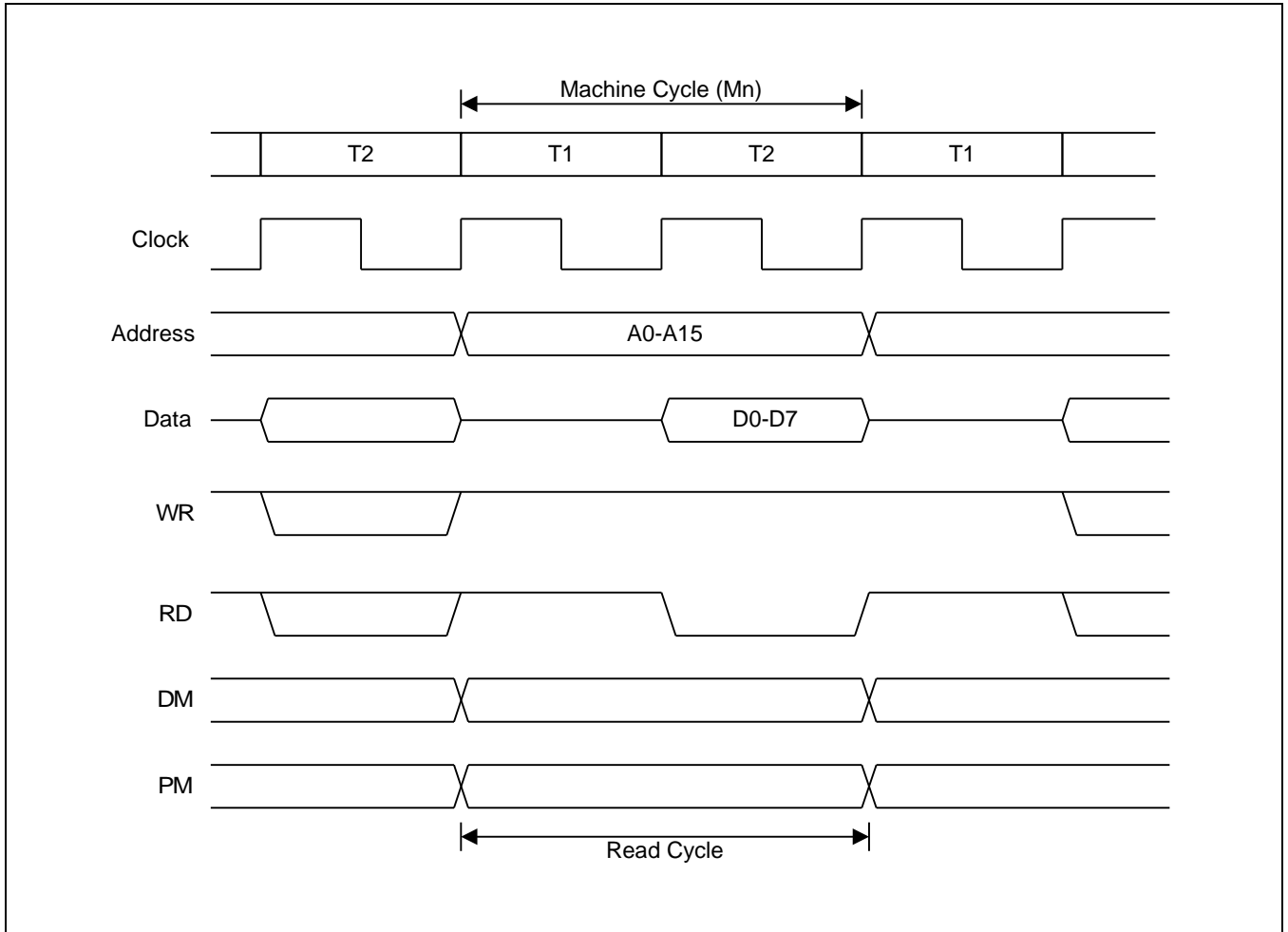
Figure 24-7 External Bus Read Cycle Timing Diagram
