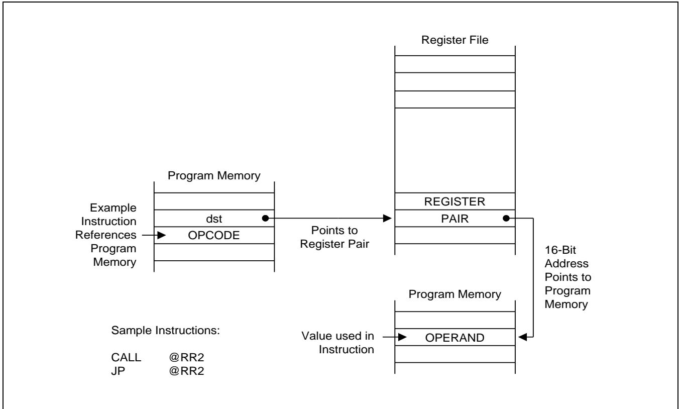
Figure 3-4 Indirect Register Addressing to Program Memory
