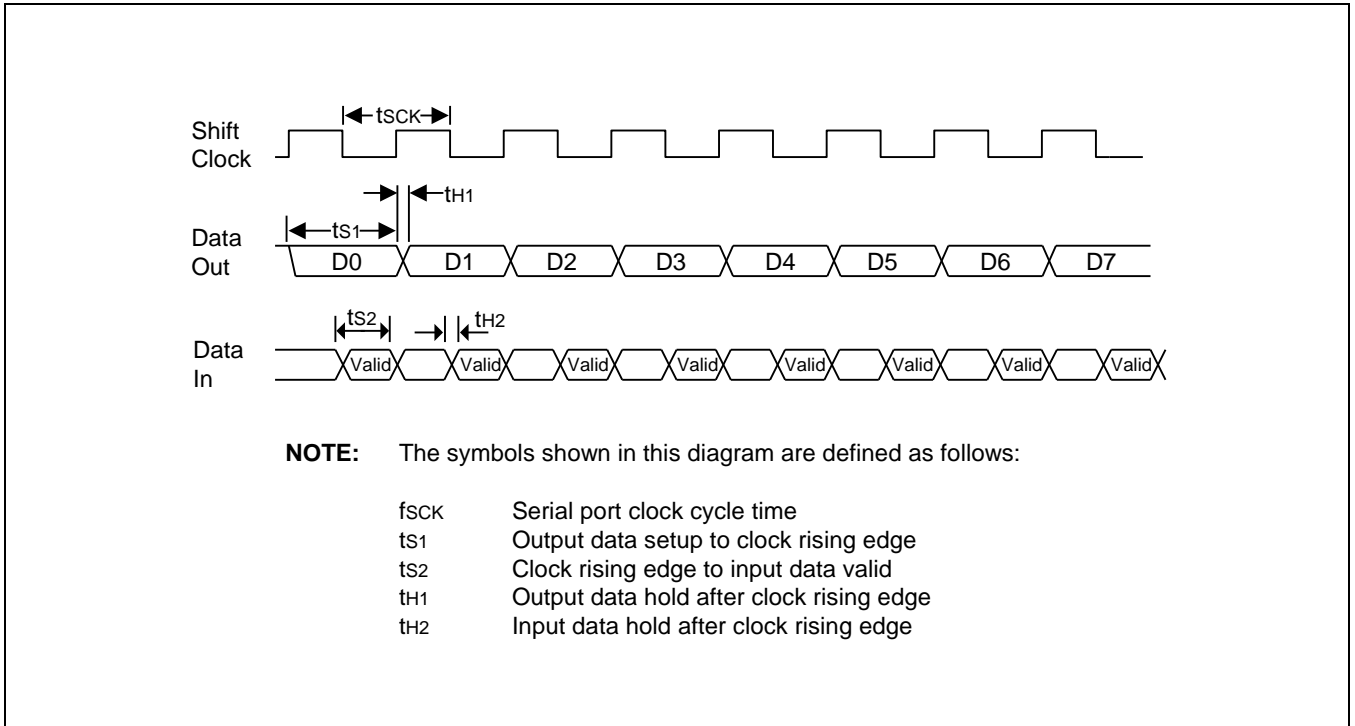
Figure 26-8 Timing Waveform for the UART Module
