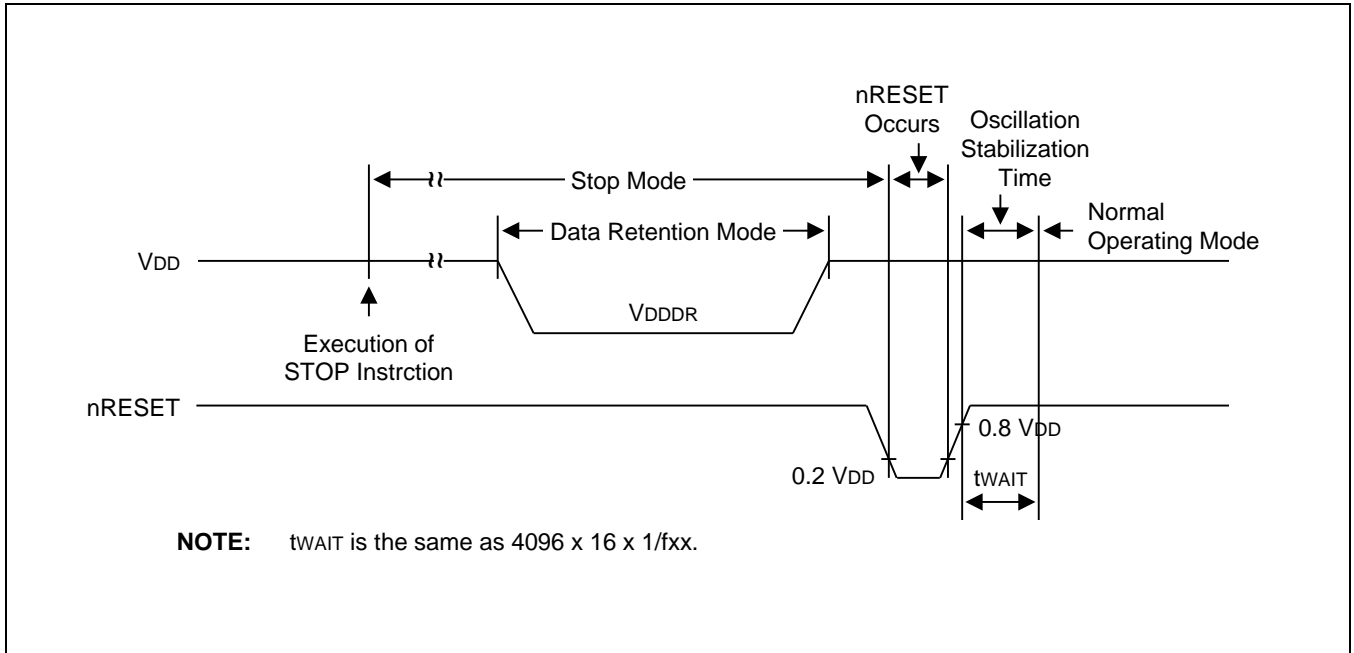
Figure 26-3 Stop Mode Release Timing Initiated by nRESET
