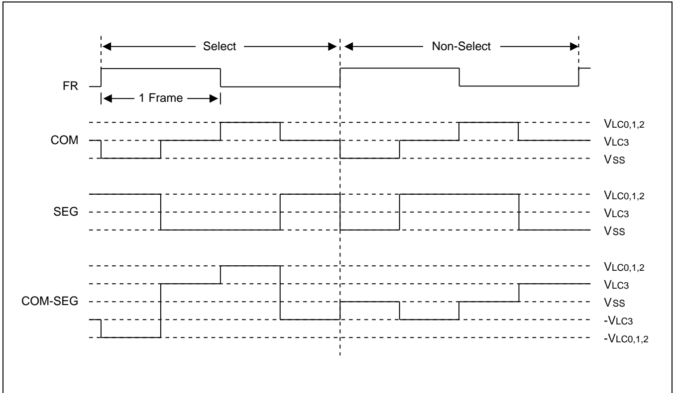
Figure 15-9 Select/No-Select Signal in 1/2 Duty, 1/2 Bias Display Mode
