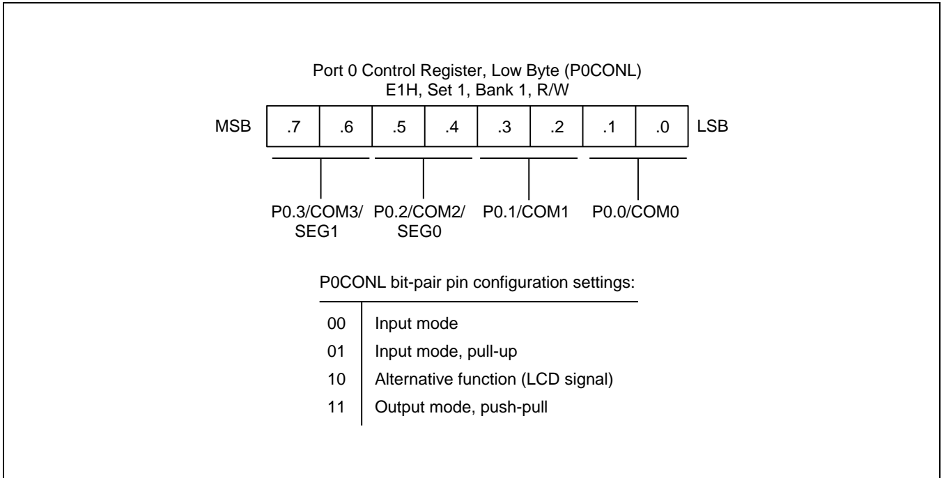
Figure 9-3 Port 0 Low-Byte Control Register (P0CONL)
