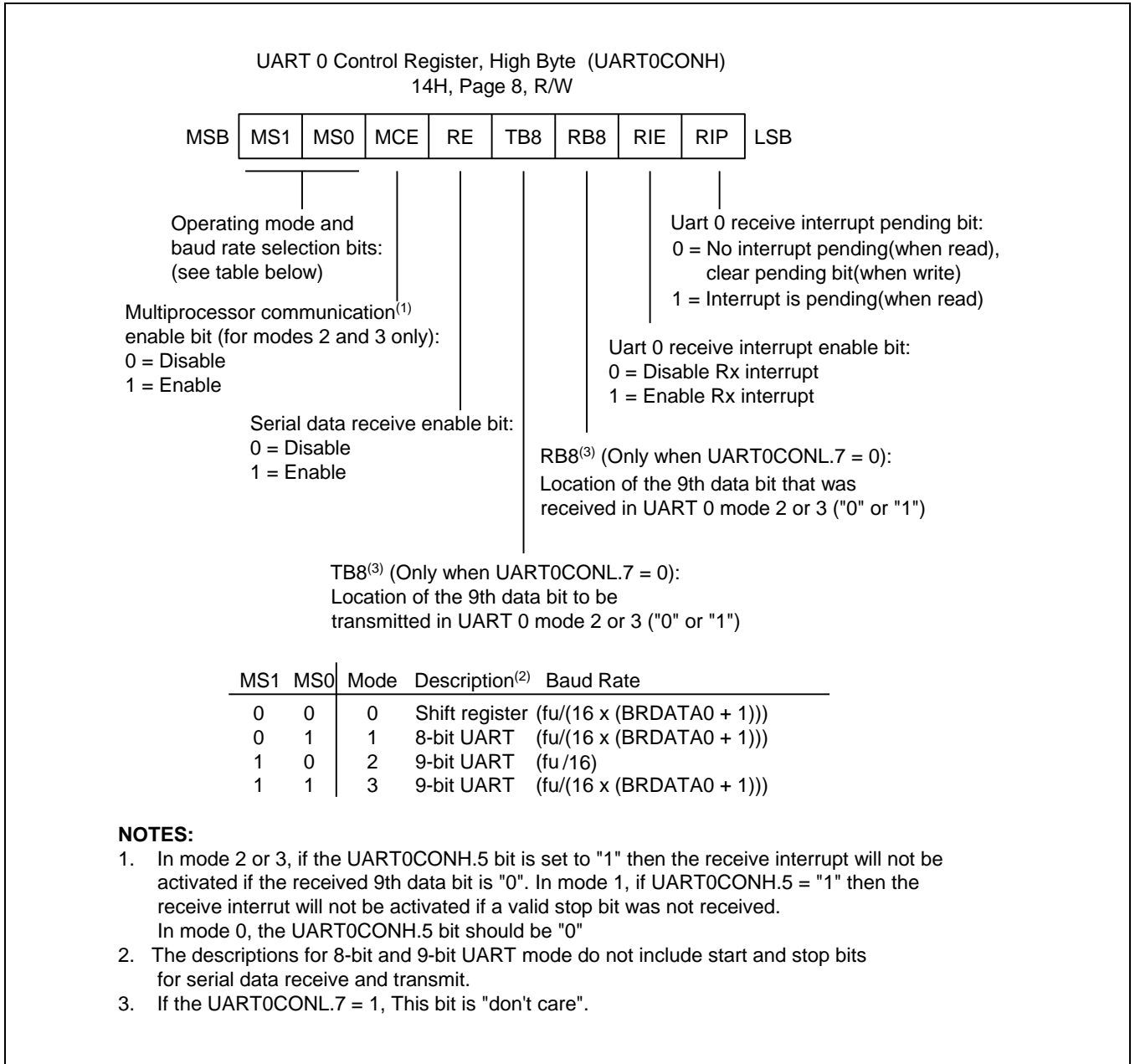
Figure 20-1 UART 0 High Byte Control Register (UART0CONH)
