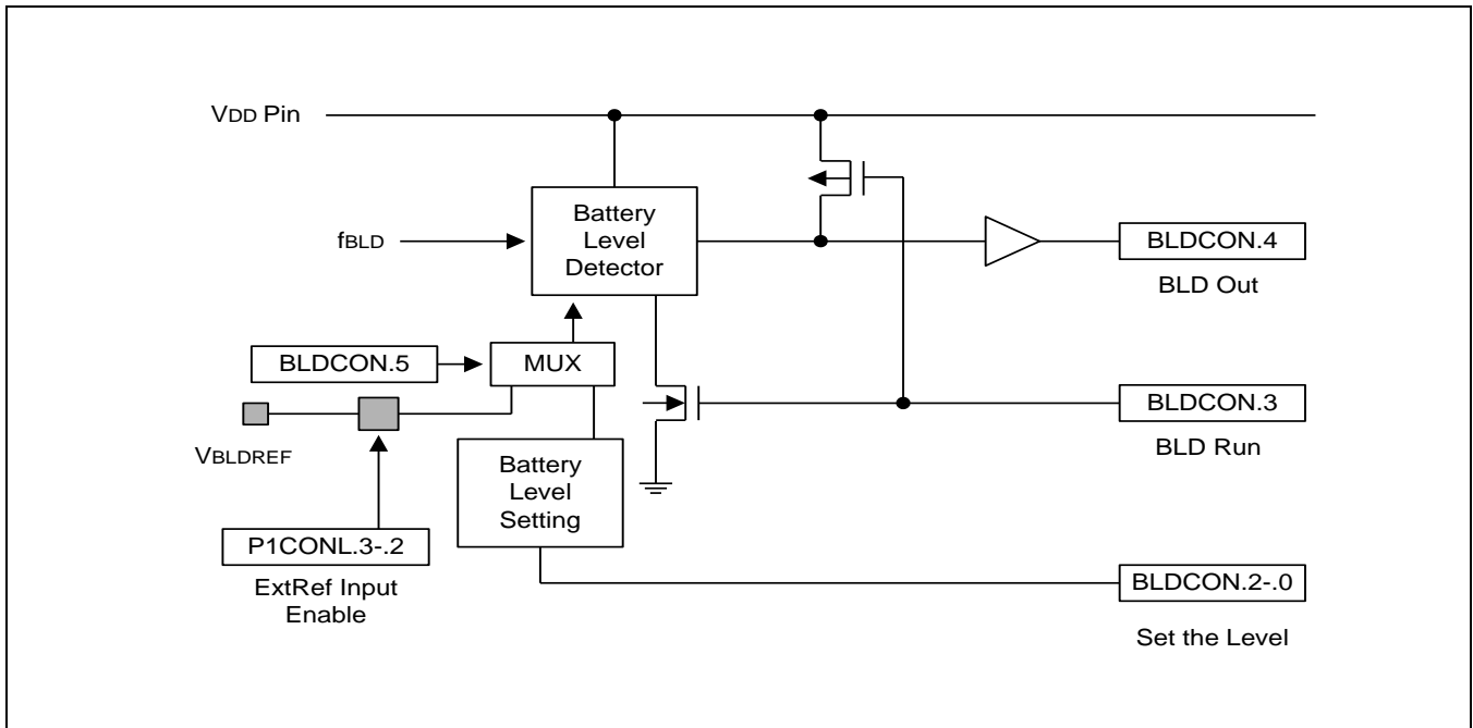
Figure 22-1 Block Diagram for Battery Level Detect
