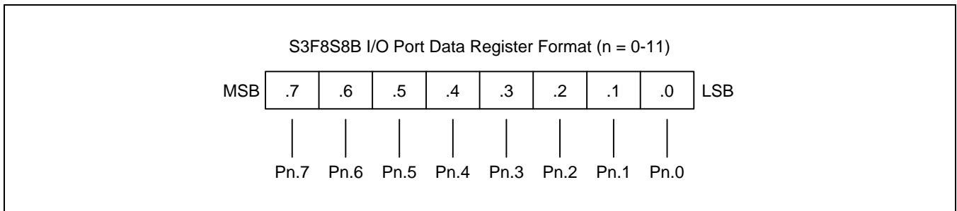
Figure 9-1 S3F8S8B I/O Port Data Register Format
