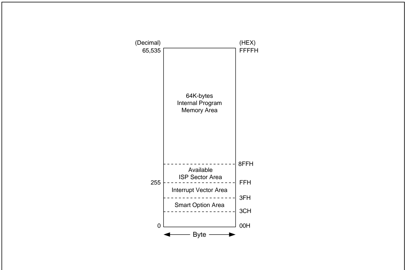
Figure 25-5 Program Memory Address Space
