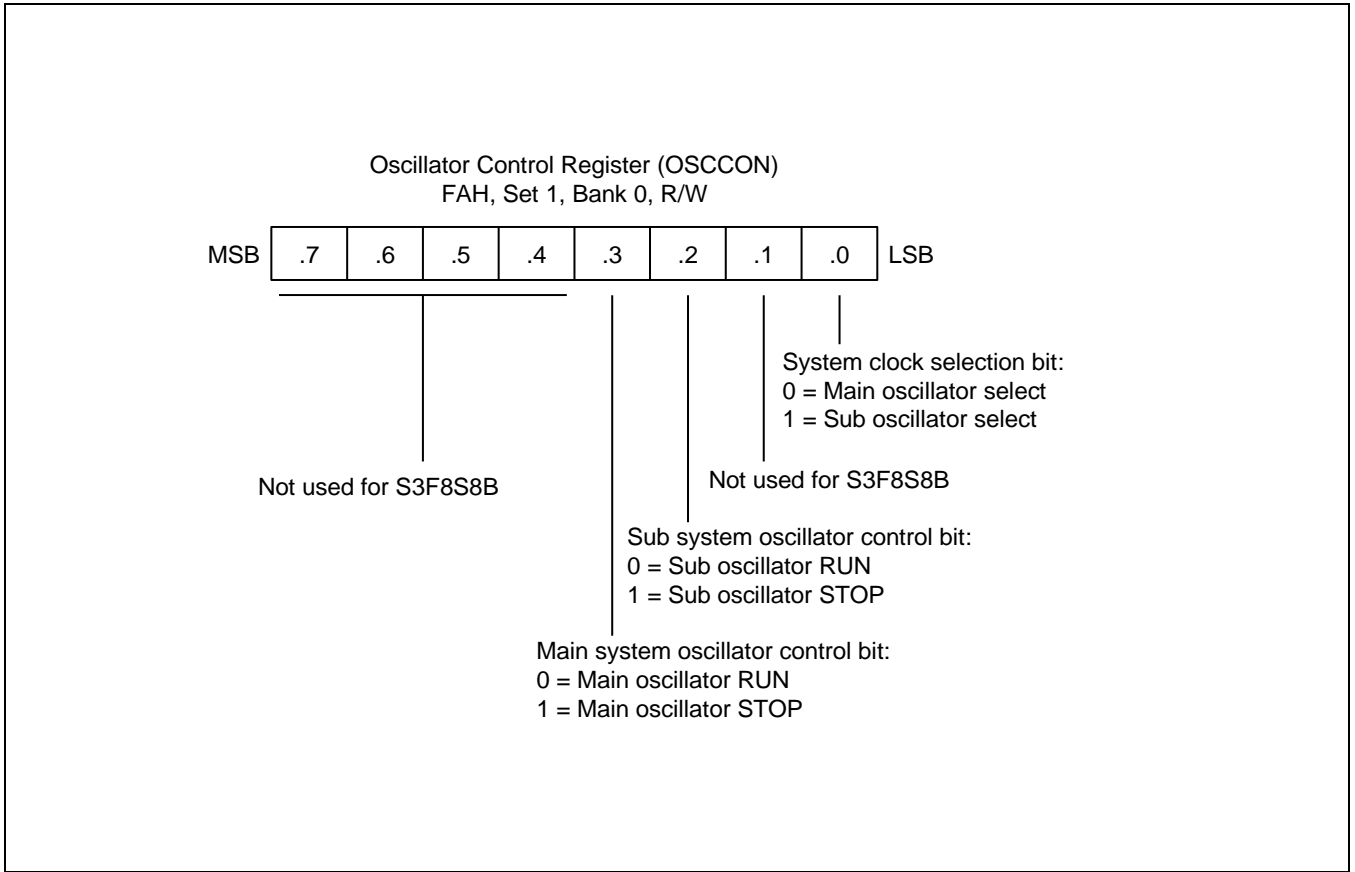
Figure 7-8 Oscillator Control Register (OSCCON)
