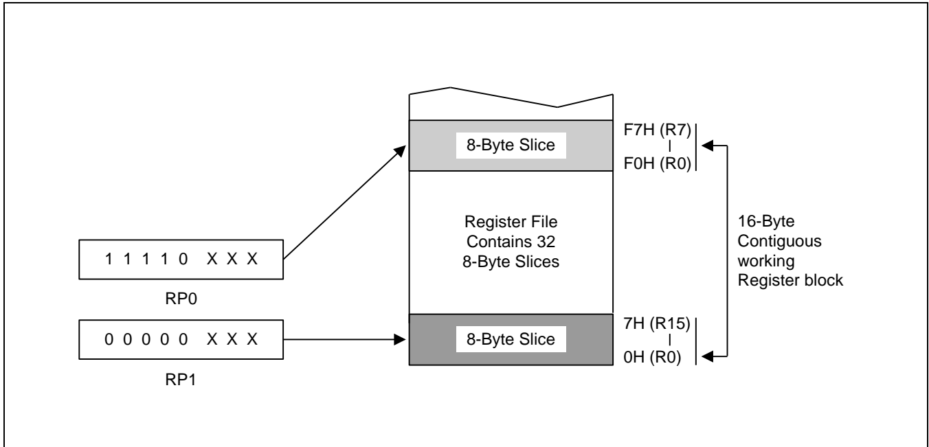
Figure 2-8 Non-Contiguous 16 Byte Working Register Block
