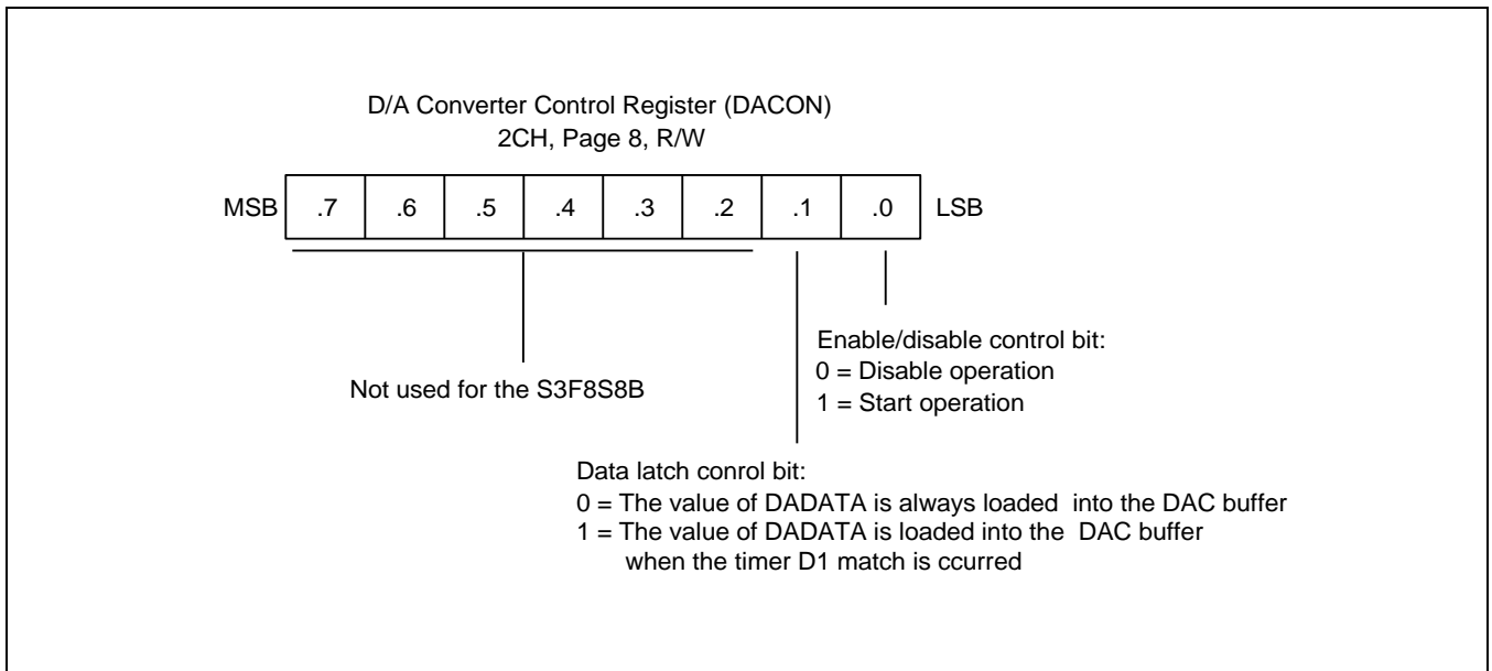
Figure 18-2 Digital to Analog Converter Control Register (DACON)
