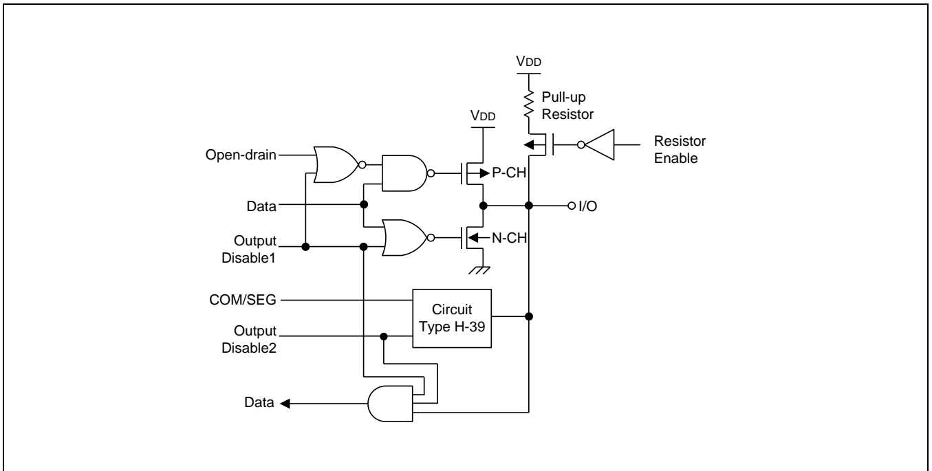
Figure 1-12 Pin Circuit Type H-42 (P1, P3, P6 - P11)
