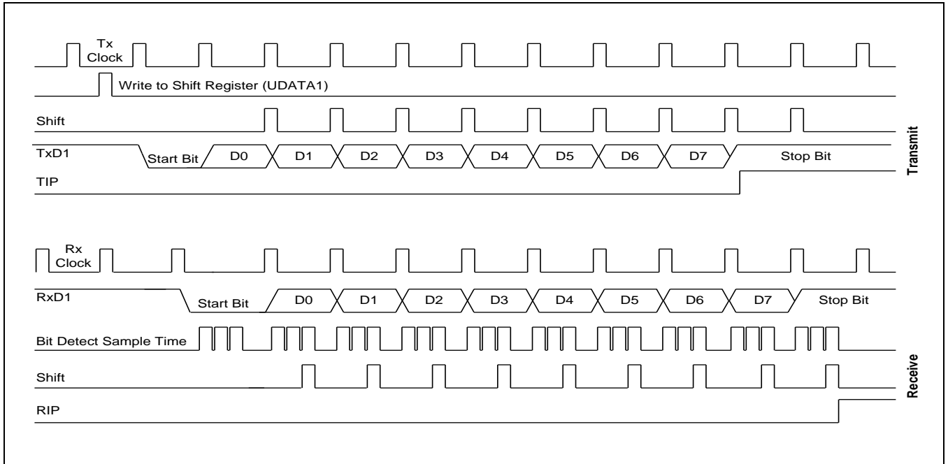
Figure 21-7 Timing Diagram for Serial Port Mode 1 Operation
