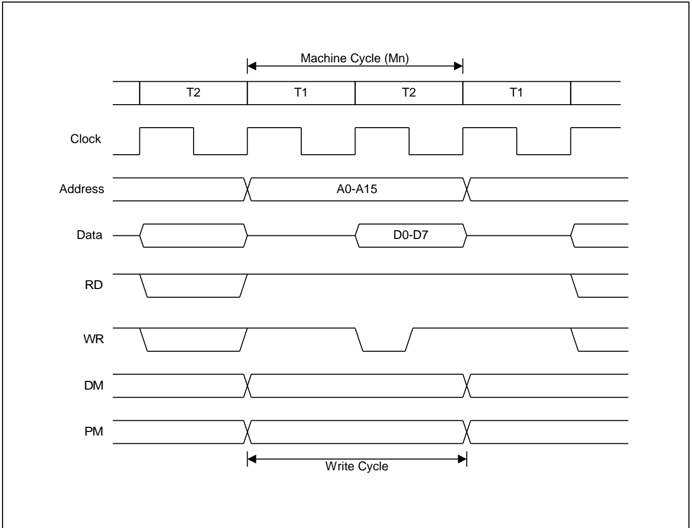
Figure 24-6 External Bus Write Cycle Timing Diagram (Address, and Data Separated)
