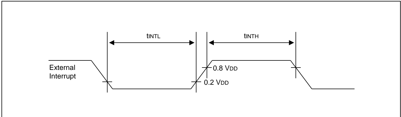
Figure 26-1 Input Timing for External Interrupts
