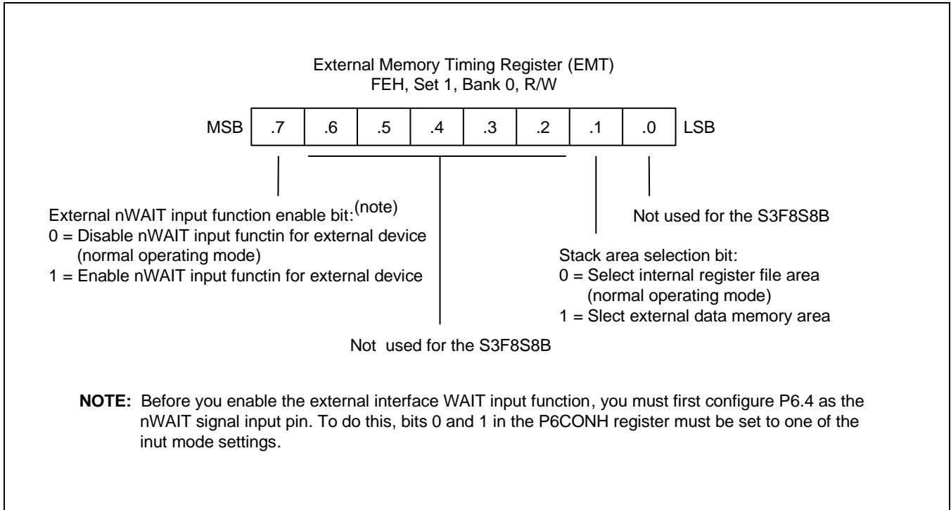
Figure 24-4 External Memory Timing Register (EMT)
