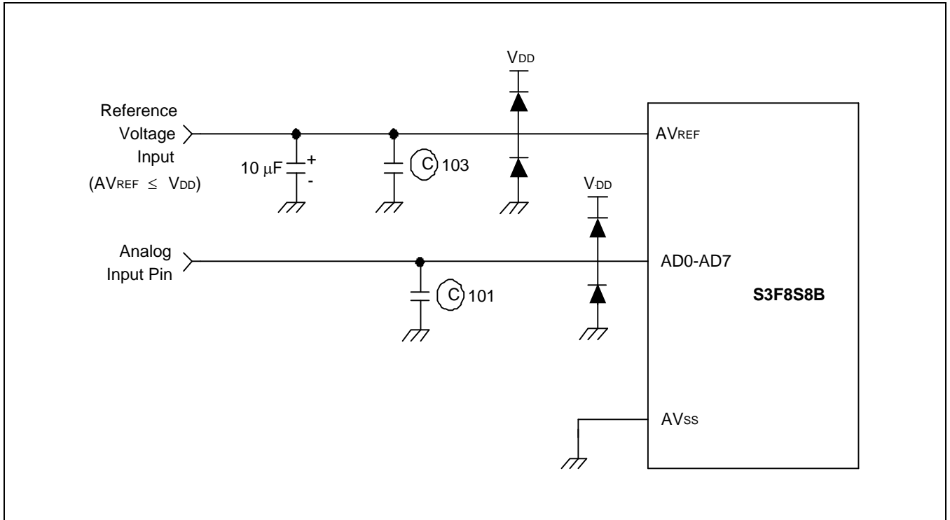
Figure 17-4 Recommended A/D Converter Circuit for Highest Absolute Accuracy
