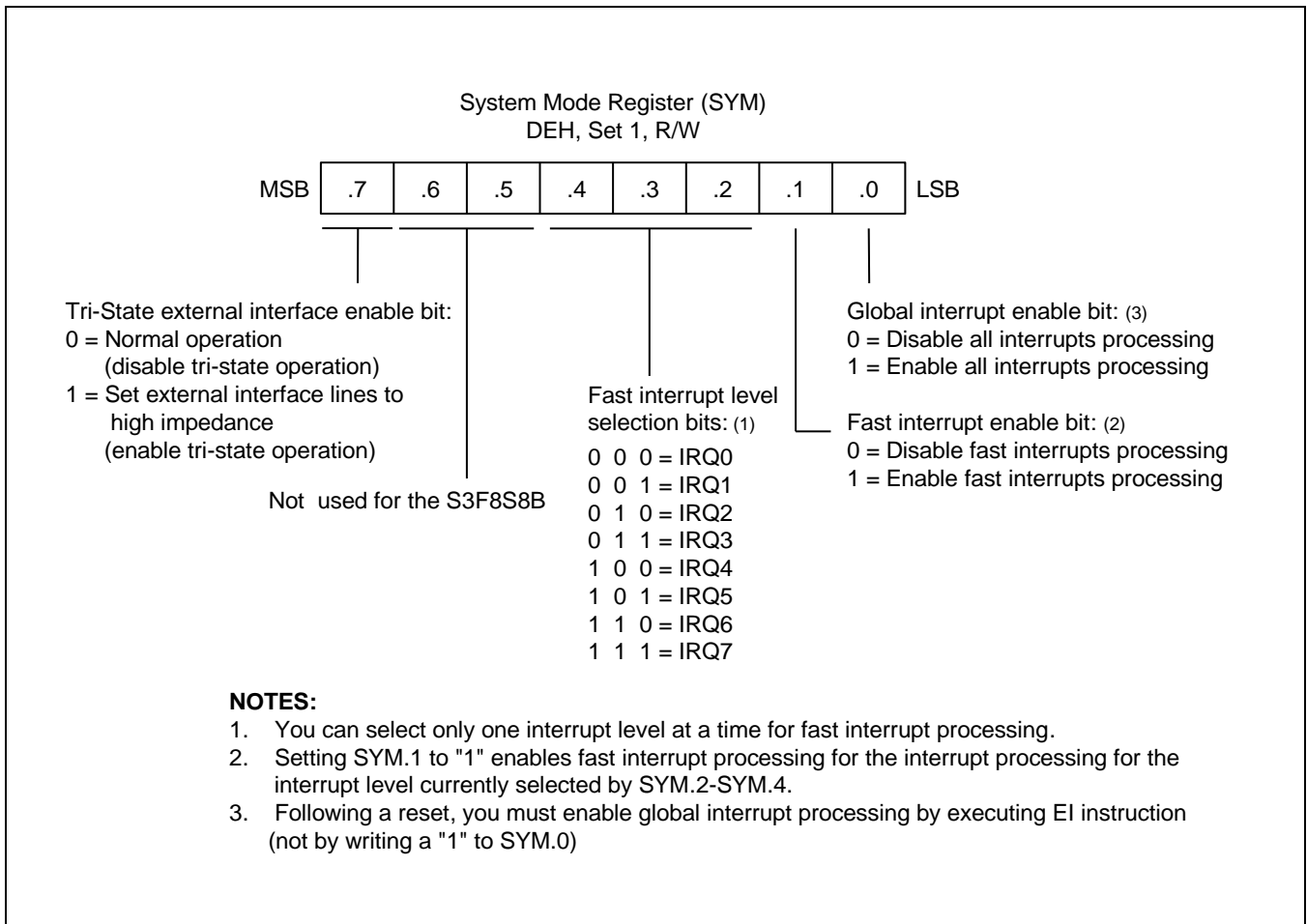
Figure 5-5 System Mode Register (SYM)
