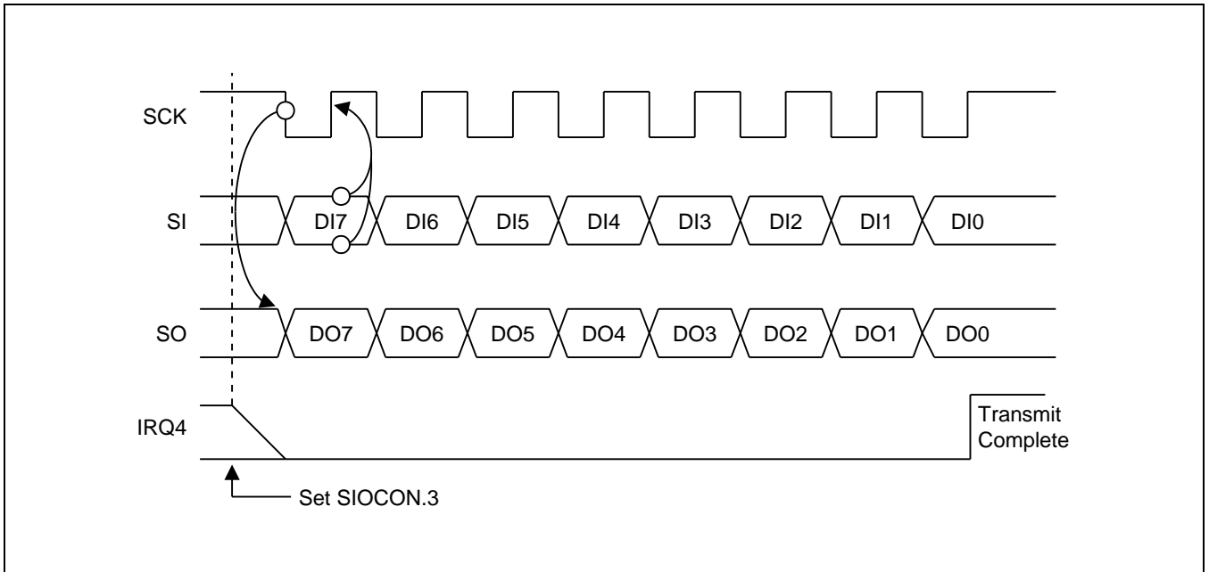
Figure 19-4 Serial I/O Timing in Transmit/Receive Mode (Tx at falling, SIOCON.4 = 0)
