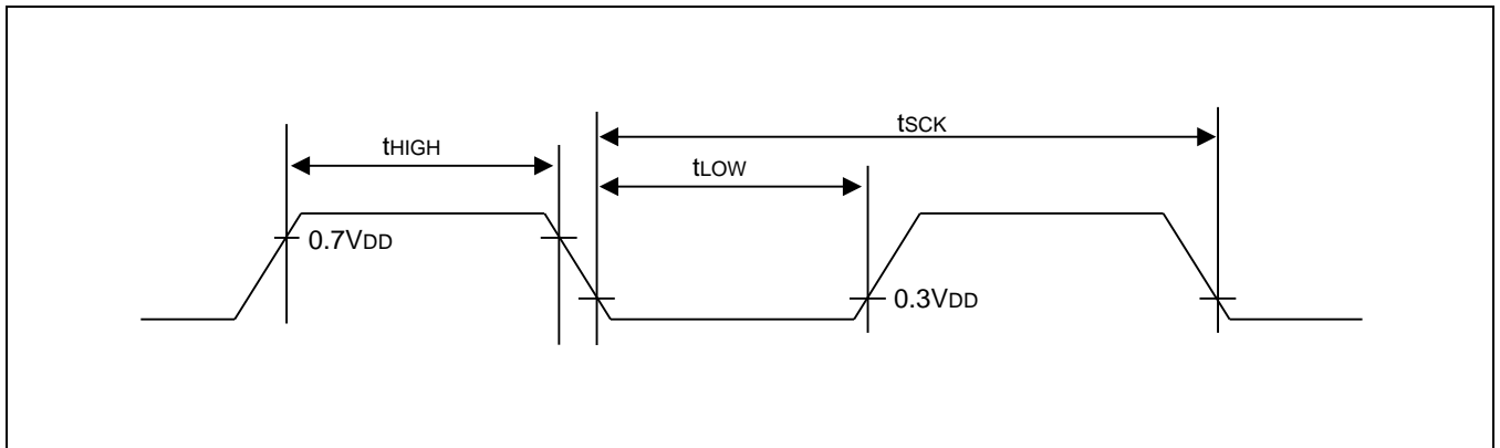
Figure 26-7 Waveform for UART Timing Characteristics
