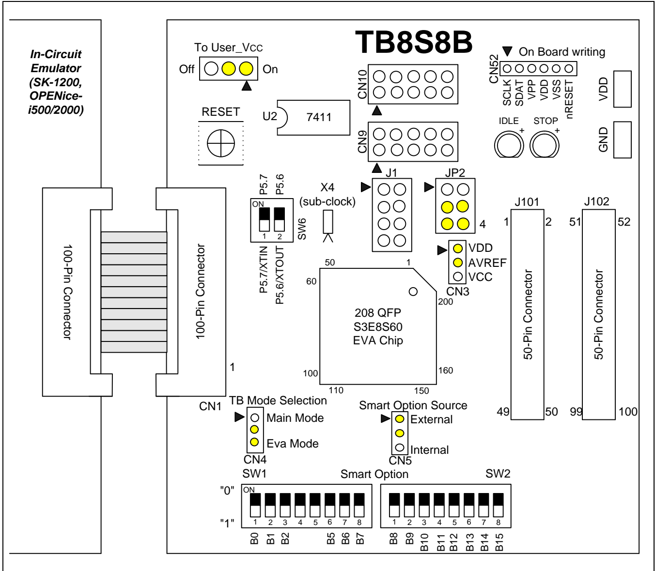
Figure 29-2 TB8S8B Target Board Configuration
