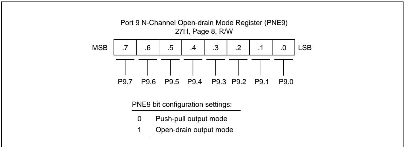
Figure 9-40 Port 9 N-Channel Open-drain Mode Register (PNE9)
