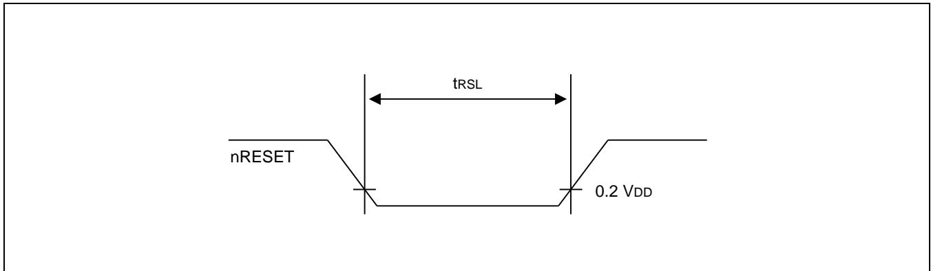
Figure 26-2 Input Timing for nRESET
