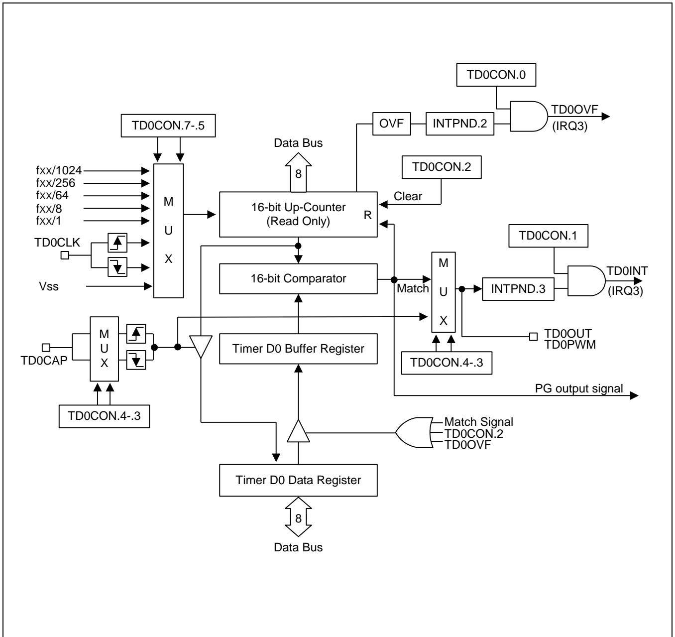
Figure 13-5 Timer D0 Functional Block Diagram
