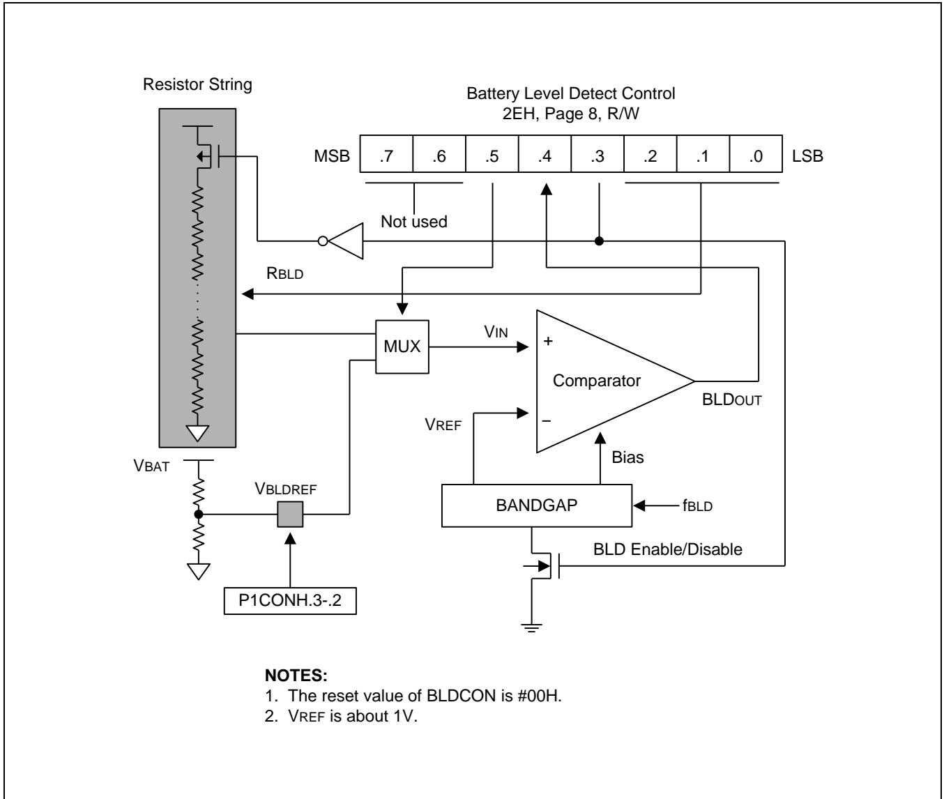
Figure 22-3 Battery Level Detector Circuit and Block Diagram
