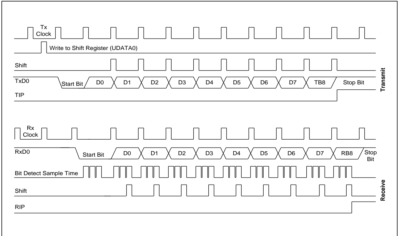
Figure 20-9 Timing Diagram for Serial Port Mode 3 Operation
