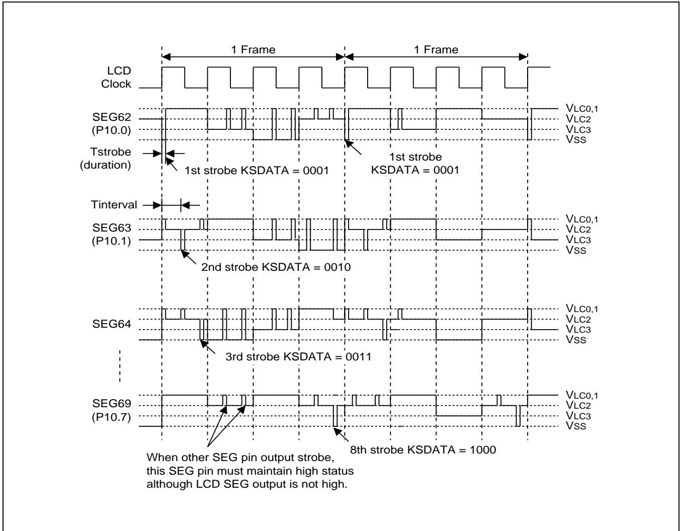
Figure 16-4 Example of Key Strobe Mode with 1/4 Duty SEG Output
