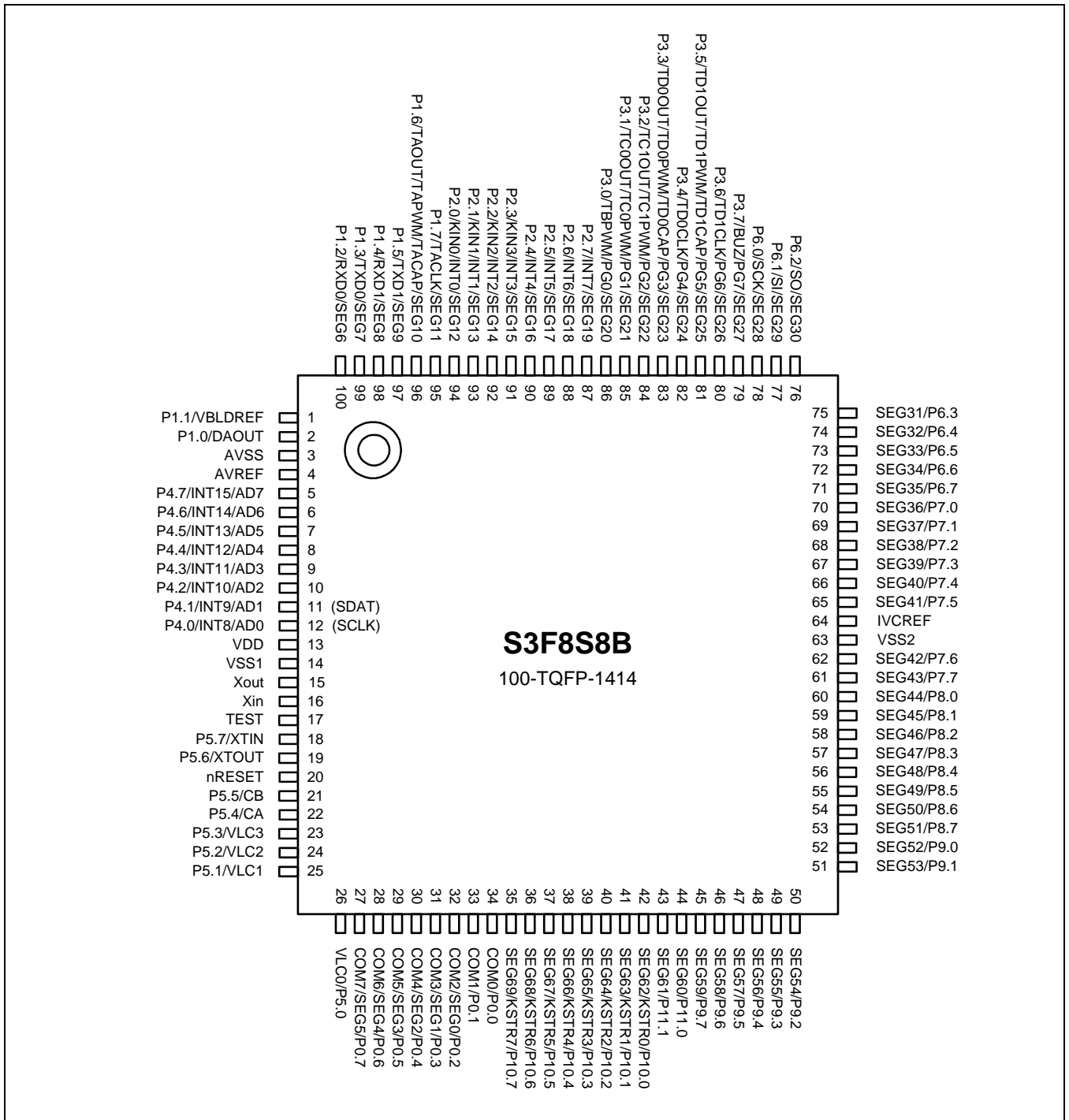
Figure 1-3 S3F8S8B Pin Assignments (100-TQFP-1414)
