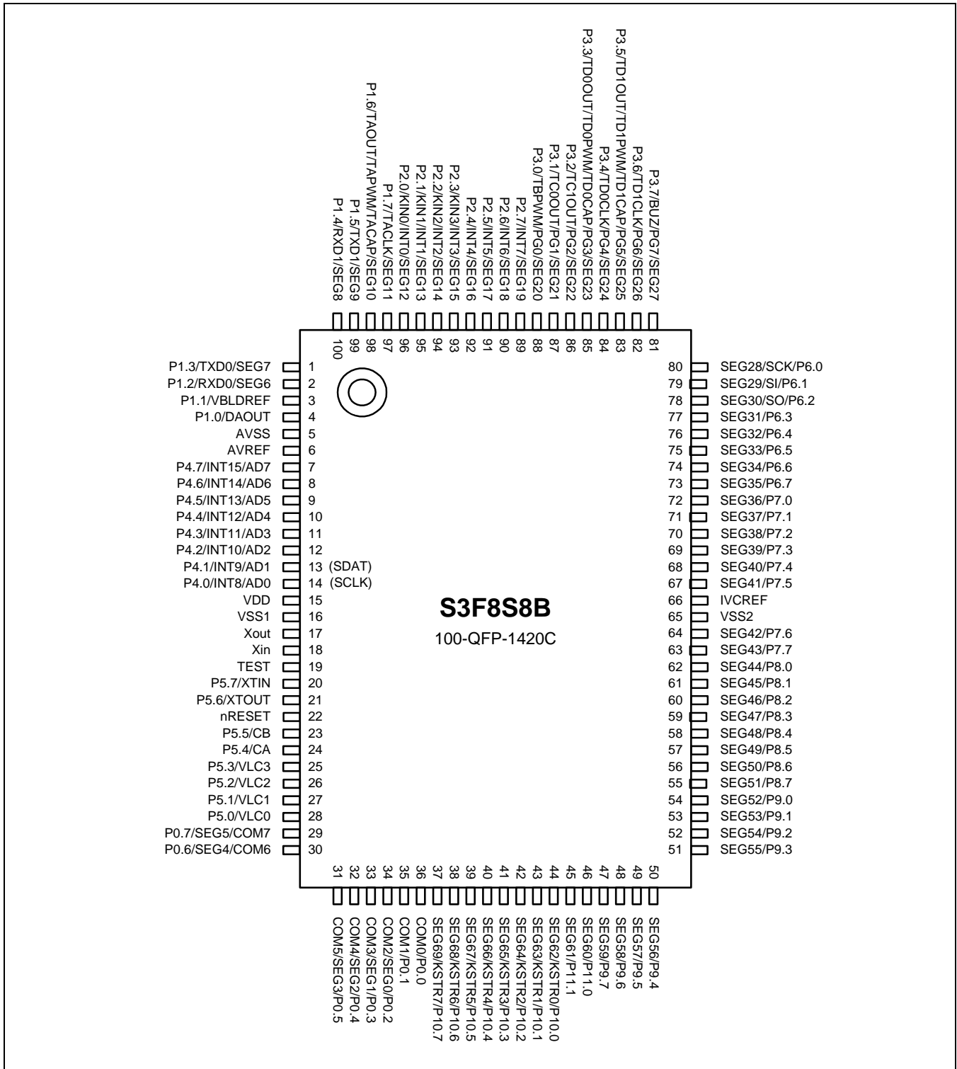
Figure 1-2 S3F8S8B Pin Assignments (100-QFP-1420C)
