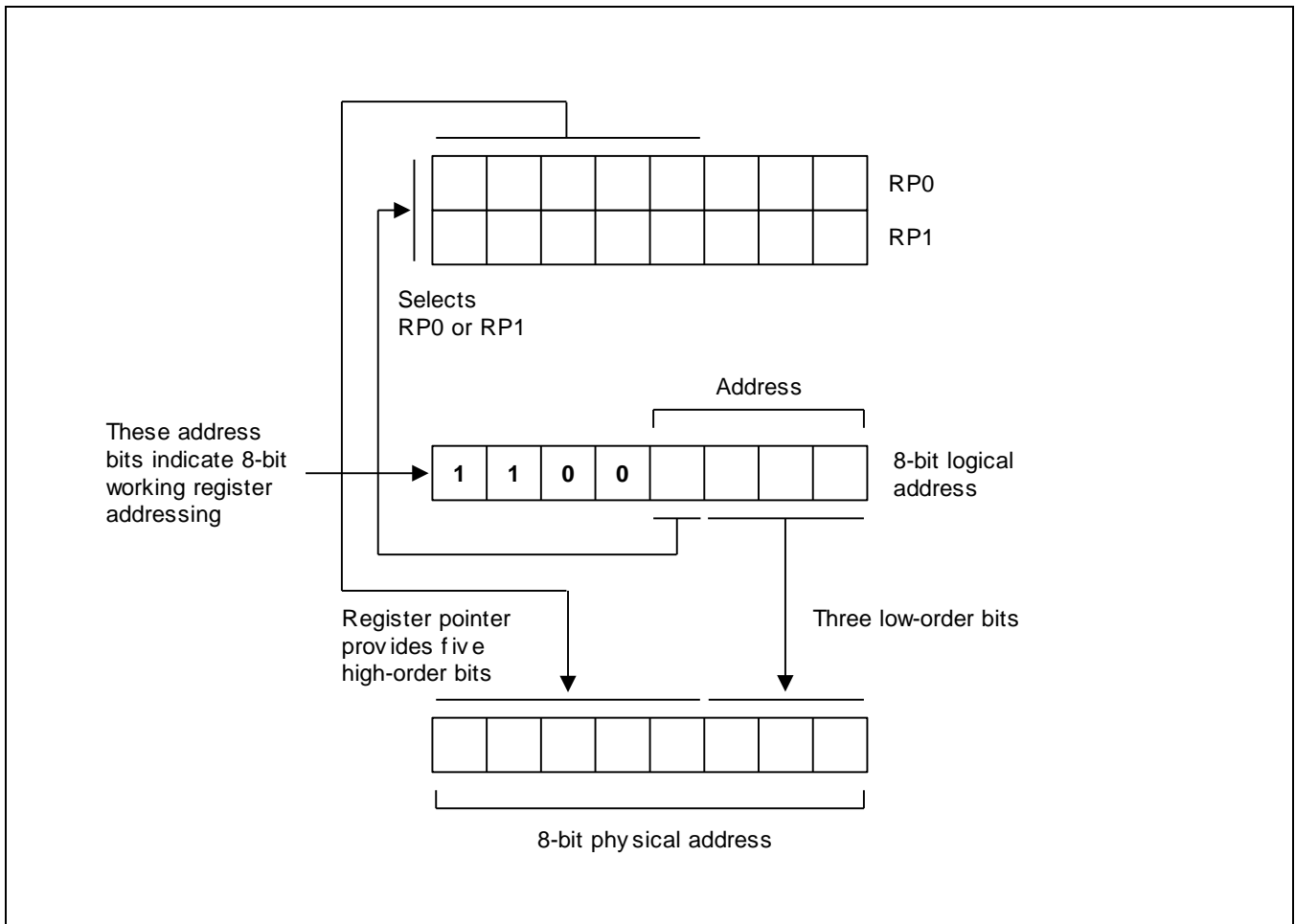
Figure 2-14 8-Bit Working Register Addressing
