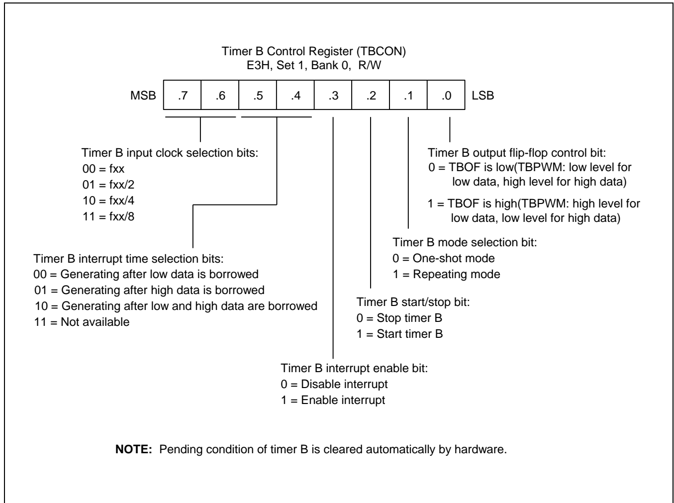
Figure 11-6 Timer B Control Register
