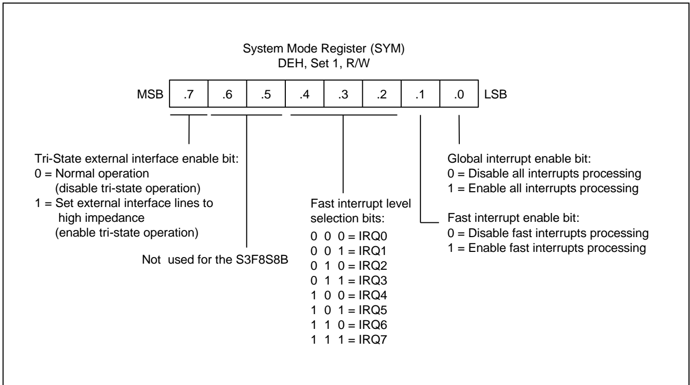
Figure 24-3 System Mode Register (SYM)
