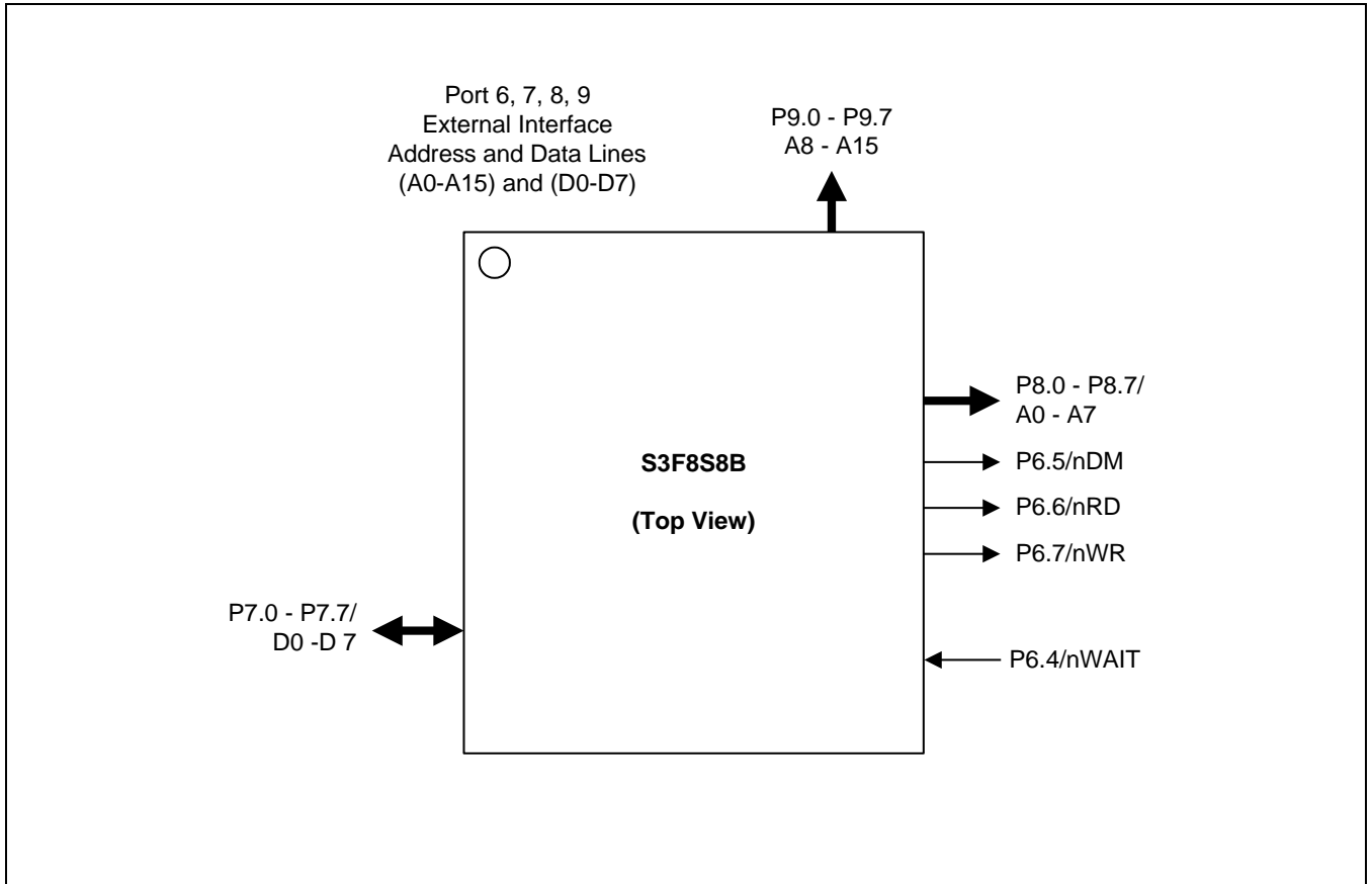
Figure 24-1 S3F8S8B External Memory Interface Function Diagram
