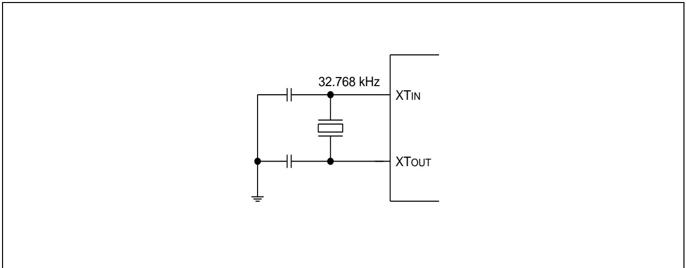
Figure 7-4 Crystal Oscillator (fxt)
