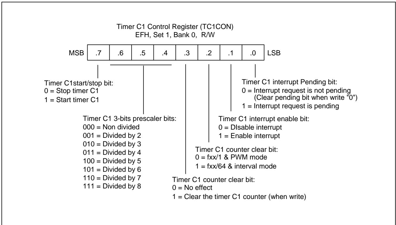
Figure 12-3 Timer C1 Control Register (TC1CON)
