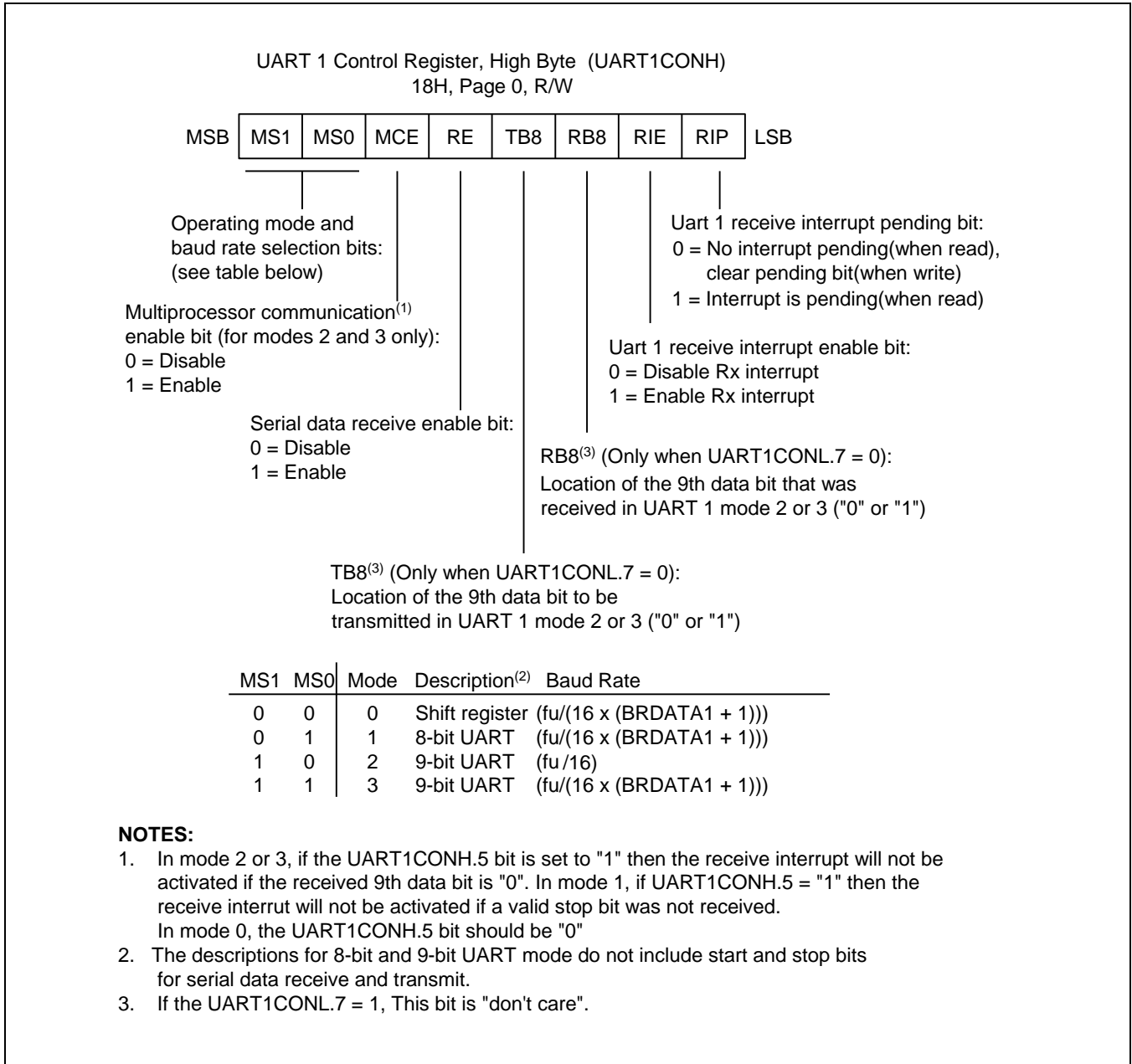
Figure 21-1 UART 1 High Byte Control Register (UART1CONH)
