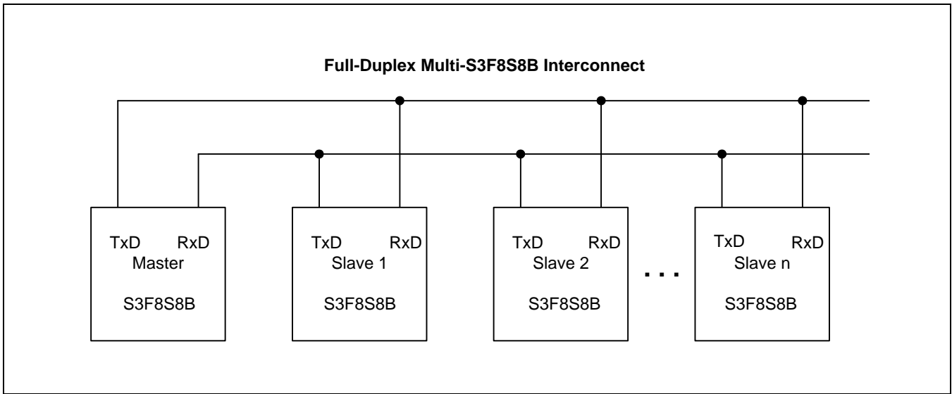
Figure 21-10 Connection Example for Multiprocessor Serial Data Communications
