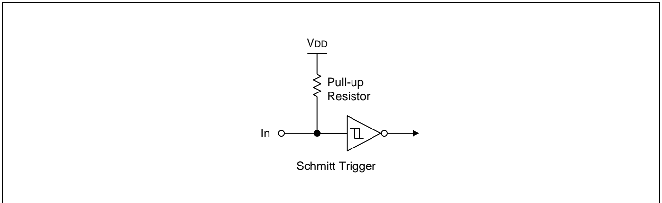
Figure 1-4 Pin Circuit Type B
