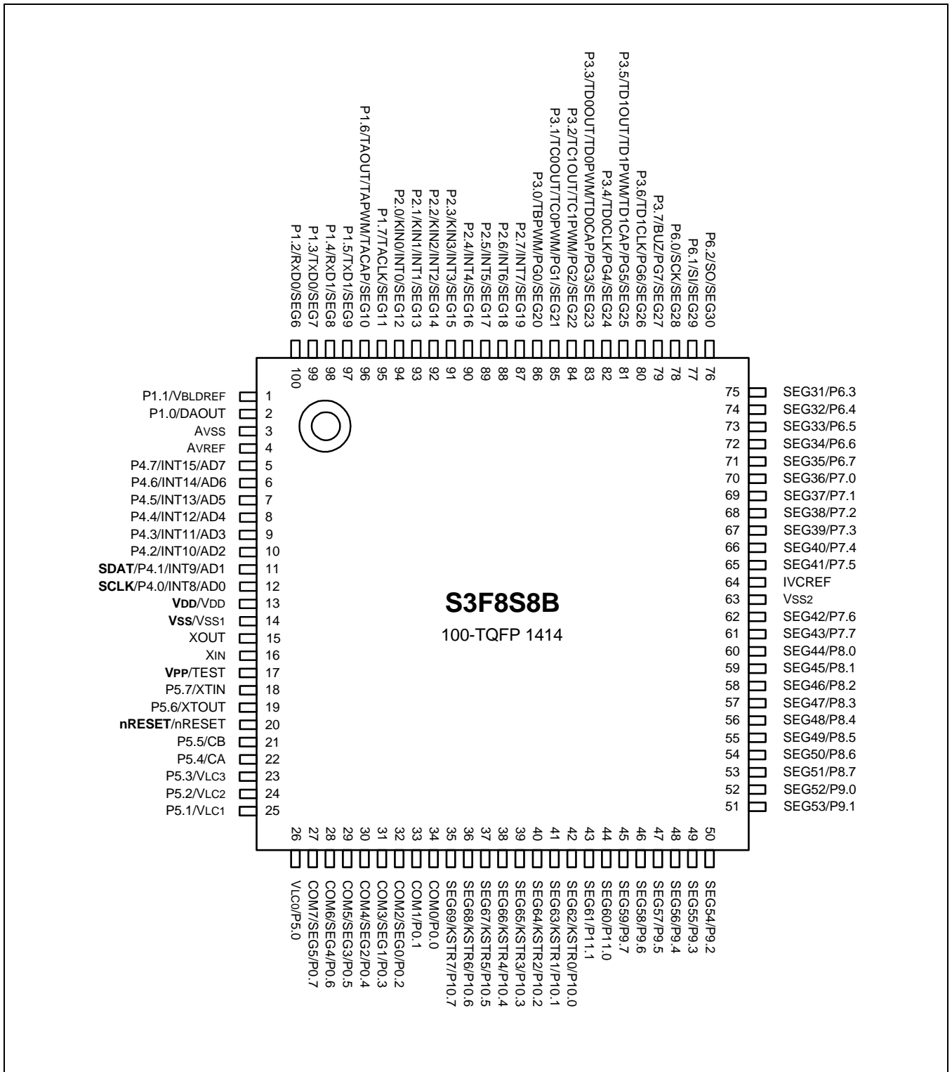
Figure 28-2 S3F8S8B Pin Assignments (100-TQFP-1414)
