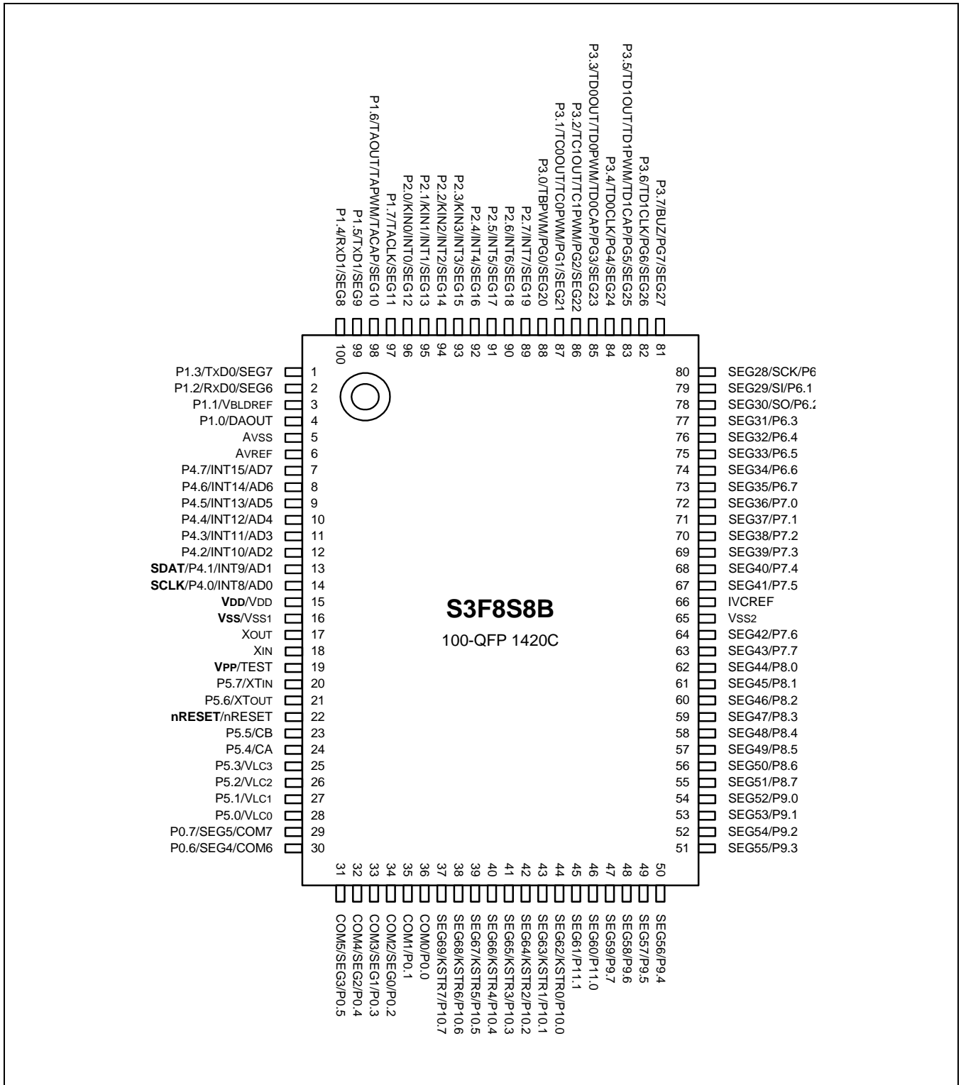
Figure 28-1 S3F8S8B Pin Assignments (100-QFP-1420C)
