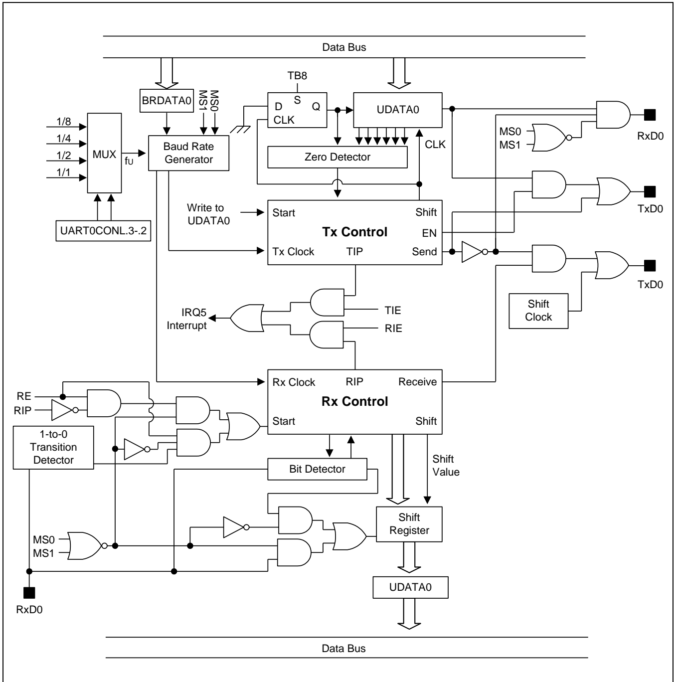
Figure 20-5 UART 0 Functional Block Diagram
