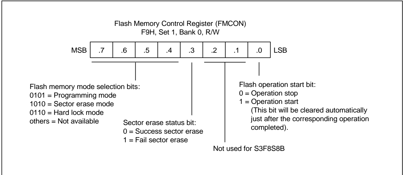
Figure 25-1 Flash Memory Control Register (FMCON)
