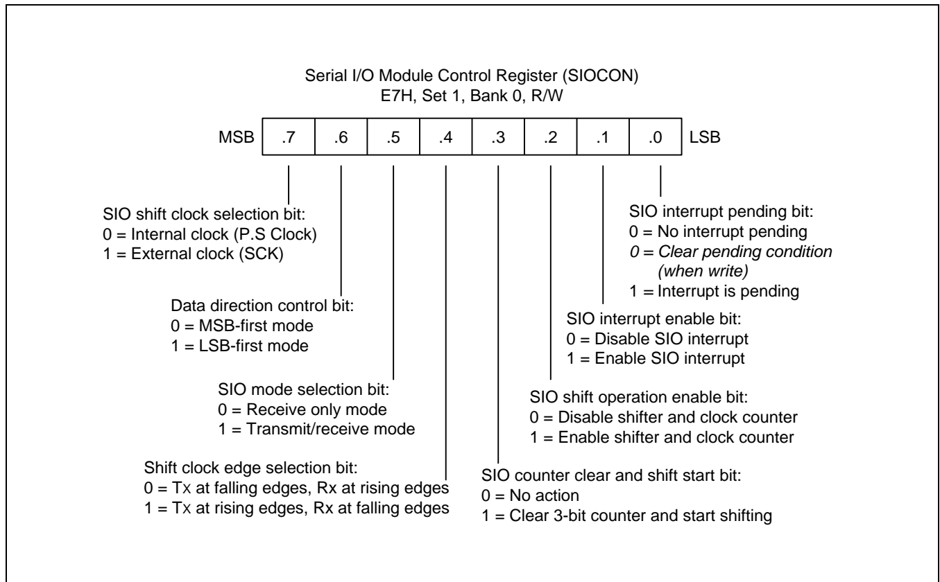
Figure 19-1 Serial I/O Module Control Registers (SIOCON)
