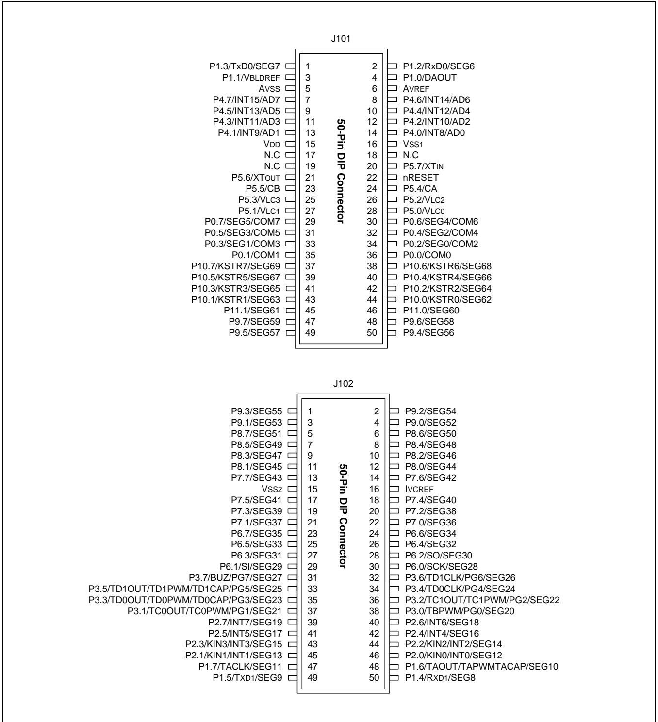
Figure 29-3 50-Pin Connectors (J101, J102) for TB8S8B
