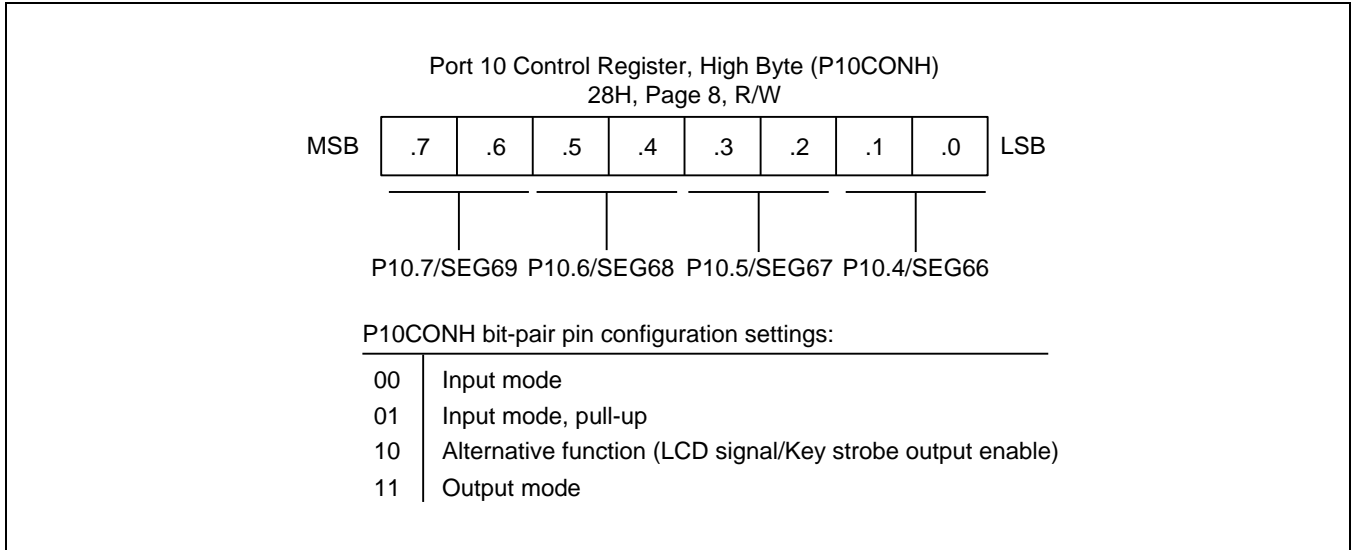
Figure 9-41 Port 10 High-byte Control Register (P10CONH)
