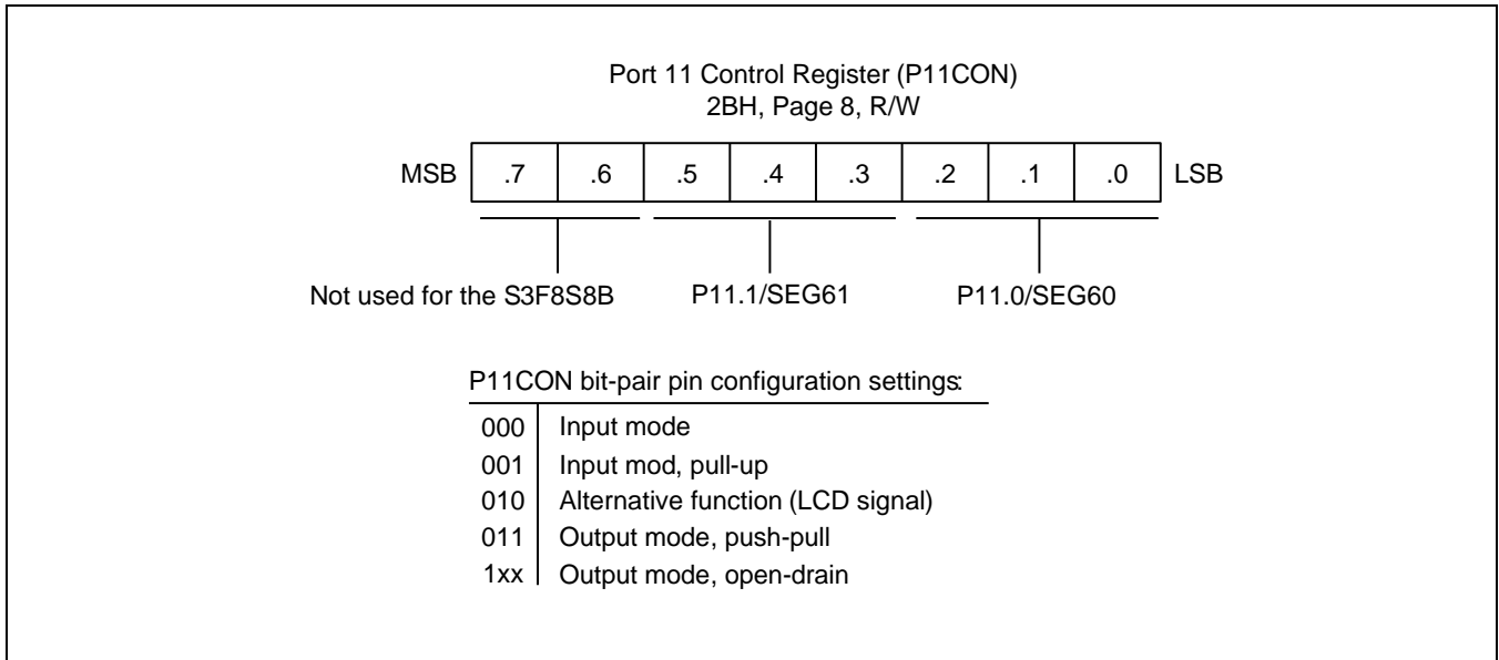
Figure 9-44 Port 11 Control Register (P11CON)
