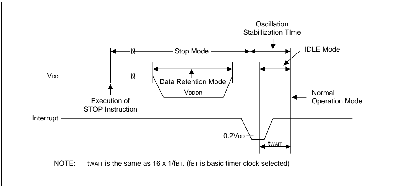
Figure 26-4 Stop Mode Release Timing Initiated by Interrupts
