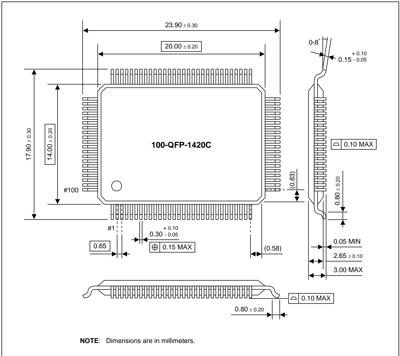
Figure 27-1 Package Dimensions (100-QFP-1420C)
