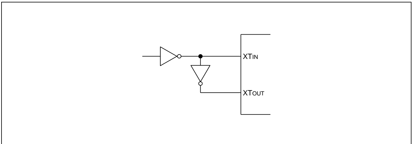
Figure 7-5 External Oscillator (fxt)
