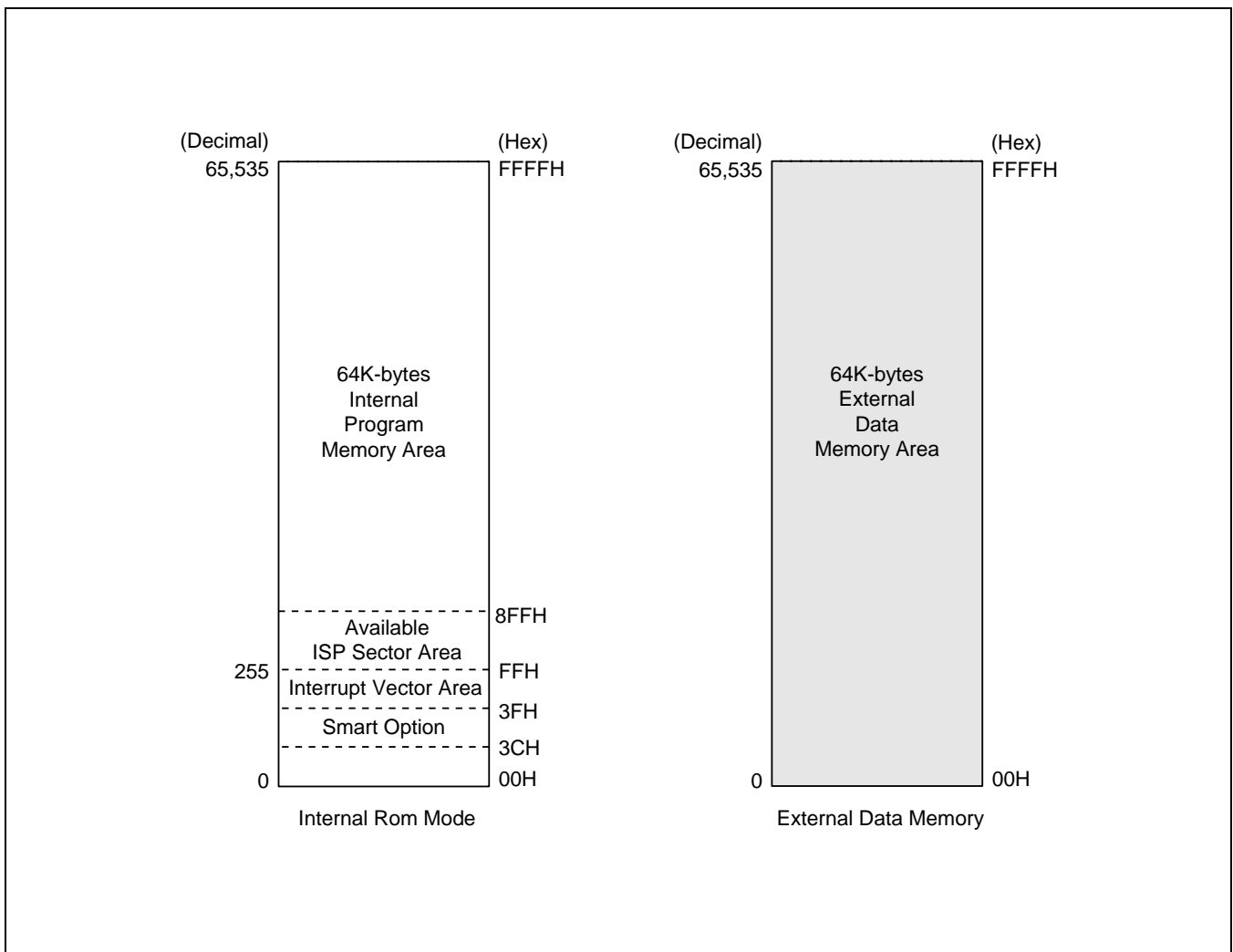
Figure 24-2 Internal Program and External Data Memory Options
