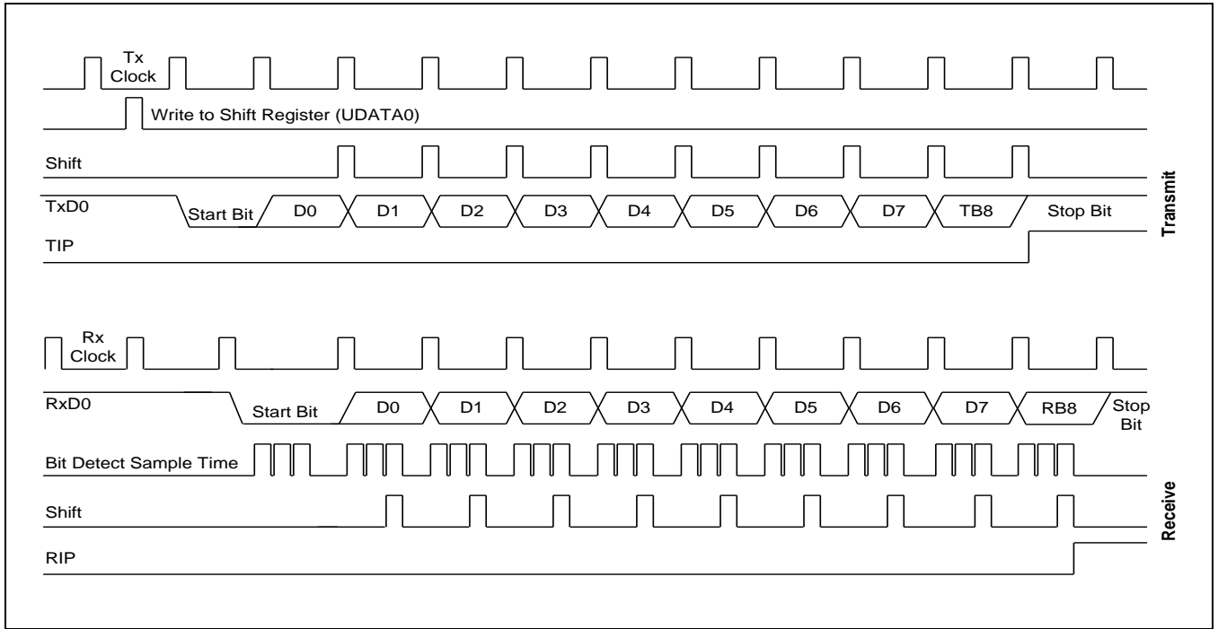
Figure 20-8 Timing Diagram for Serial Port Mode 2 Operation
