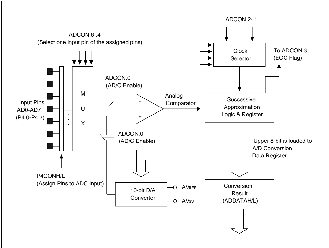
Figure 17-3 A/D Converter Functional Block Diagram
