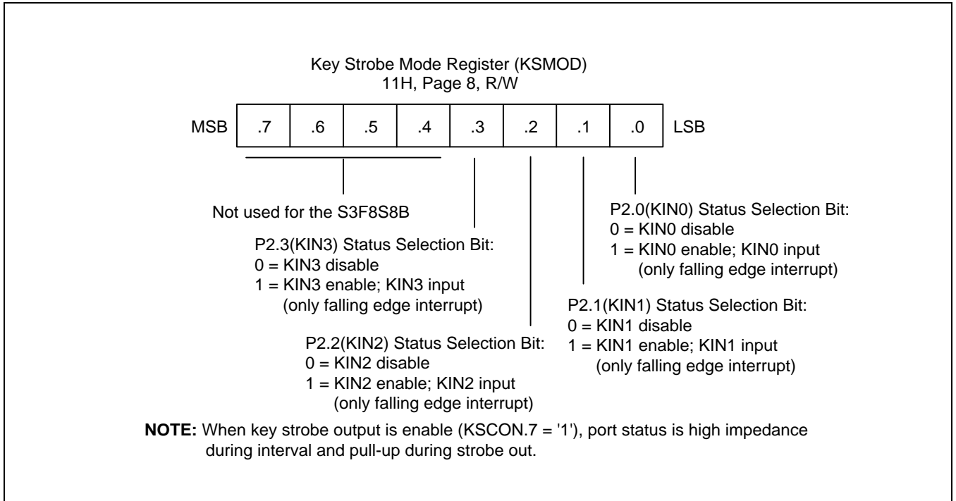
Figure 16-2 Key Strobe Mode Register (KSMOD)
