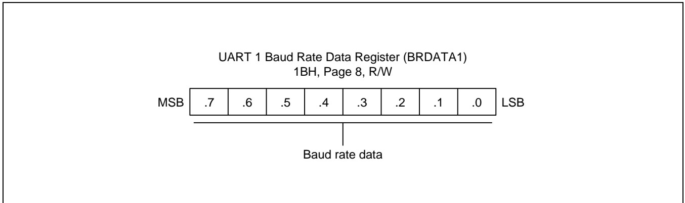
Figure 21-4 UART 1 Baud Rate Data Register (BRDATA1)
