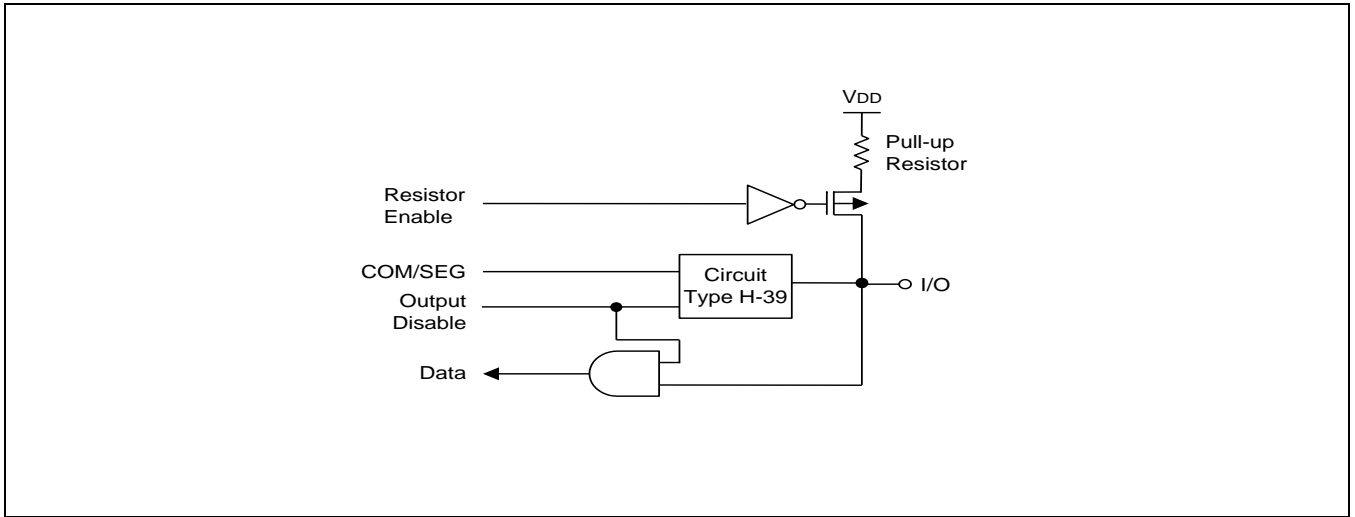
Figure 1-11 Pin Circuit Type H-44 (P0)
