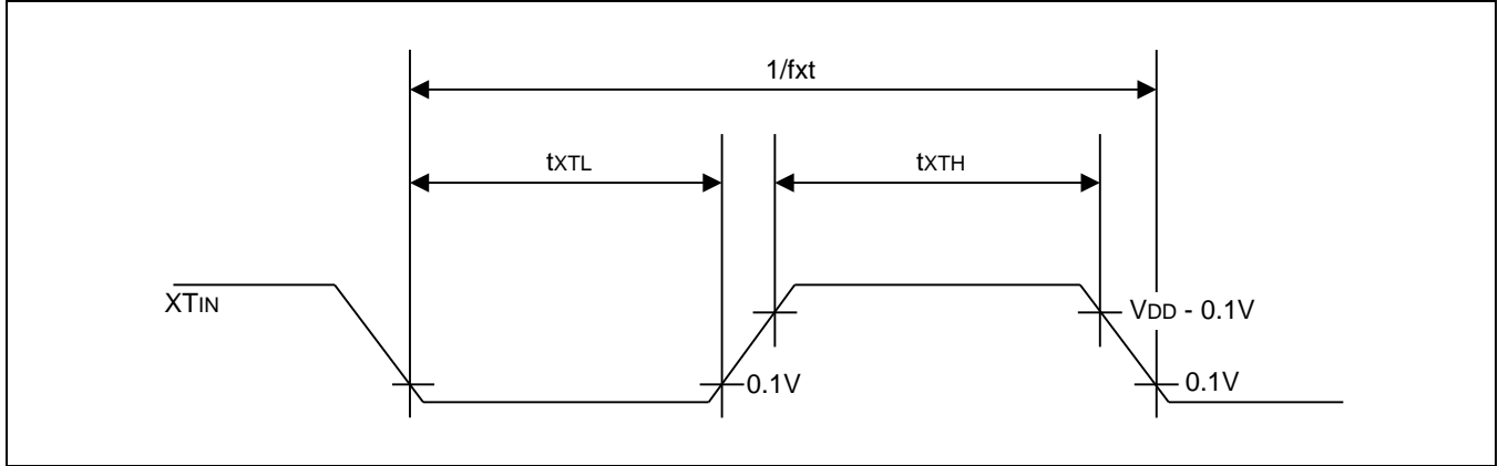
Figure 26-10 Clock Timing Measurement at XT_{IN}
