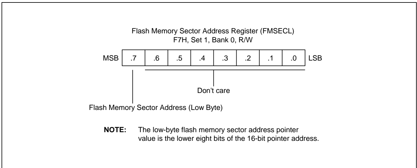
Figure 25-4 Flash Memory Sector Address Register Low Byte (FMSECL)
