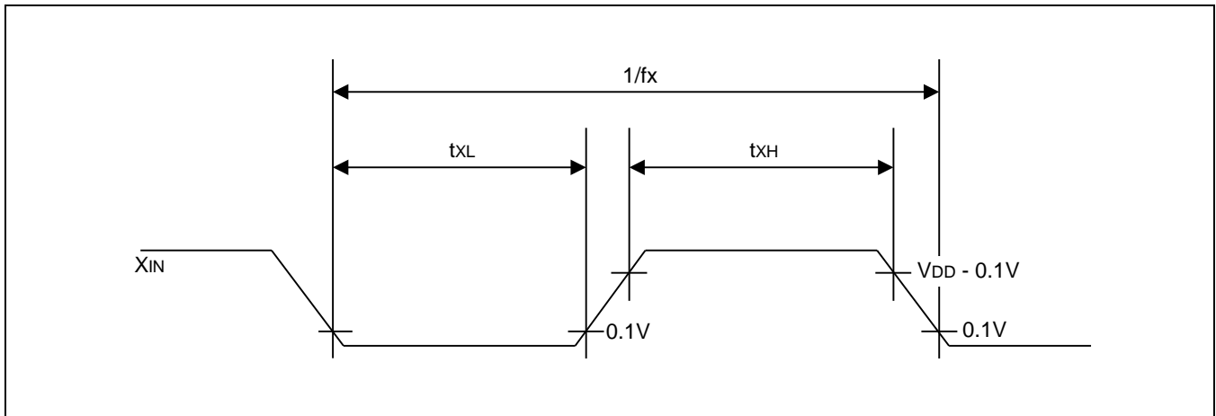
Figure 26-9 Clock Timing Measurement at X_{IN}
