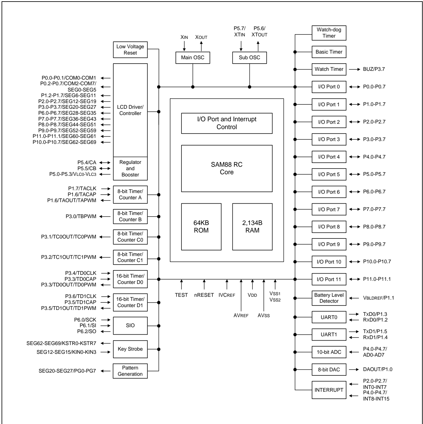
Figure 1-1 Block Diagram
