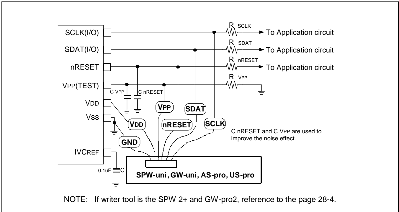
Figure 28-4 PCB Design Guide for on Board Programming
