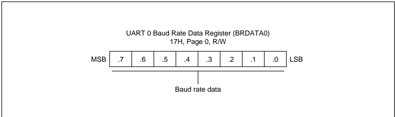
Figure 20-4 UART 0 Baud Rate Data Register (BRDATA0)
