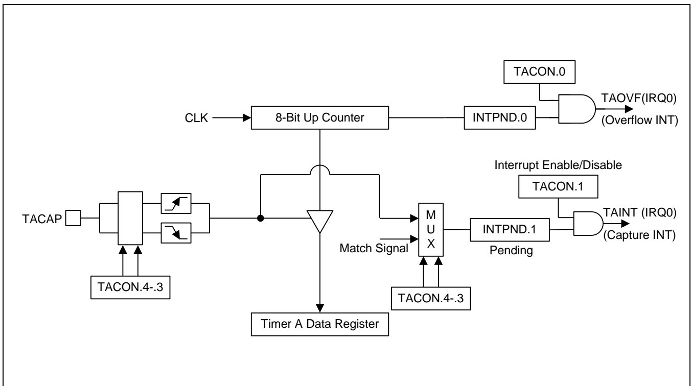
Figure 11-4 Simplified Timer A Function Diagram: Capture Mode
