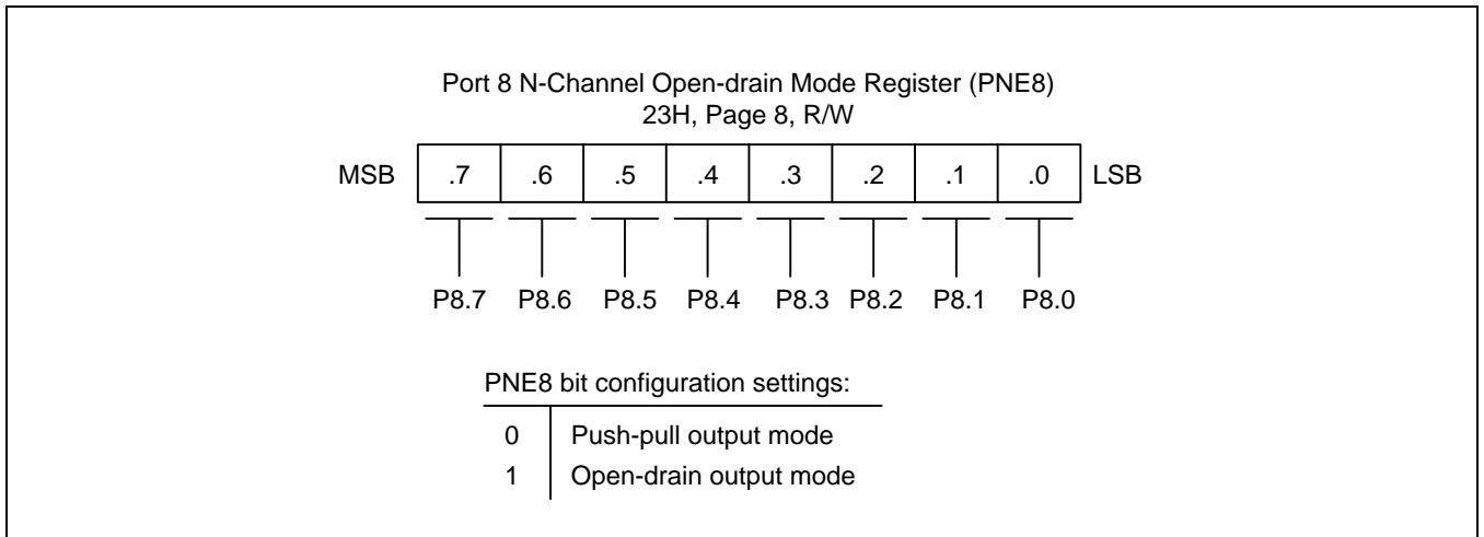
Figure 9-36 Port 8 N-Channel Open-drain Mode Register (PNE8)
