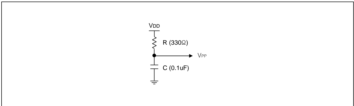
Figure 28-3 RC Delay Circuit
