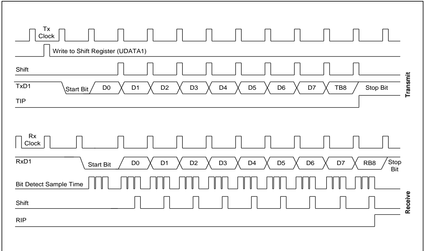
Figure 21-9 Timing Diagram for Serial Port Mode 3 Operation
