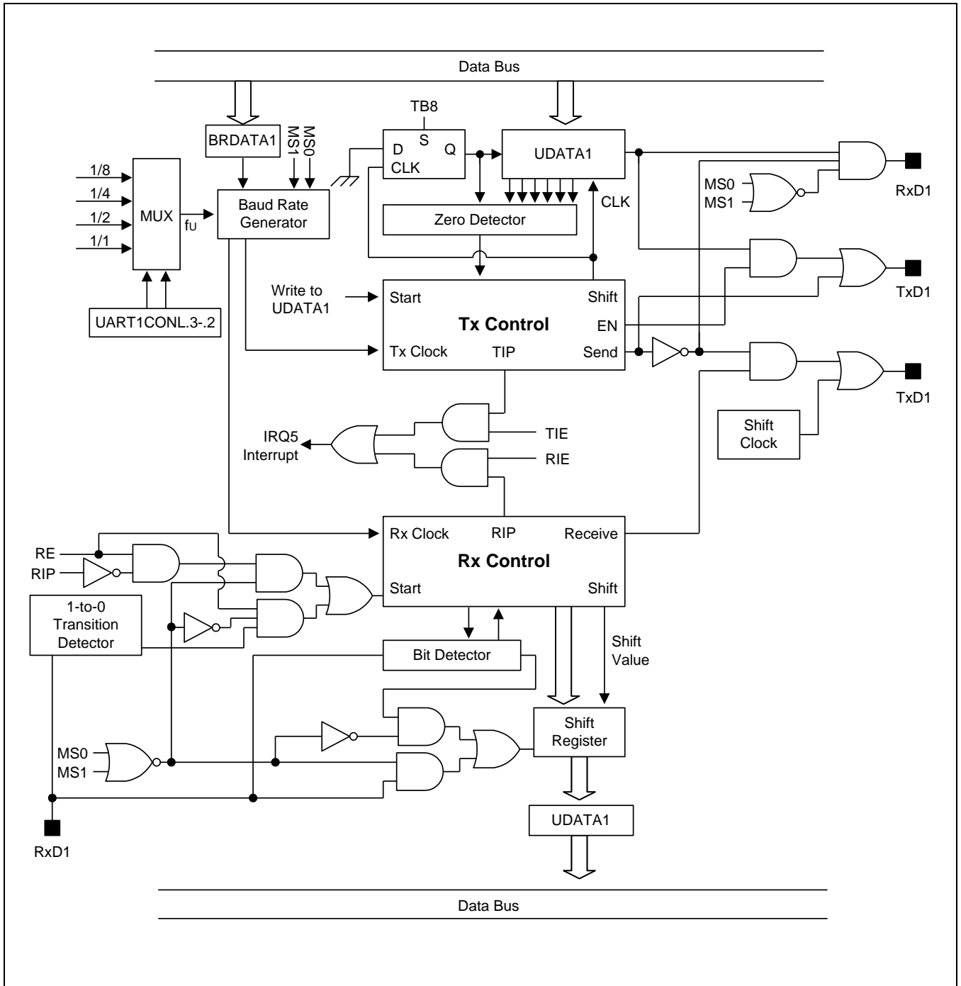
Figure 21-5 UART 1 Functional Block Diagram
