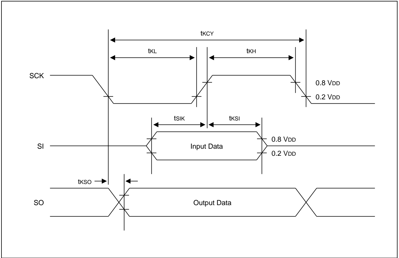
Figure 26-6 Serial Data Transfer Timing
