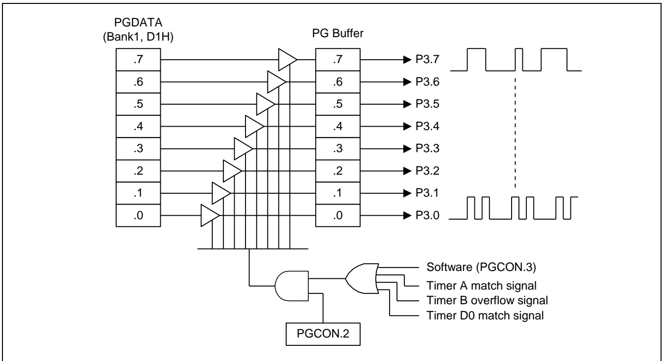
Figure 23-3 Pattern Generation Circuit Diagram
