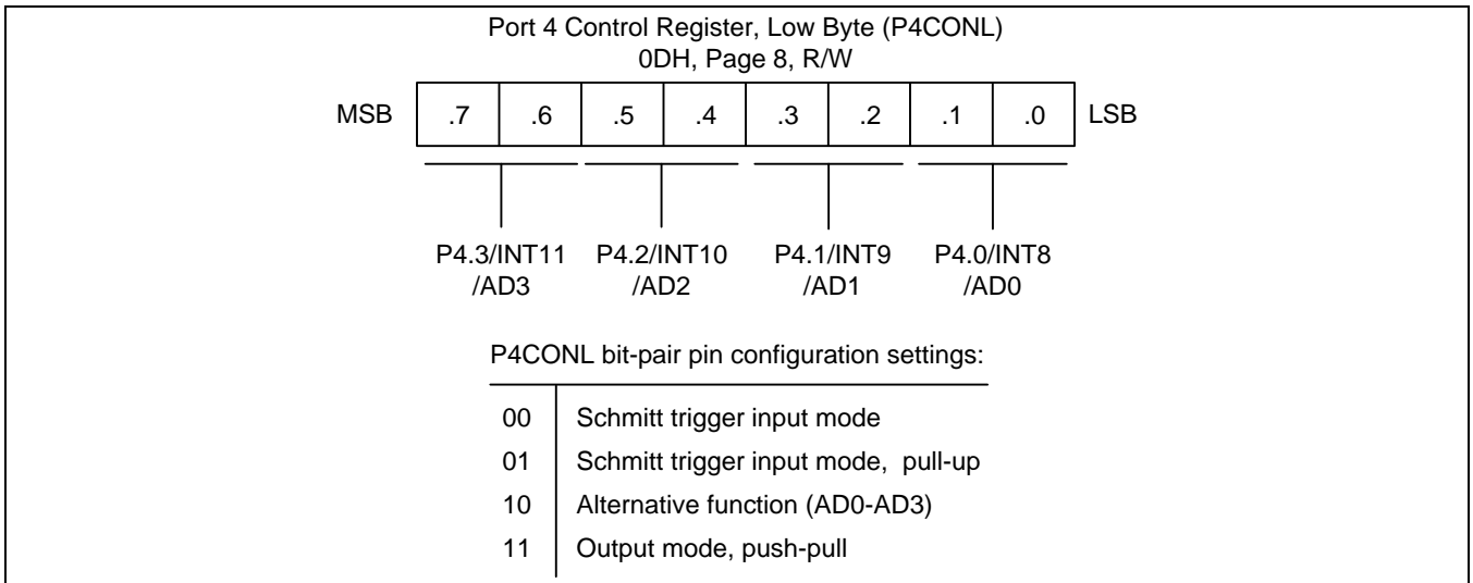
Figure 9-19 Port 4 Low-Byte Control Register (P4CONL)
