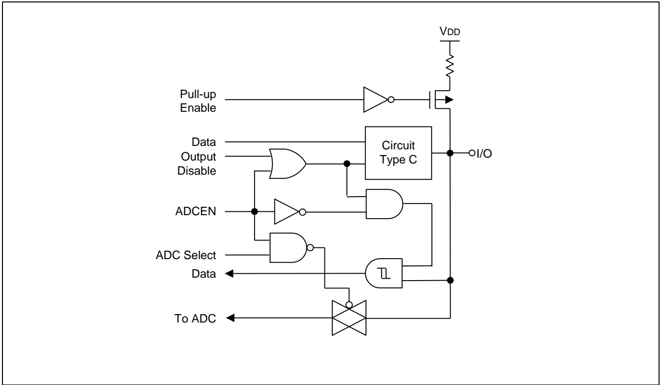
Figure 1-7 Pin Circuit Type F-16 (P4)
