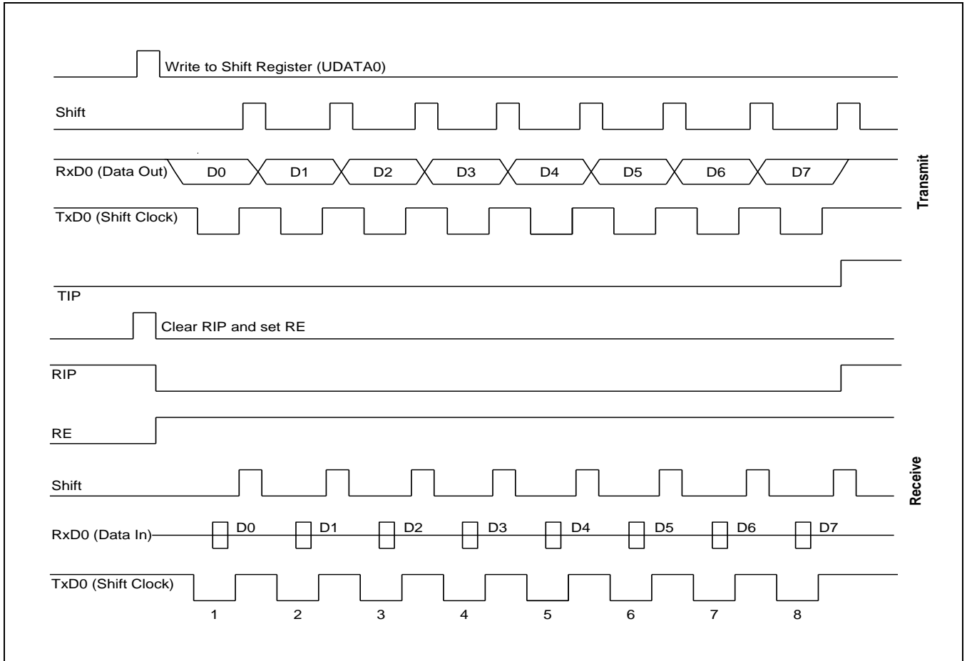
Figure 20-6 Timing Diagram for Serial Port Mode 0 Operation
