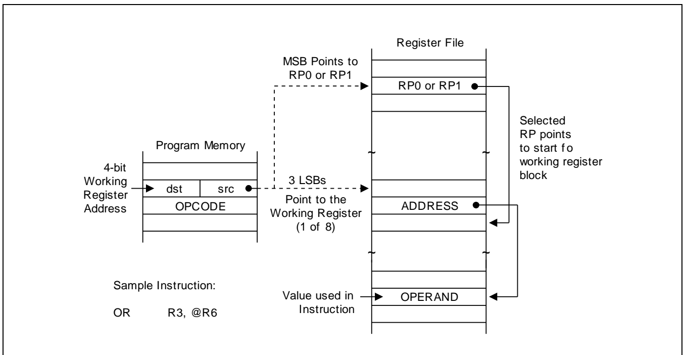
Figure 3-5 Indirect Working Register Addressing to Register File
