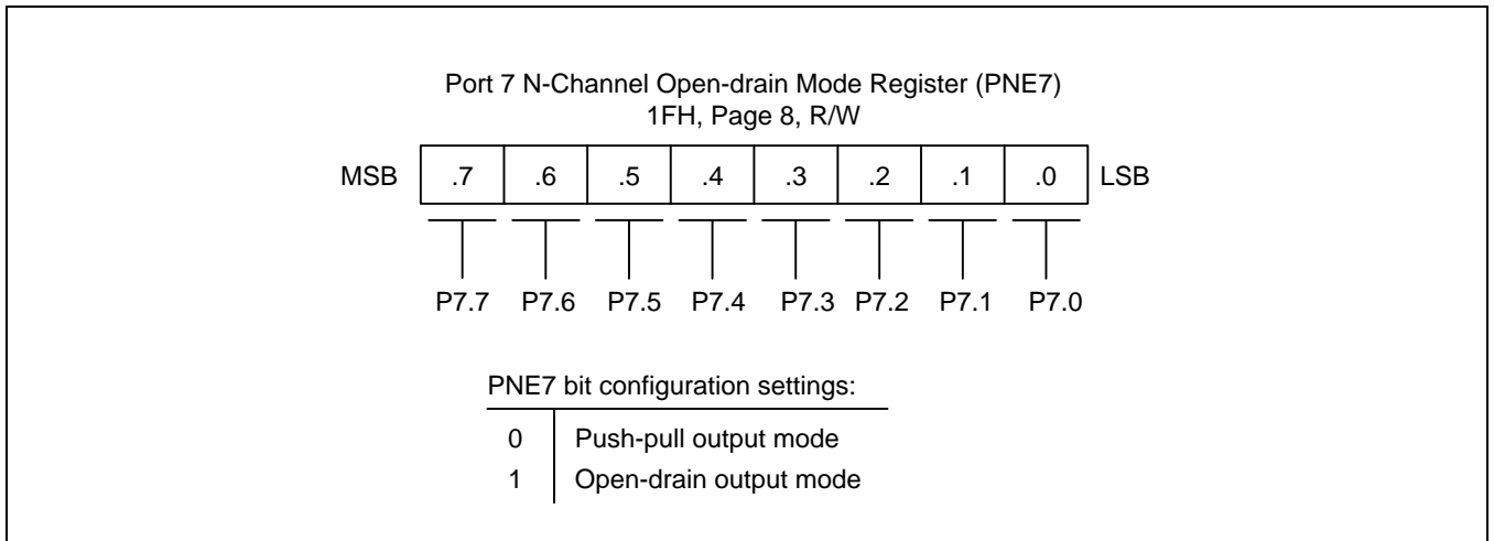
Figure 9-32 Port 7 N-Channel Open-drain Mode Register (PNE7)
