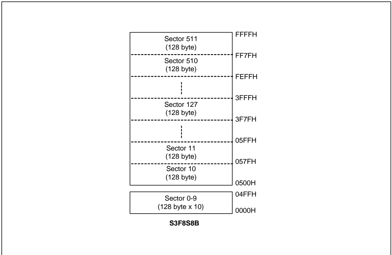
Figure 25-6 Sector Configurations in User Program Mode
