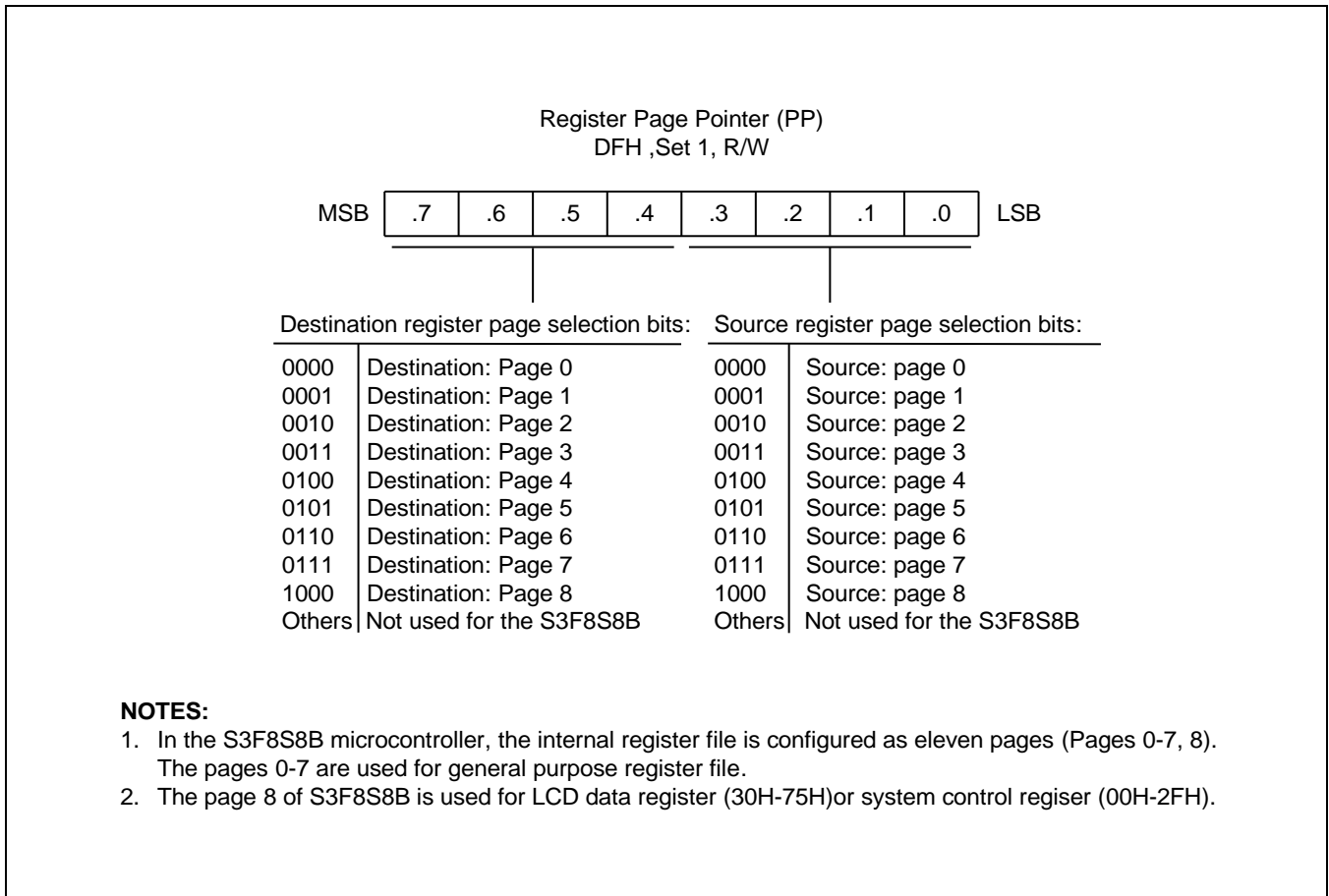
Figure 2-4 Register Page Pointer (PP)
