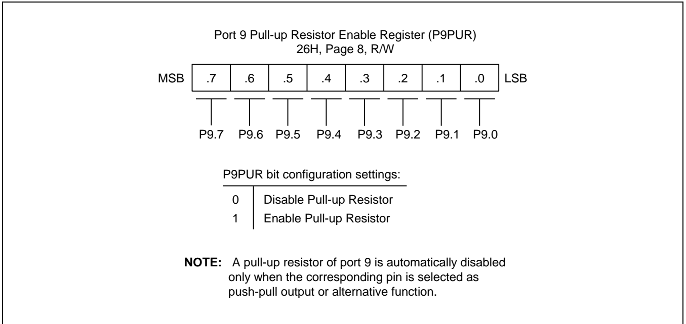
Figure 9-39 Port 9 Pull-up Resistor Enable Register (P9PUR)
