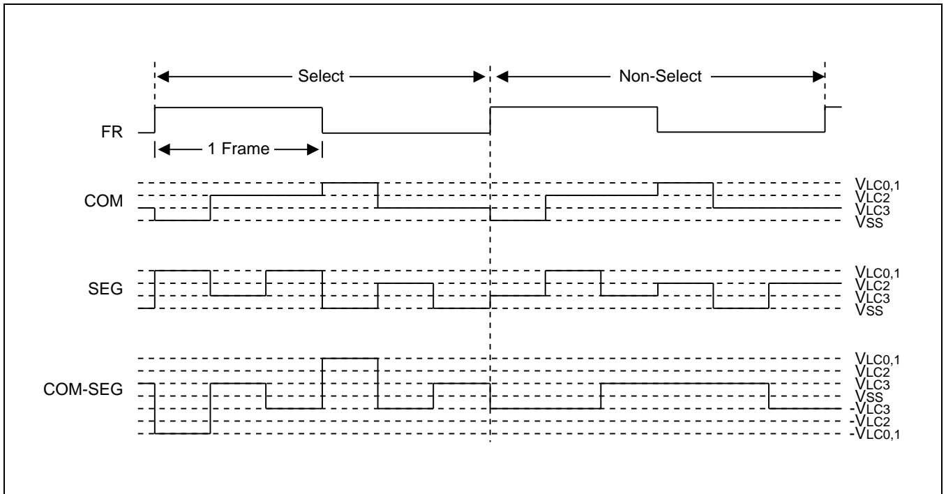
Figure 15-10 Select/No-Select Signal in 1/3 Duty, 1/3 Bias Display Mode
