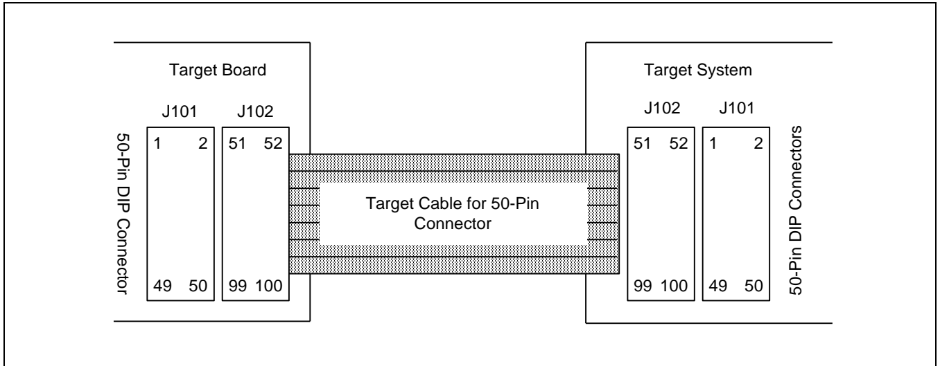
Figure 29-4 S3E8S60 Cables for 100-QFP Package
